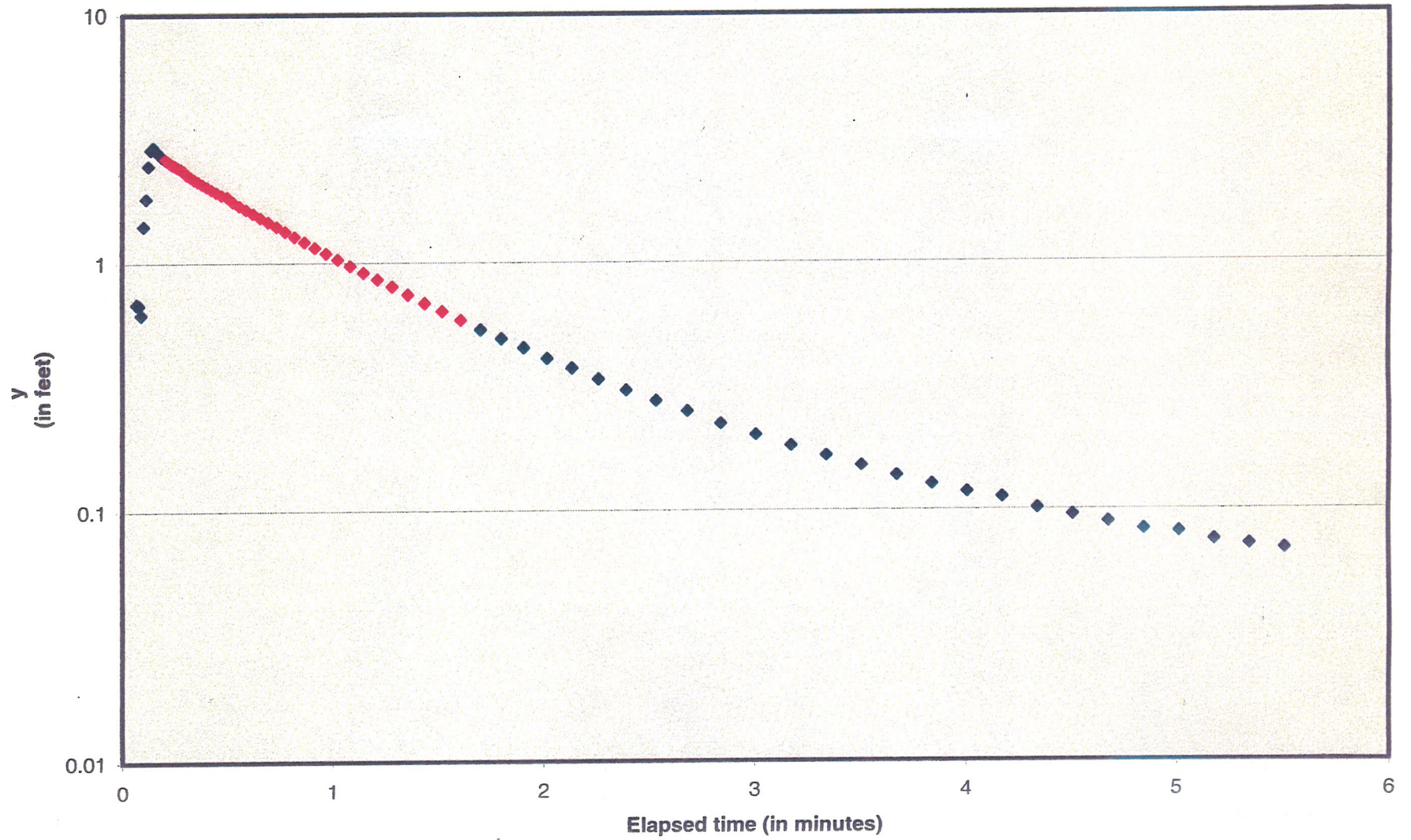
OW-946 (slug-out2) Recovery vs. Time
