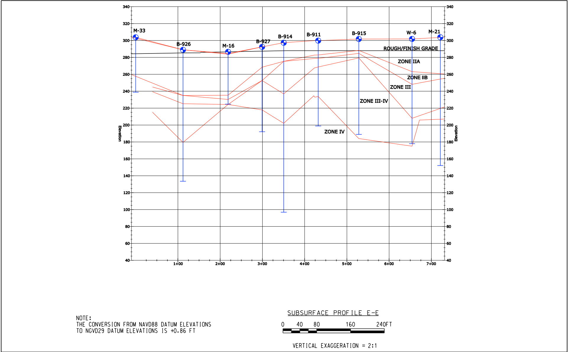
NAPS COL 2.0-29-A Figure 2.5.4-211 Subsurface Profile E-E
