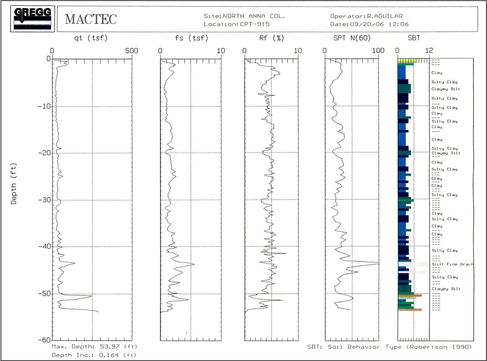
NAPS COL 2.0-30-A Figure 2.5.5-220 Log of CPT C-915
