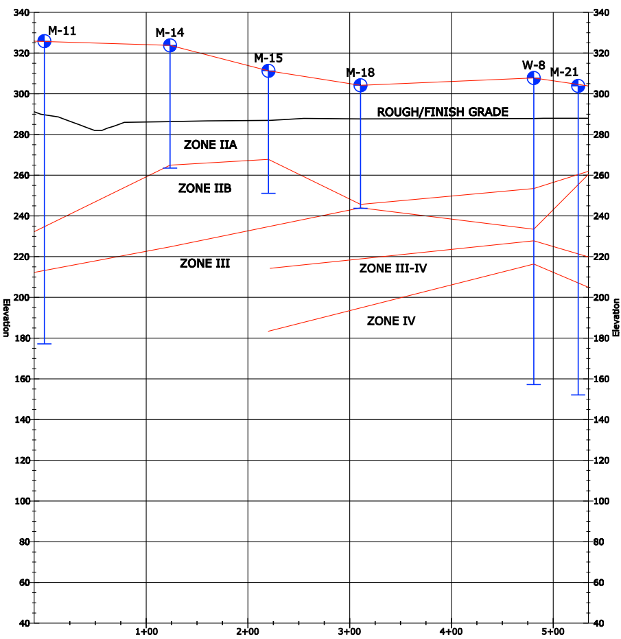
NAPS COL 2.0-29-A Figure 2.5.4-214 Subsurface Profile H-H
