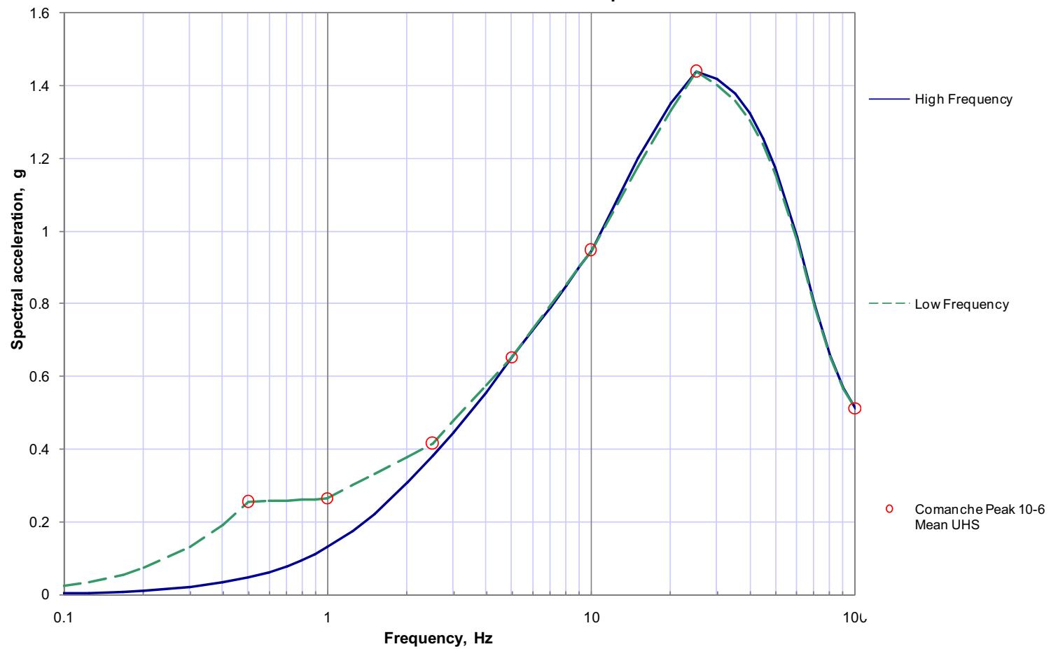
Figure 2.5.2-233 Smooth 10^{-6} Rock UHS for High and Low Frequencies
