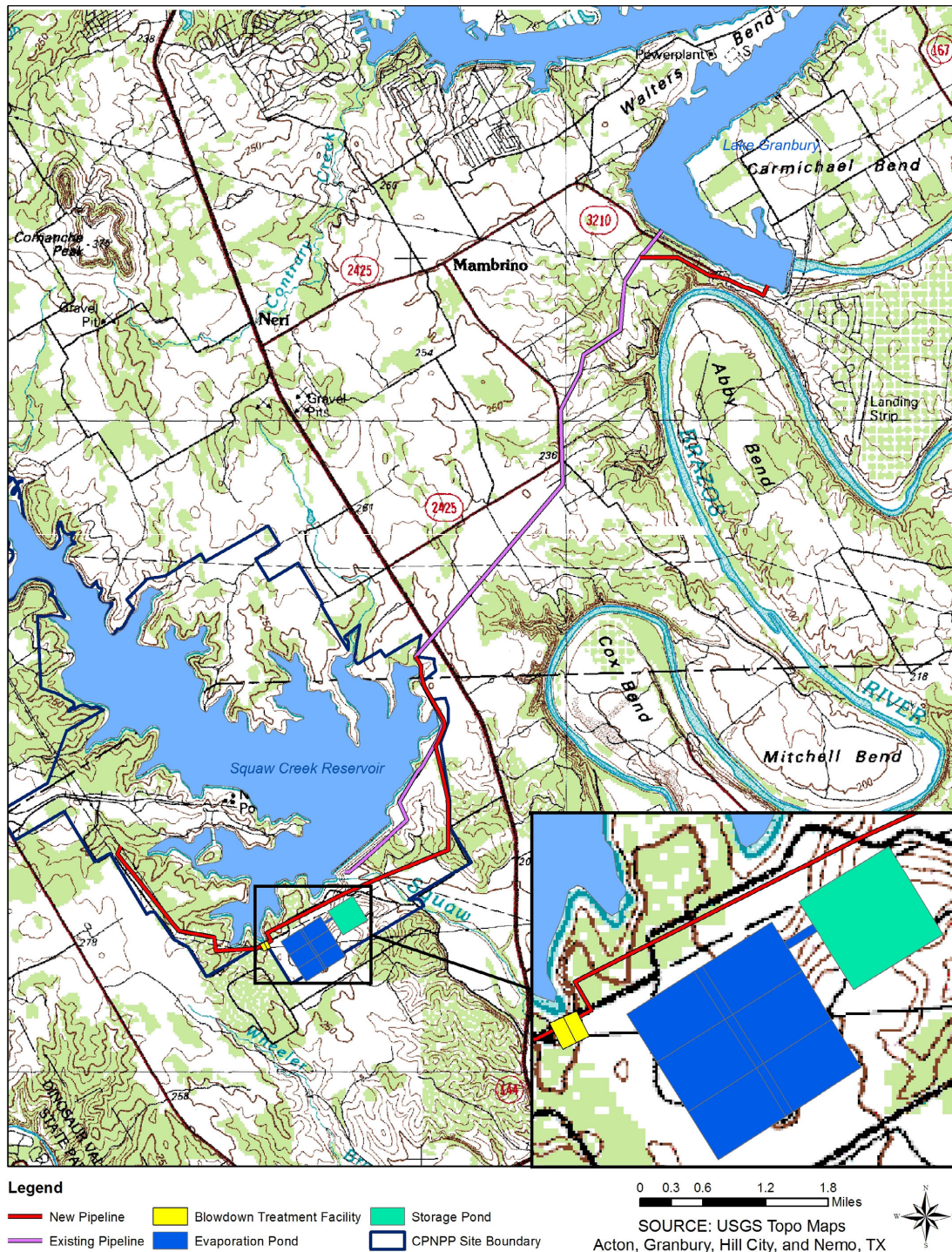
Figure 1.1-4 Off-site Cooling Water Pipelines
