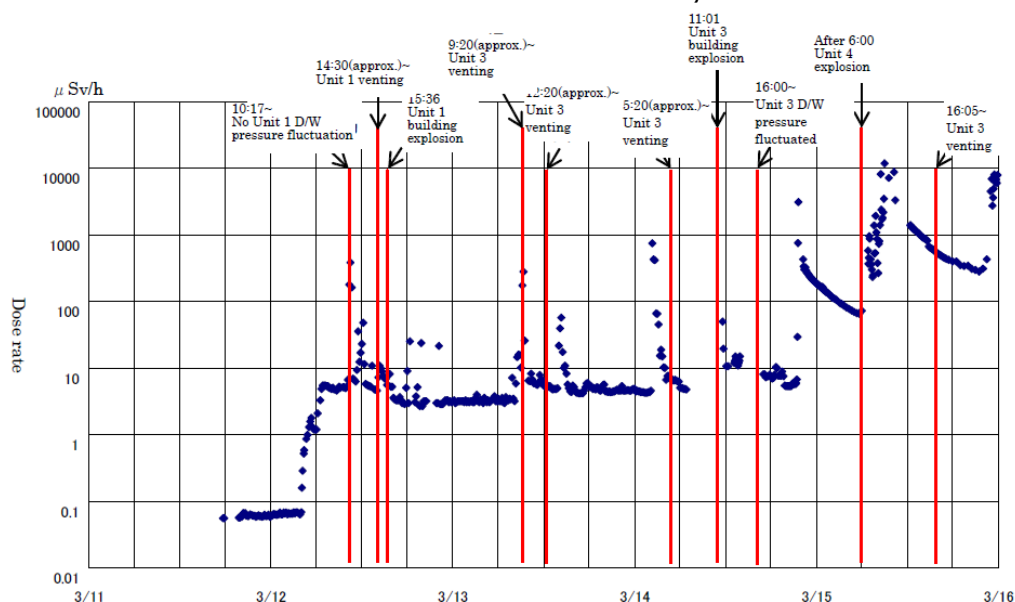
Figure 142: Dose Rate in Vicinity of Fukushima Daiichi Nuclear Plant Site Main Gate between March 11 and March 16, 2011
