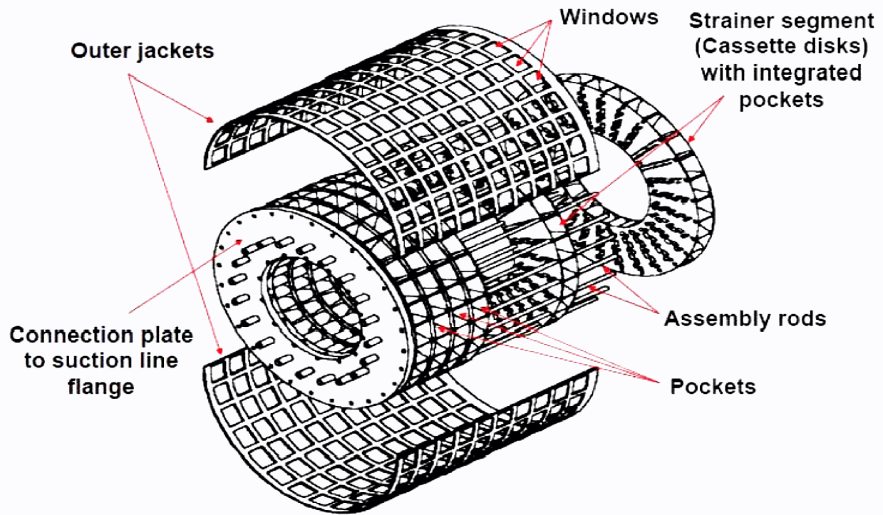
Figure 6C-1 Cassette Strainer Cutaway
