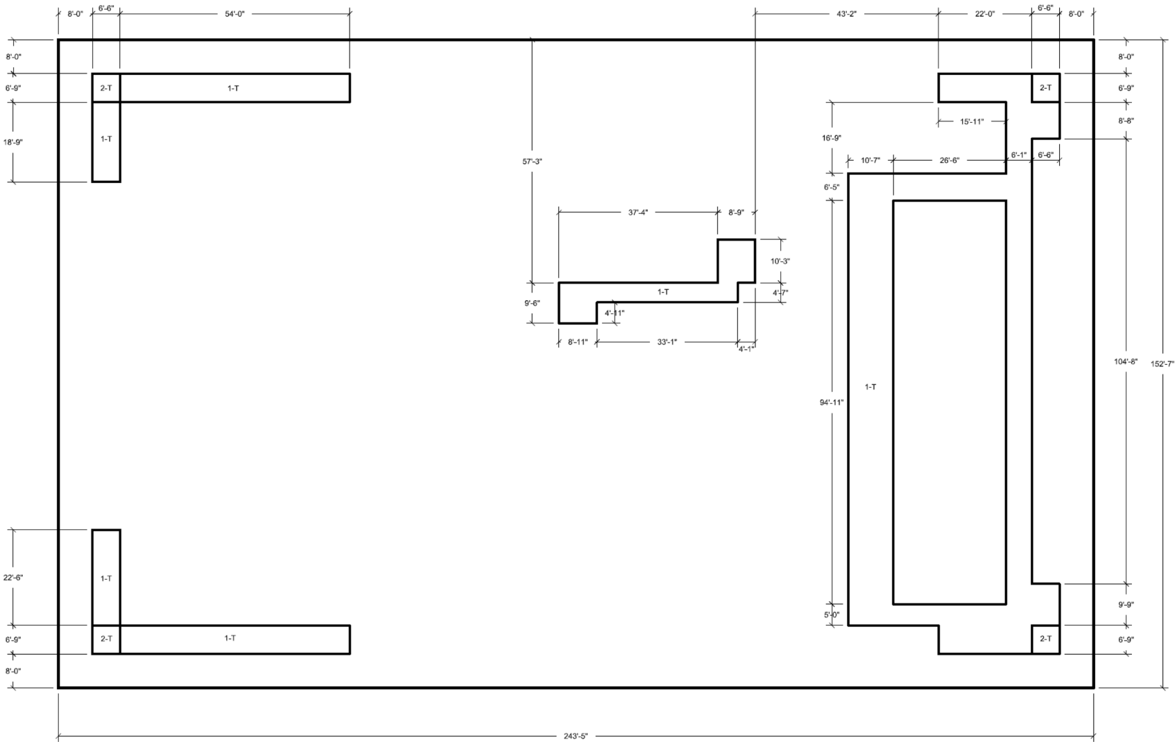
Figure 3H.3-32 RWB Basemat Looking Down Transverse Reinforcement Zones
