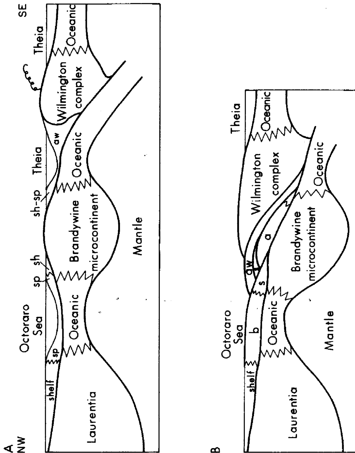
Figure 2.5-207 — {Brandywine Microcontinent}
