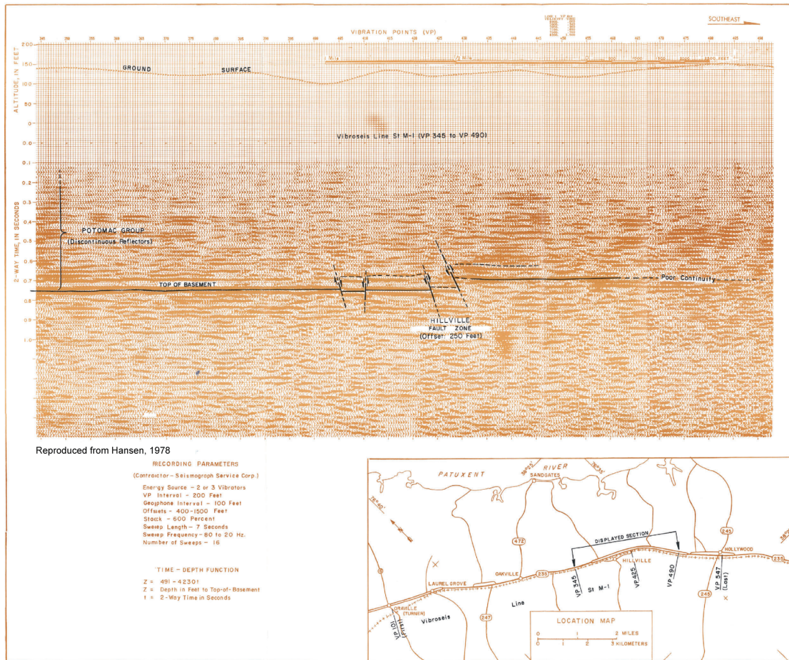
Figure 2.5-218— {Seismic Reflection Line St. M-1 Showing Hillville Fault of Hansen (1978)}
