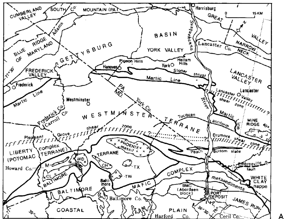
Figure 2.5-201— {Appalachian Orogen}
