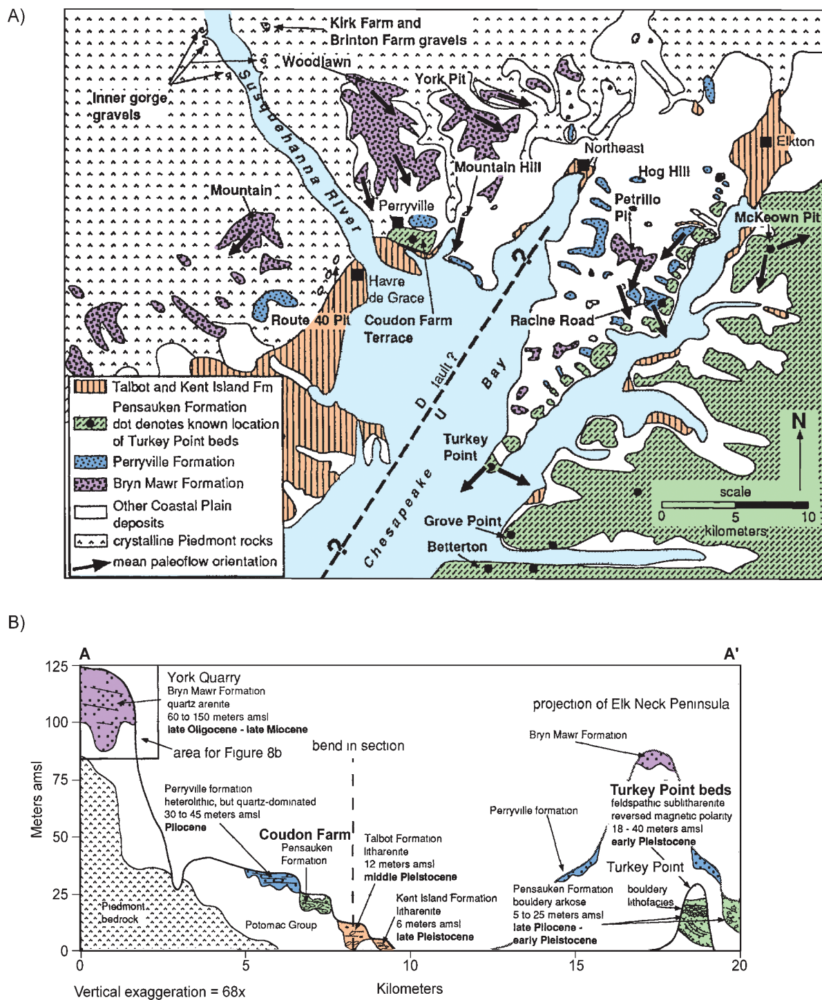
Figure 2.5-216— {(A) Generalized Geological Map and (B) Schematic Cross Section of the Northern Chesapeake Bay}
