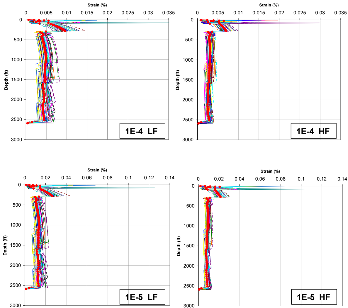
Figure 2.5-223— {Calculated Maximum Strains Based on Initially Adopted EPRI Curves}
