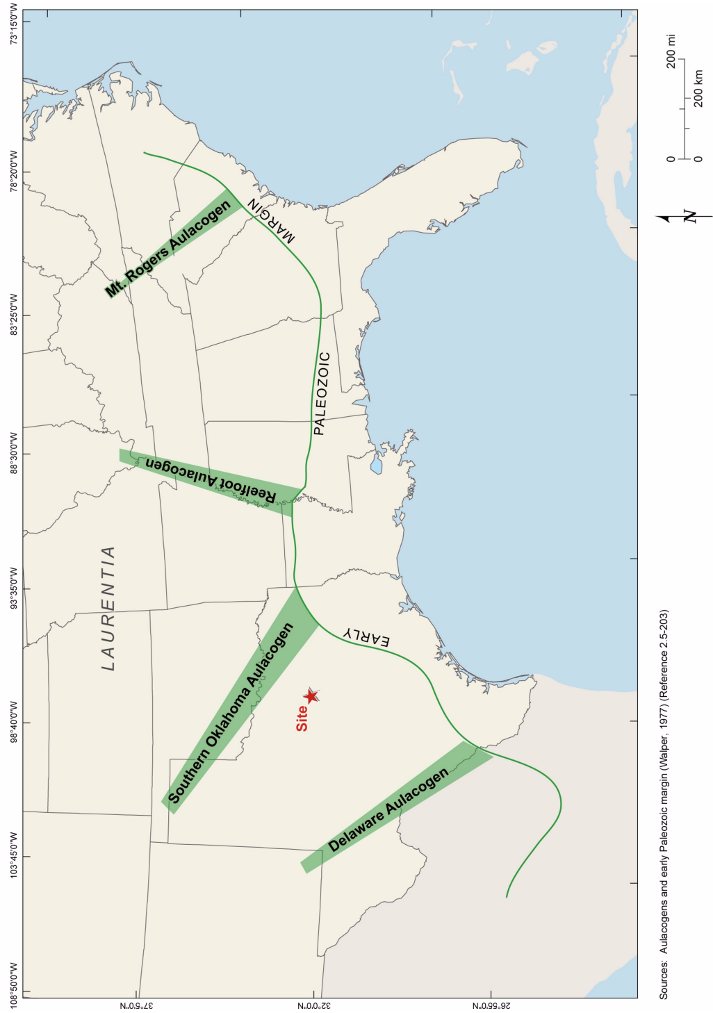
Figure 2.5.1-208 North American Aulacogens
