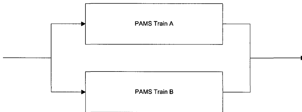
Figure 4.1-1. Top Level PAMS RBD
