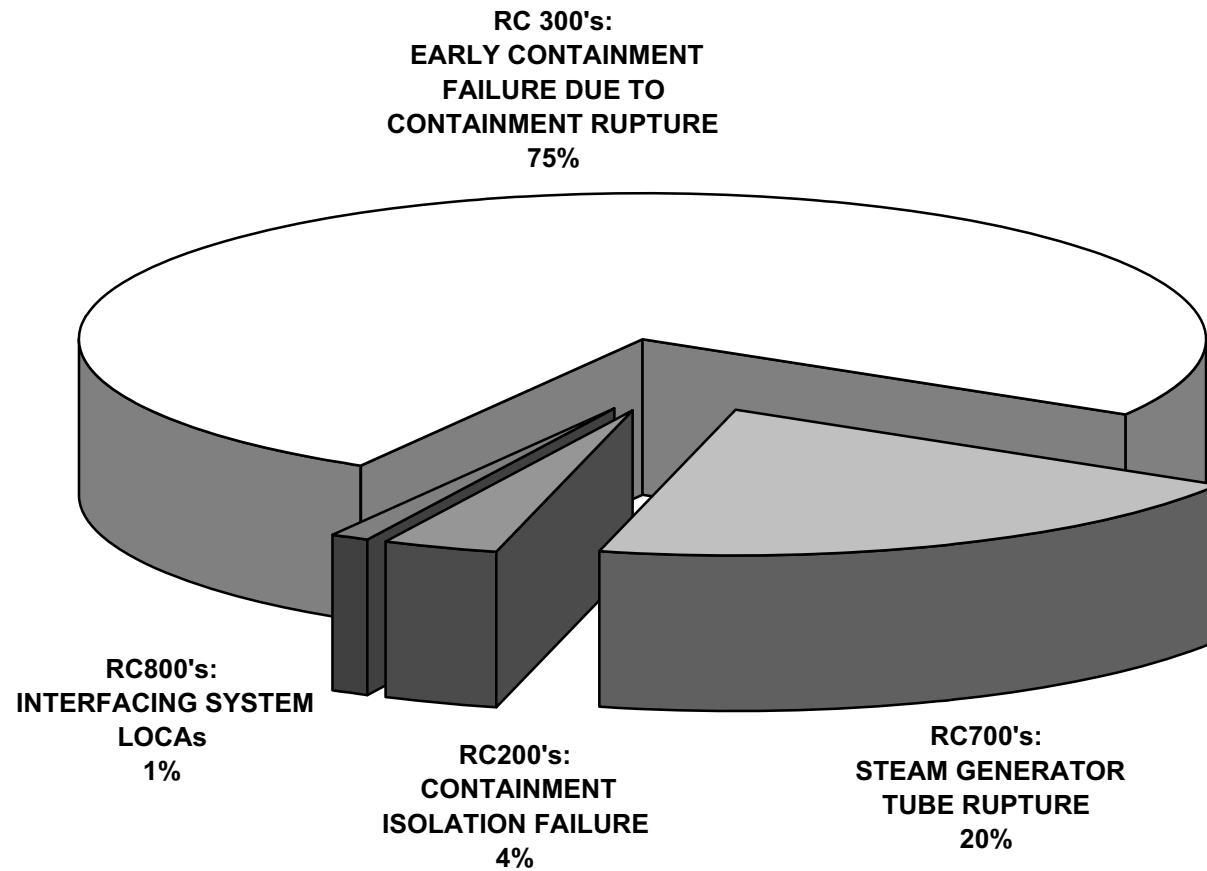
Figure 19.1-27—U.S. EPR Level 2 Release Category Contribution to Total At-Power LRF
