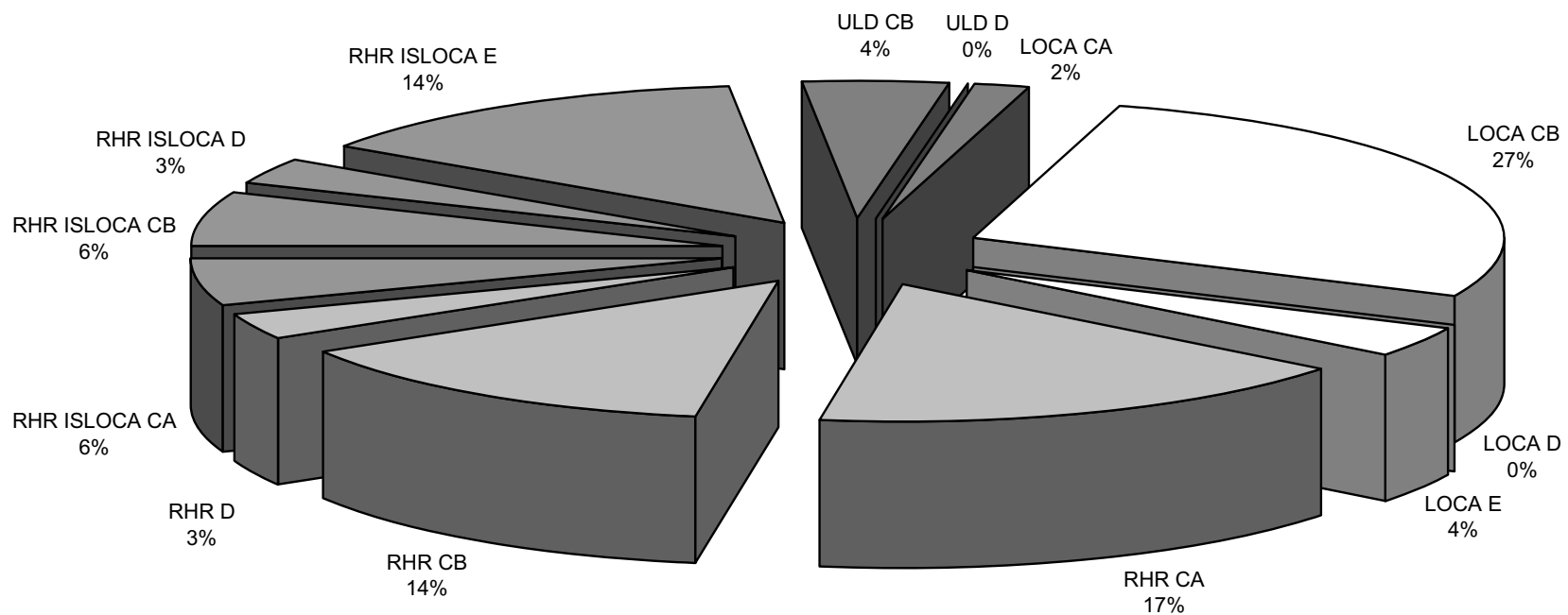
Figure 19.1-37—Initiating Events Contributions to Shutdown LRF
