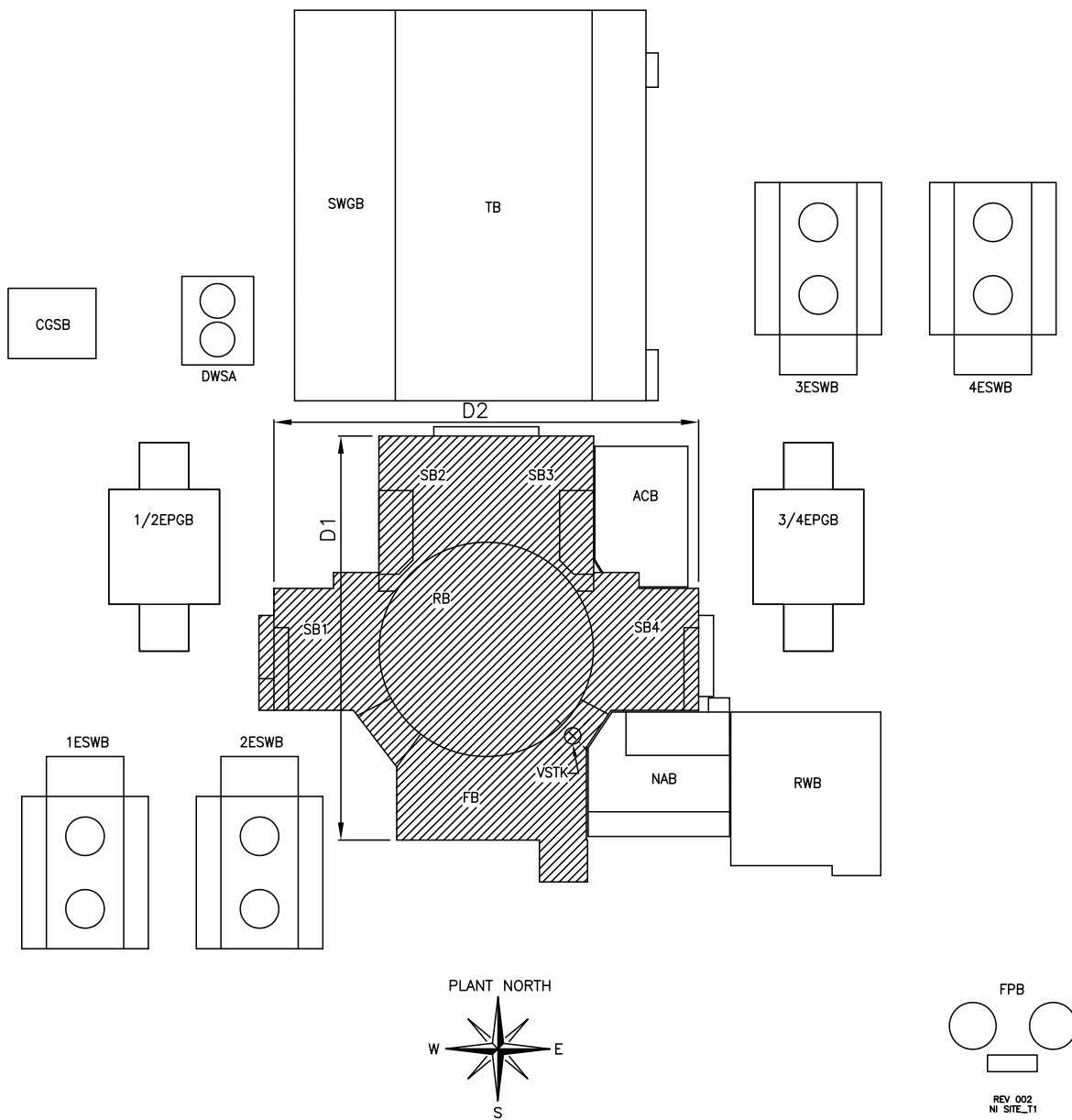
Figure 2.1.1-1—U.S. EPR Building Layout Showing NI Structures Location
