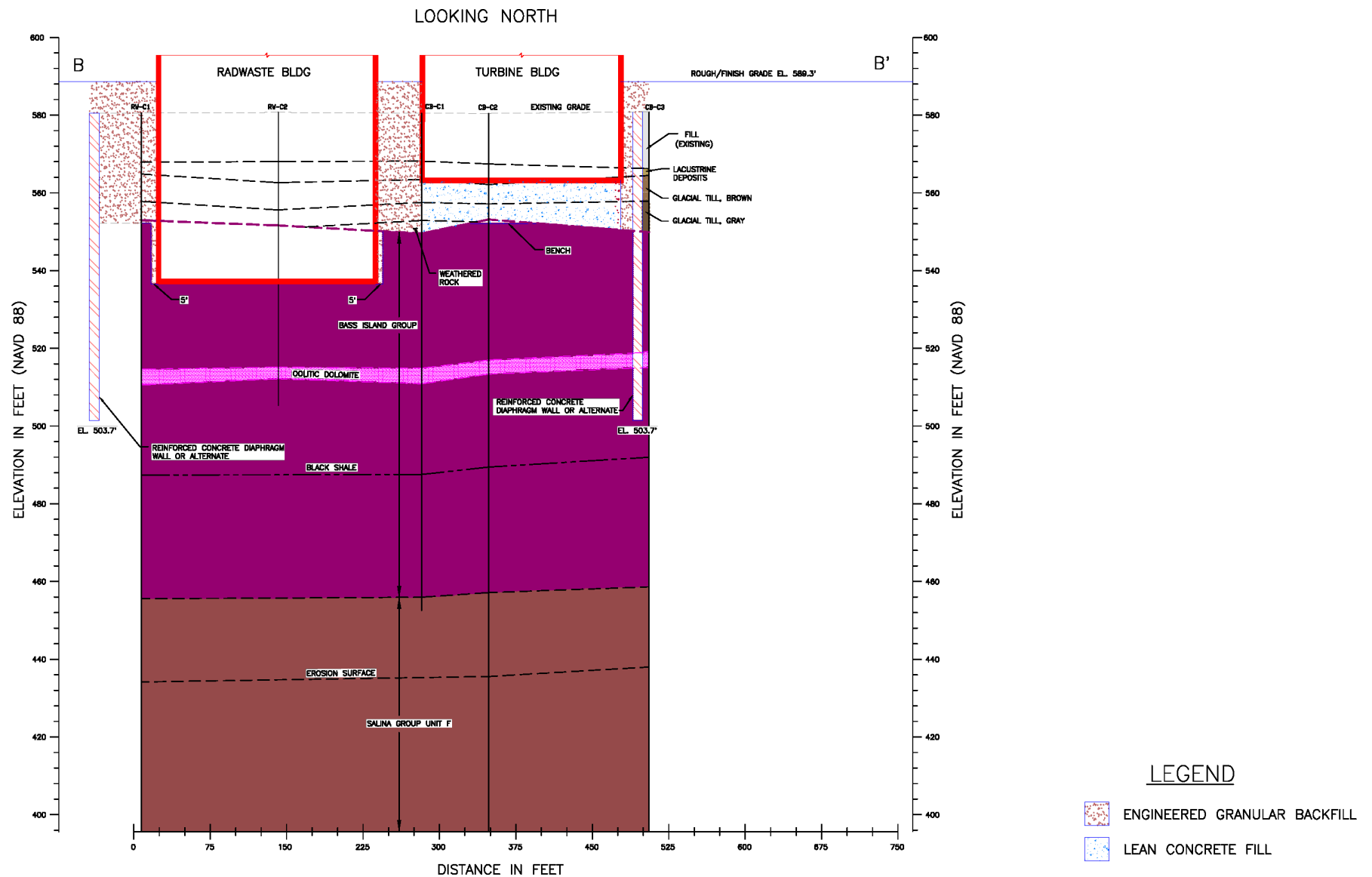
Figure 2.5.4-204 Excavation Cross Section B-B'
