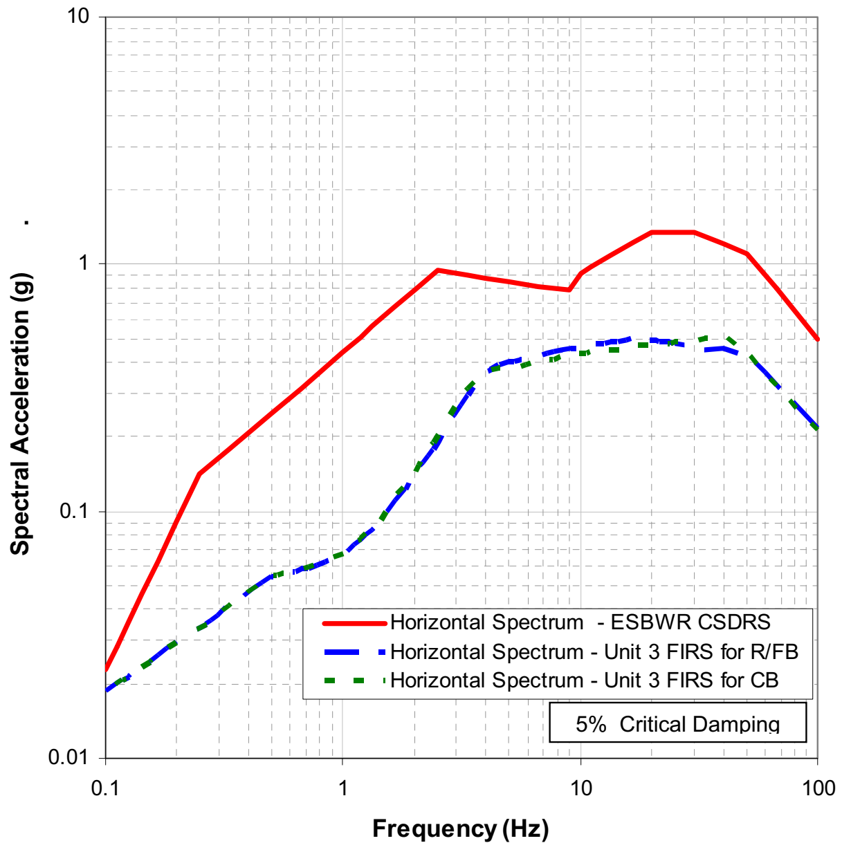
Figure 2.0-201 Comparison of Horizontal CSDRS with the Unit 3 FIRS for the RB/FB and CB [EF3 COL 2.0-1-A]
