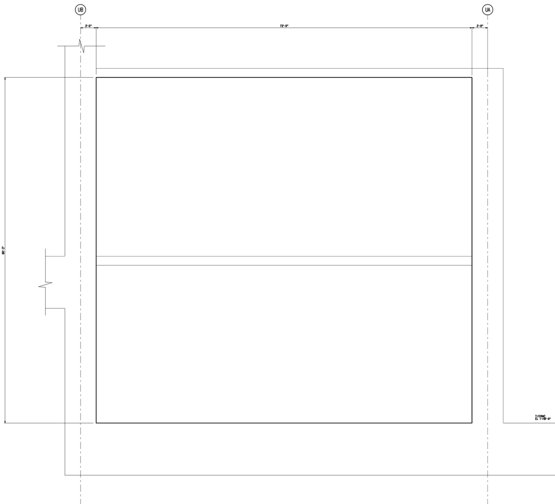
Figure 3H.6-73 Pumphouse Internal East Wall Looking West Vertical Reinforcement Zones Near Side Face
