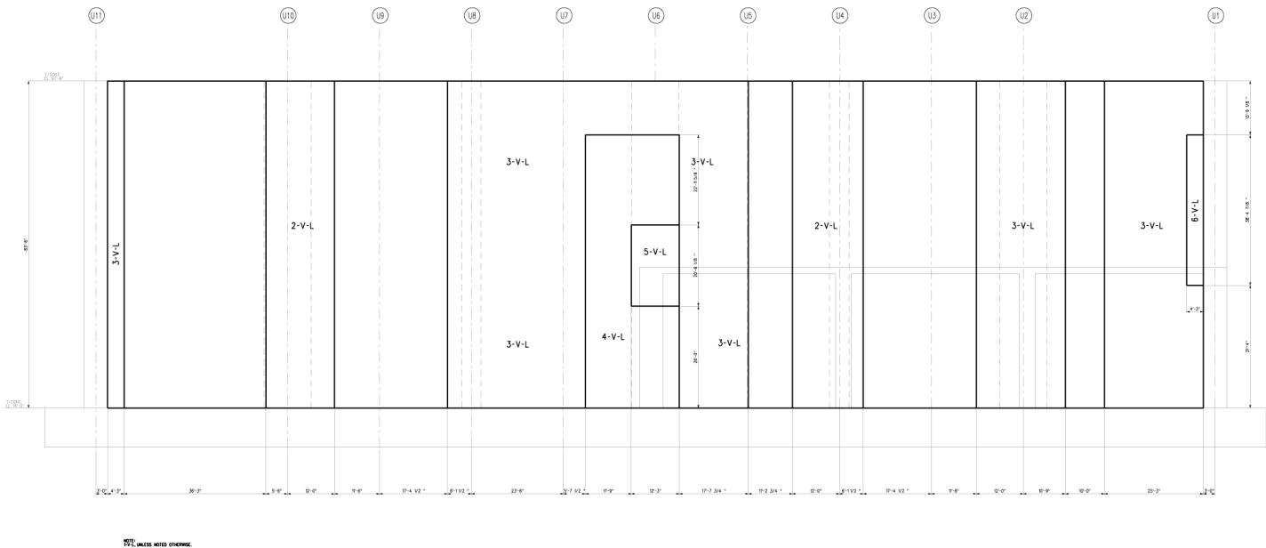
Figure 3H.6-83 Basin North Wall Looking South Vertical Reinforcement Zones Near Side Face
