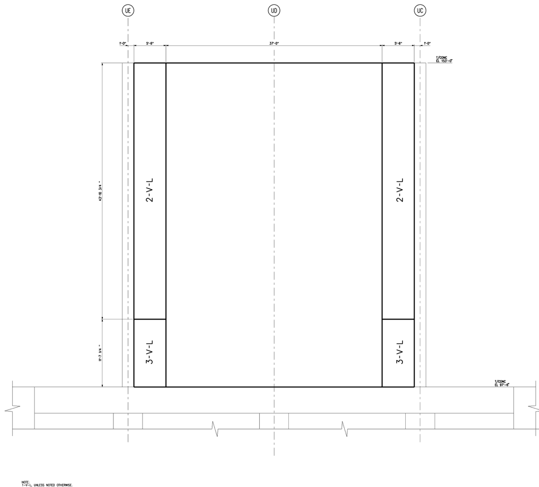
Figure 3H.6-122 Fan Internal Wall Looking West Vertical Reinforcement Zones Near and Far Side Faces
