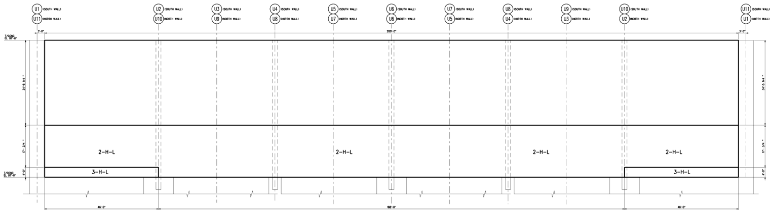
Figure 3H.6-108 Fan North (and South) Wall Looking South (North) Horizontal Reinforcement Zones Near Side Face
