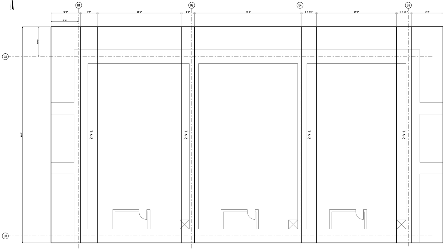
Figure 3H.6-126 Pumphouse Mat North/South Reinforcement Zones Bottom Face
