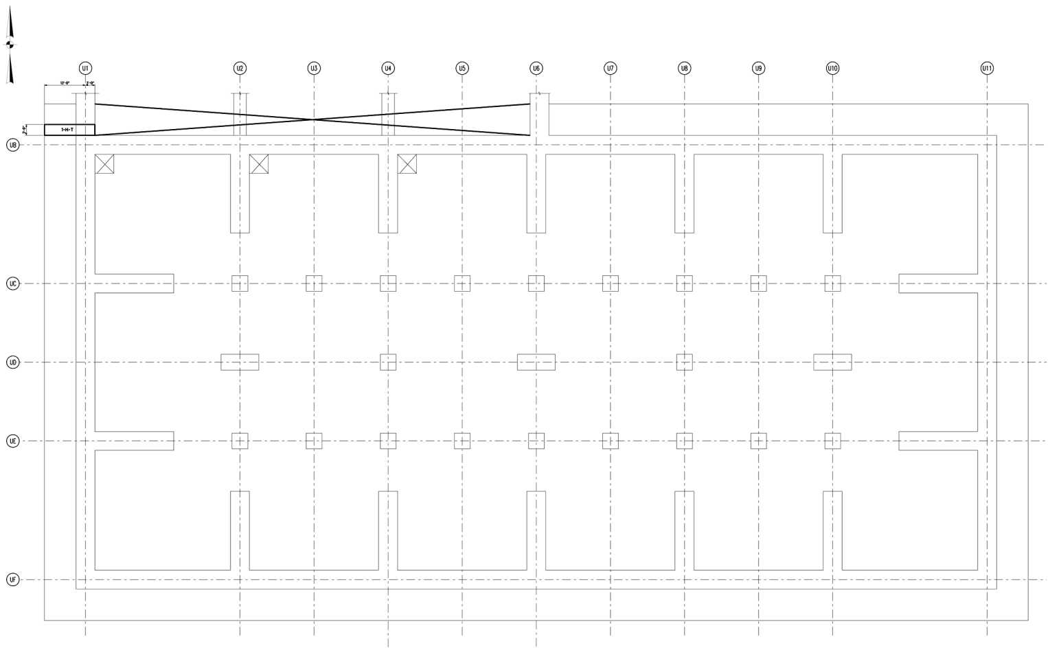
Figure 3H.6-133 Ultimate Heat Sink Basin Base Mat Plan Transverse Horizontal Reinforcement Zones
