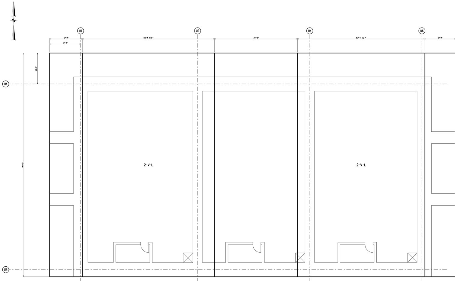
Figure 3H.6-124 Pumphouse Mat North/South Reinforcement Zones Top Face
