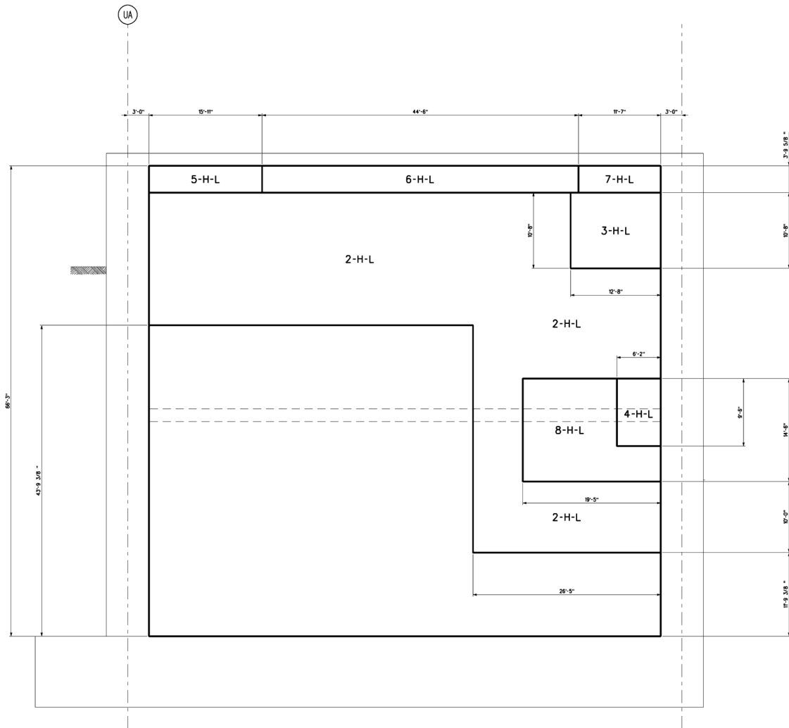
Figure 3H.6-67 Pumphouse West Wall Looking East Horizontal Reinforcement Zones Near Side Face
