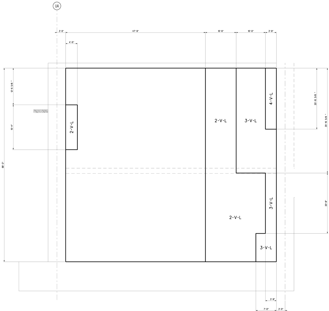
Figure 3H.6-70 Pumphouse West Wall Looking East Vertical Reinforcement Zones Far Side Face
