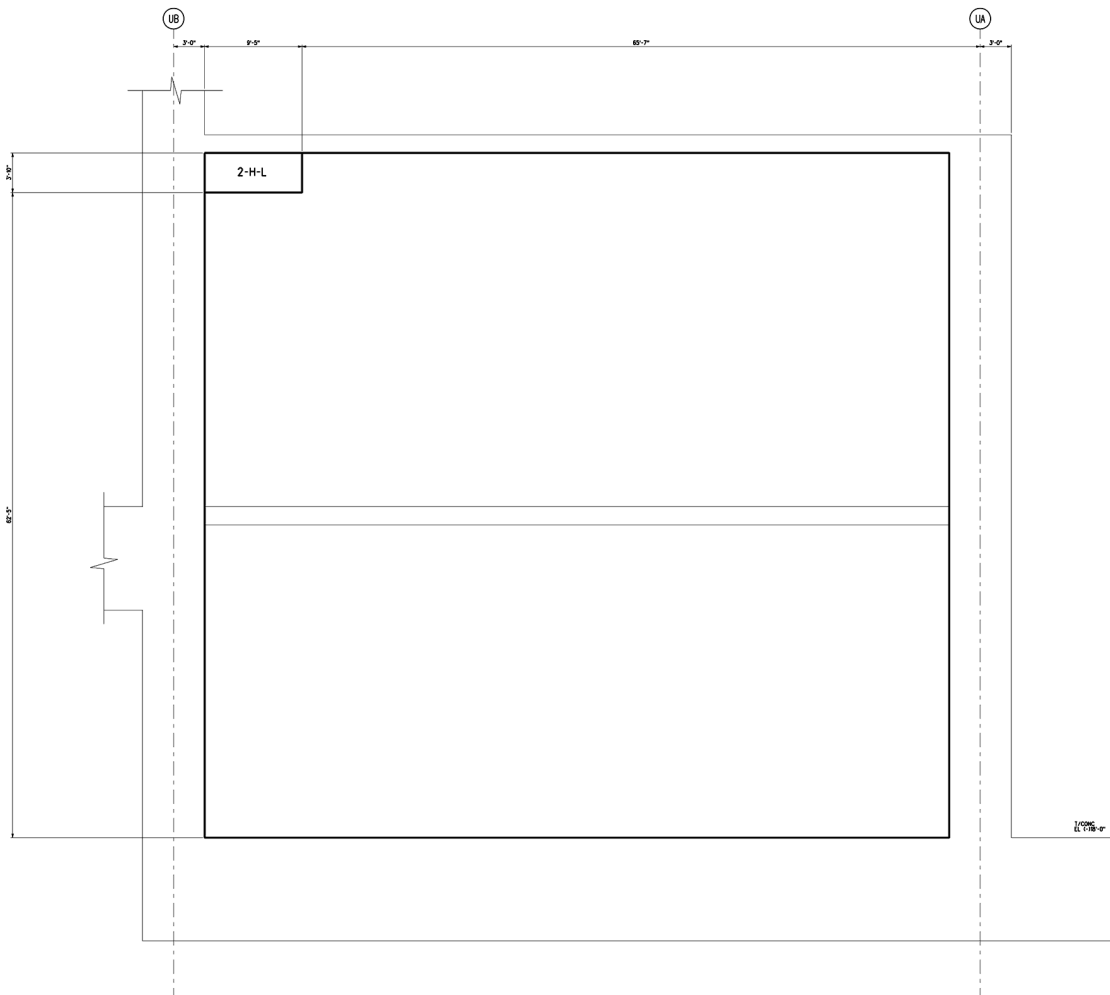
Figure 3H.6-76 Pumphouse Internal West Wall Looking West Horizontal Reinforcement Zones Near Side Face
