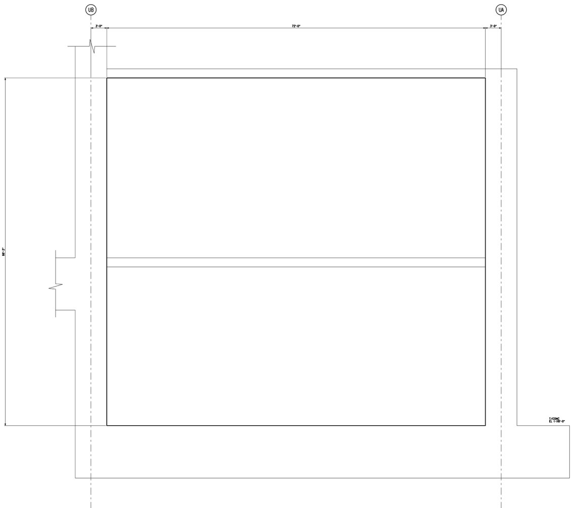
Figure 3H.6-75 Pumphouse Internal East Wall Looking West Vertical Reinforcement Zones Far Side Face
