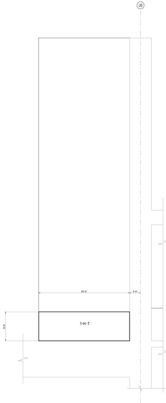
Figure 3H.6-104 Basin North Buttress Looking West & Basin South Buttress Looking East Transverse Horizontal Reinforcement Zones
