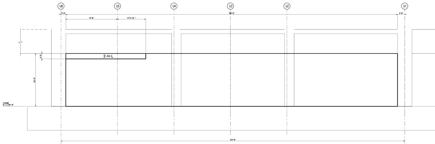
Figure 3H.6-62 Pumphouse South Wall Looking South Horizontal Reinforcement Zones Rear Side Face
