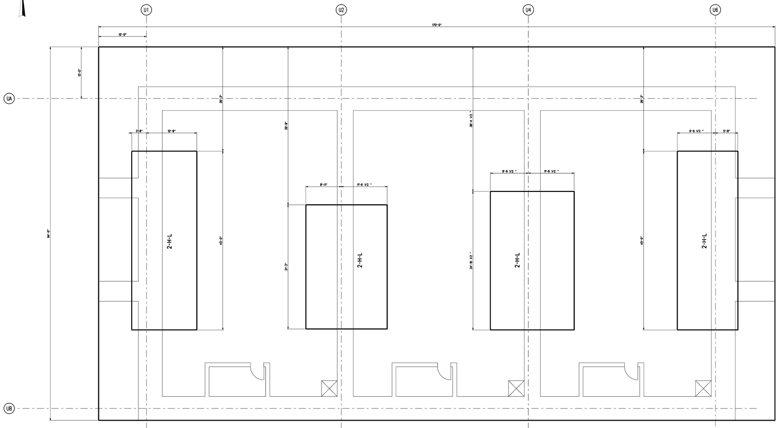
Figure 3H.6-125 Pumphouse Mat East/West Reinforcement Zones Bottom Face
