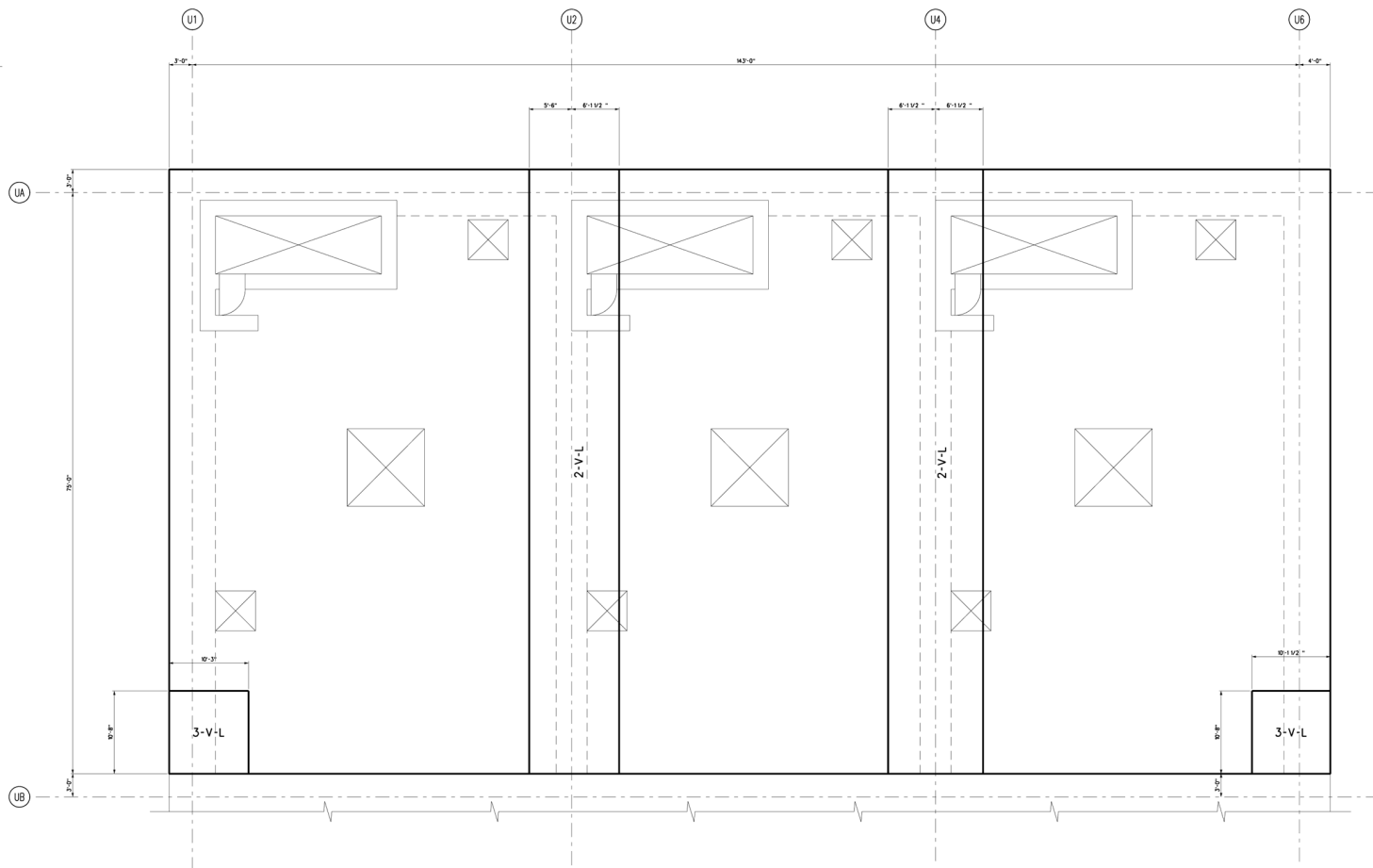
Figure 3H.6-51 Pumphouse Roof North/South Reinforcement Zones Bottom Face
