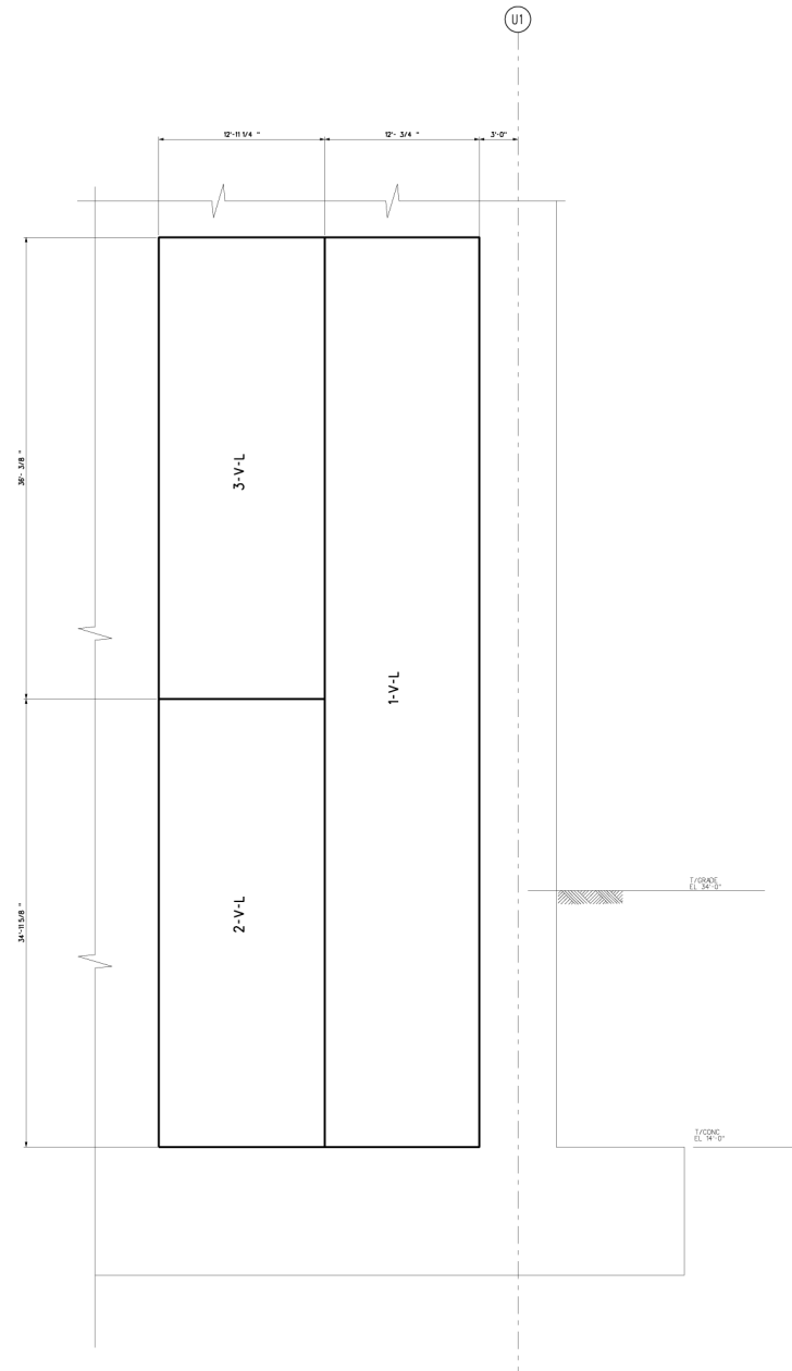
Figure 3H.6-106 Basin East Buttress Looking North & Basin West Buttress Looking South Vertical Reinforcement Zones Near & Far Side Faces
