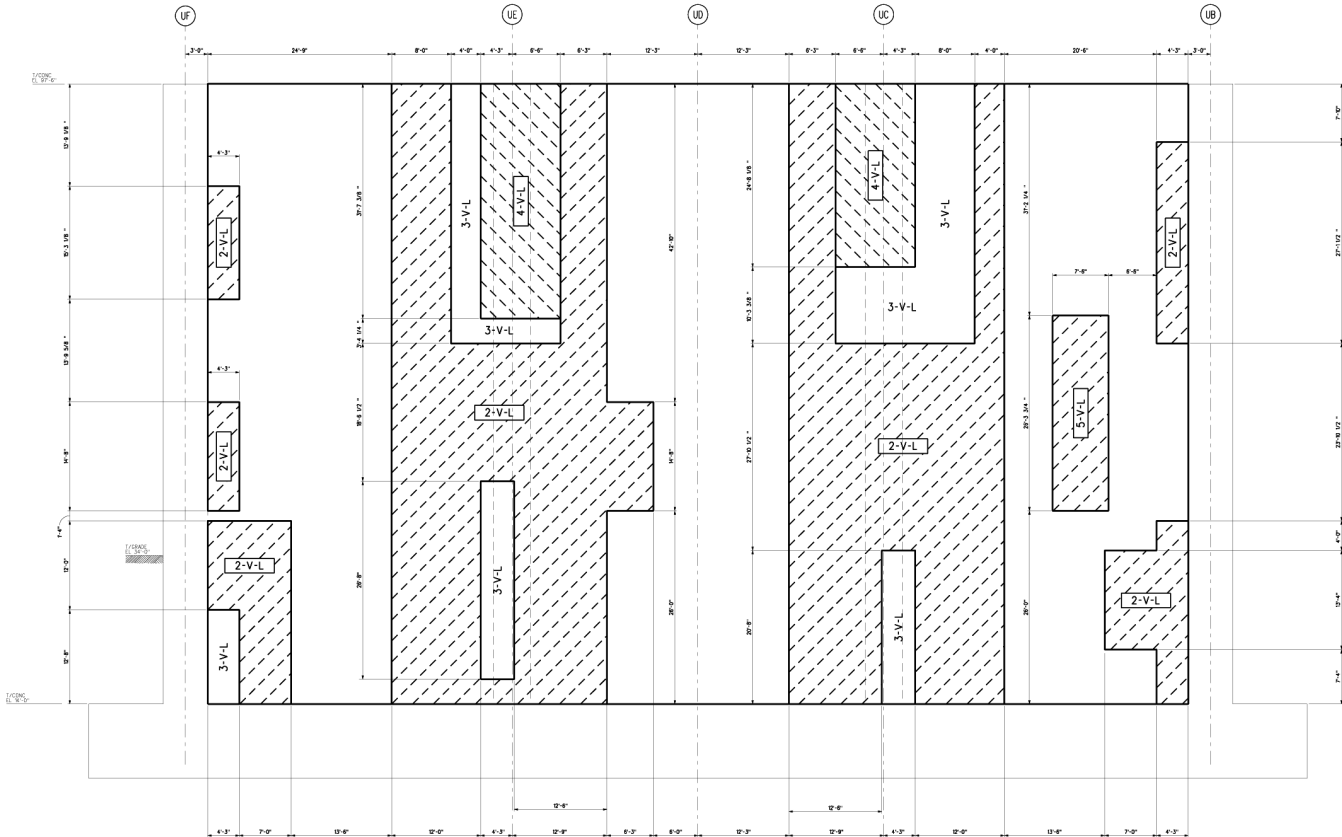
Figure 3H.6-93 Basin East Wall Looking West Vertical Reinforcement Zones Near Side Face
