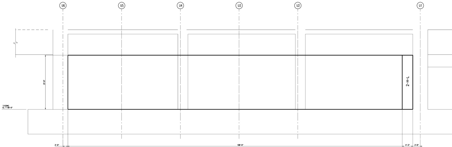
Figure 3H.6-64 Pumphouse South Wall Looking South Horizontal Reinforcement Zones Far Side Face
