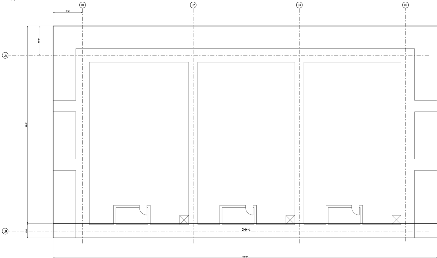
Figure 3H.6-123 Pumphouse Mat East/West Reinforcement Zones Top Face
