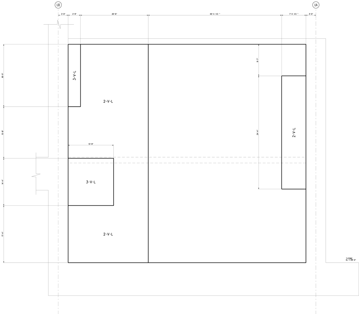
Figure 3H.6-58 Pumphouse East Wall Looking West Vertical Reinforcement Zones Near Side Face
