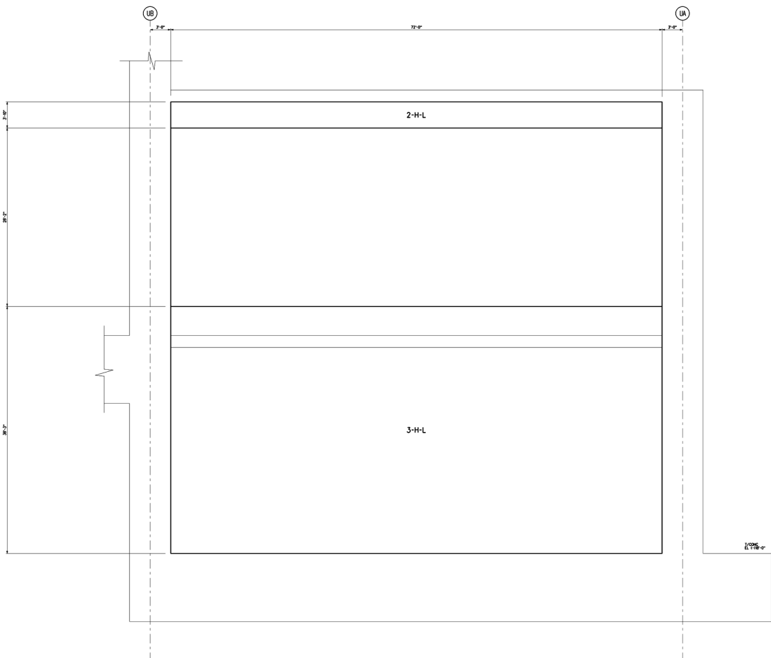
Figure 3H.6-74 Pumphouse Internal East Wall Looking West Horizontal Reinforcement Zones Far Side Face
