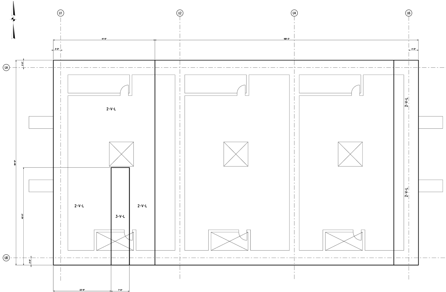
Figure 3H.6-128 Pumhouse Floor EI 14'-0" North/South Reinforcement Zones Top and Bottom Faces
