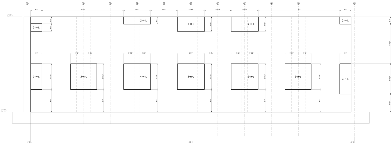
Figure 3H.6-89 Basin South Wall Looking North Horizontal Reinforcement Zones Far Side Face
