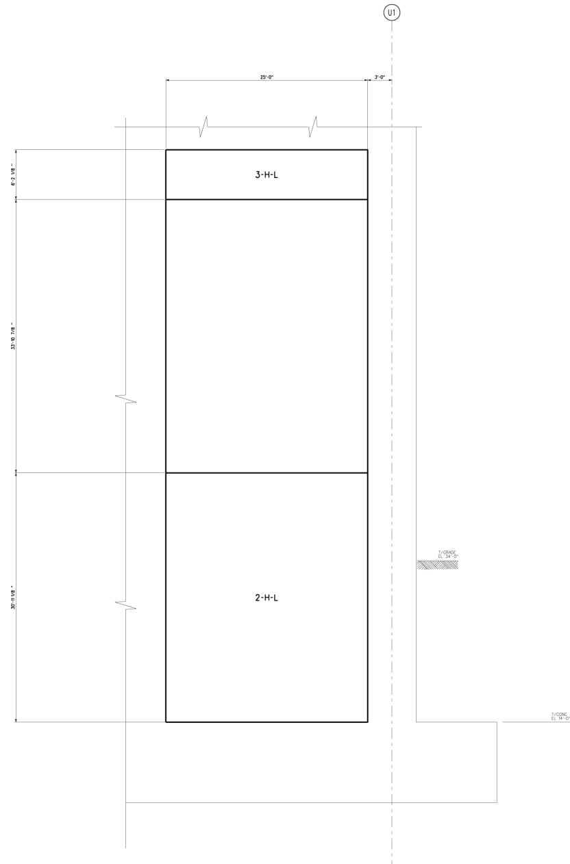
Figure 3H.6-105 Basin East Buttress Looking North & Basin West Buttress Looking South Horizontal Reinforcement Zones Near and Far Side Faces
