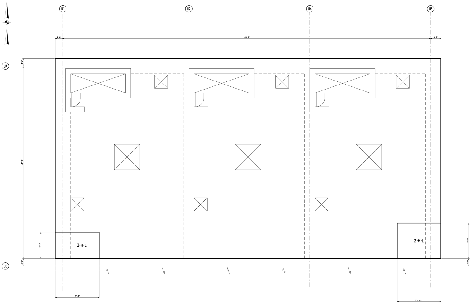
Figure 3H.6-136 Pumphouse Roof East/West Reinforcement Zones Bottom Face
