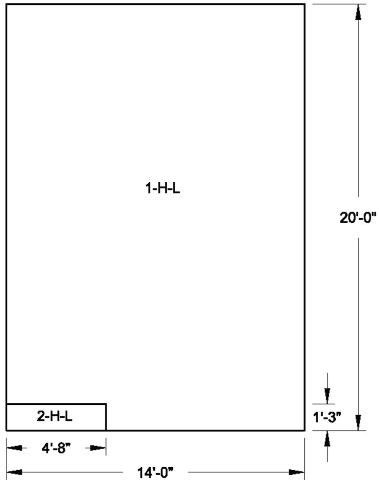
Figure 3H.6-173 Wall 9 Looking From Outside Horizontal Reinforcement Zones Near Side Face
