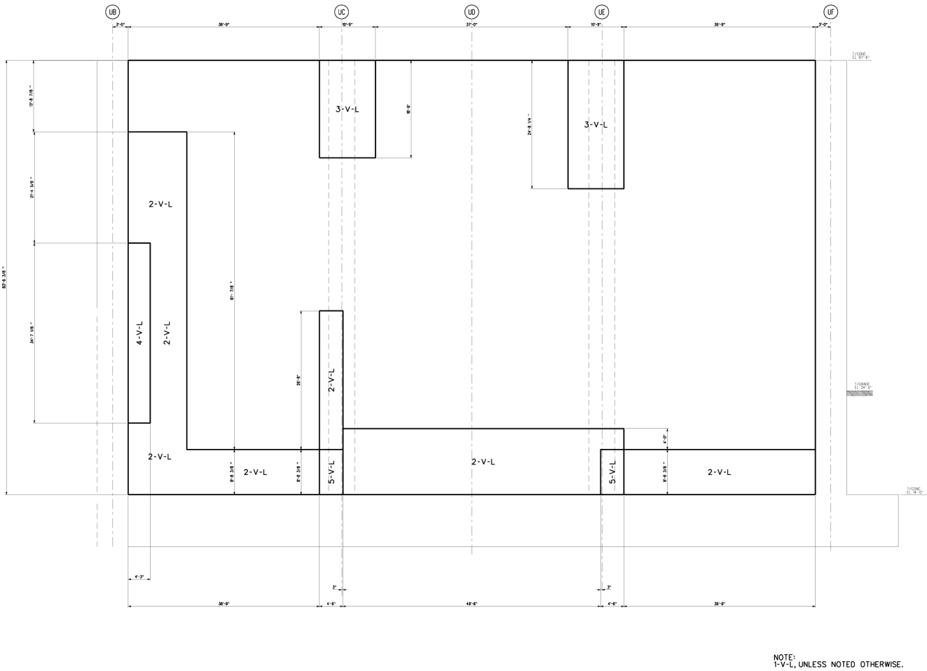
Figure 3H.6-100 Basin West Wall Looking East Vertical Reinforcement Zones Far Side Face
