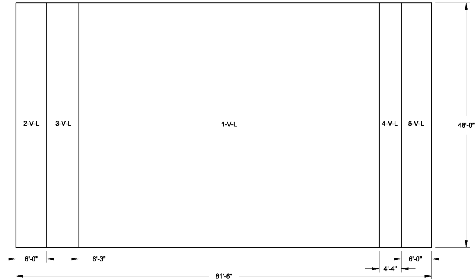
Figure 3H.6-143 Slab 1 Looking Down Vertical Reinforcement Zones Near Side Face
