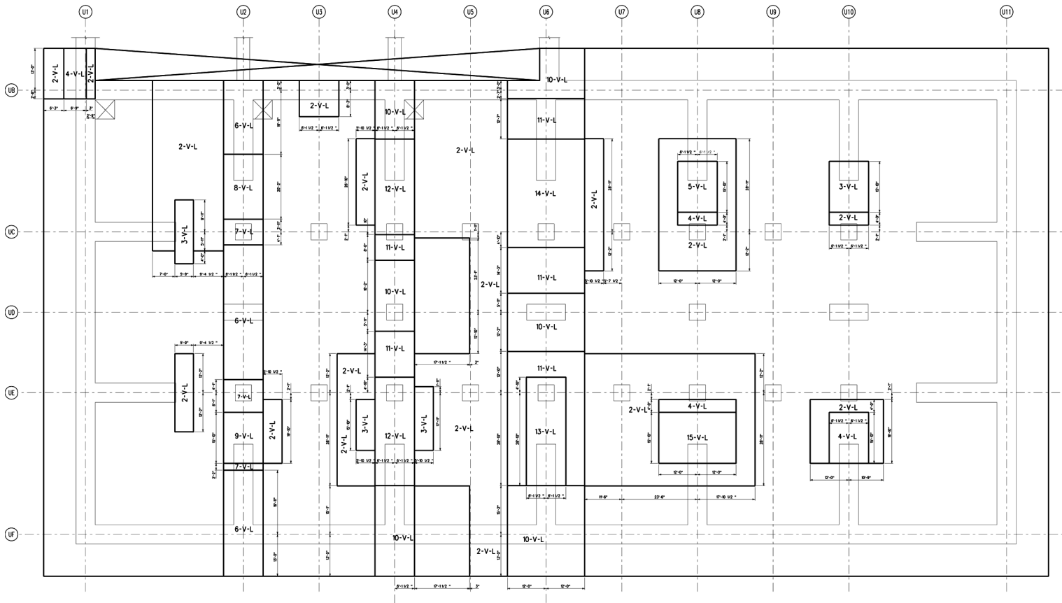
Figure 3H.6-130 Ultimate Heat Sink Basin Base Mat Plan North/South Reinforcement Zones Top Face
