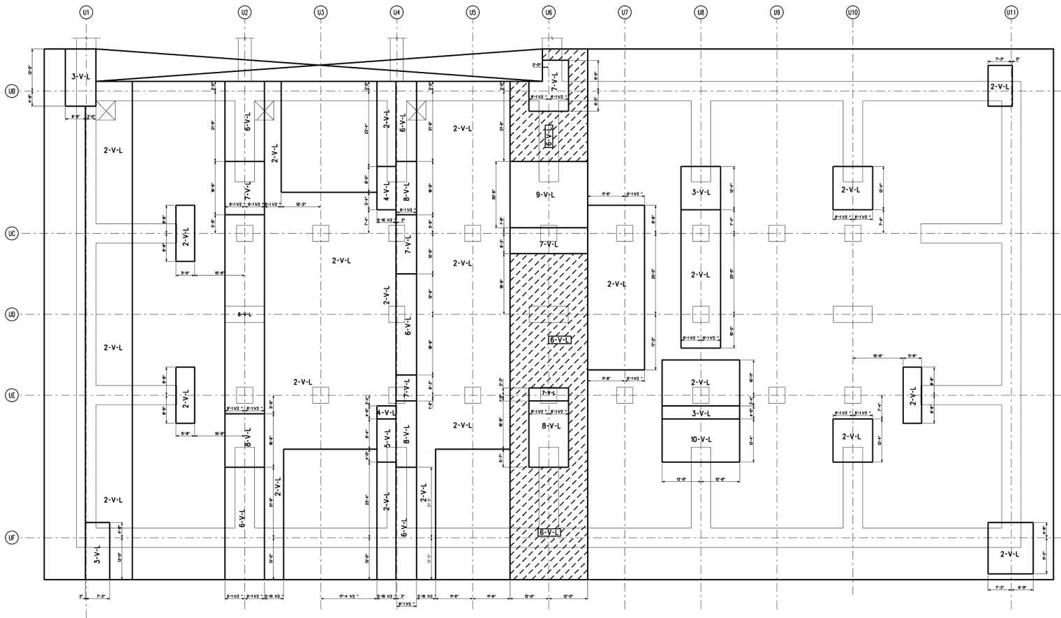
Figure 3H.6-132 Ultimate Heat Sink Basin Base Mat Plan North/South Reinforcement Zones Bottom Face
