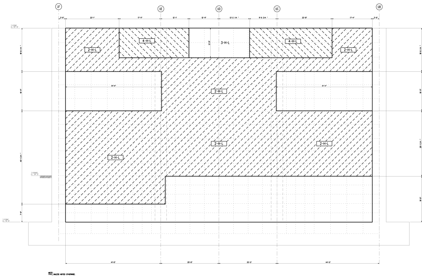
Figure 3H.6-92 Basin East Wall Looking West Horizontal Reinforcement Zones Near Side Face
