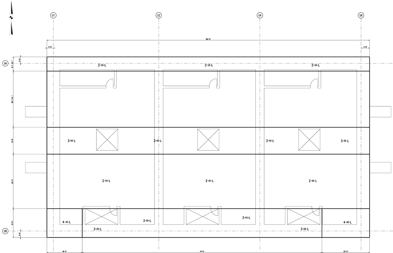
Figure 3H.6-127 Pumphouse Floor El 14'-0" East/ West Reinforcement Zones Top and Bottom Faces
