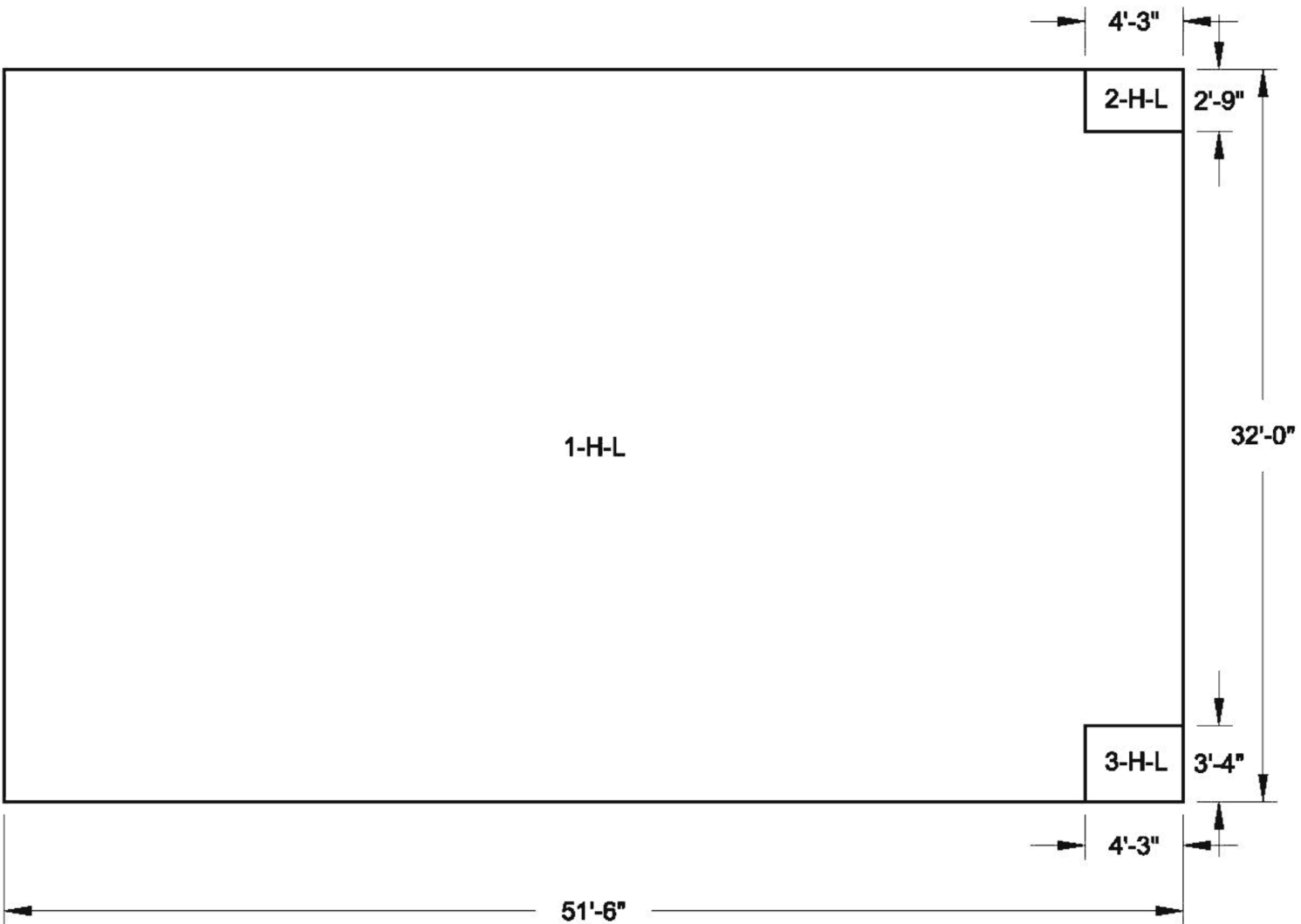
Figure 3H.6-147 Roof 2 Looking Down Horizontal Reinforcement Zones Near Side Face
