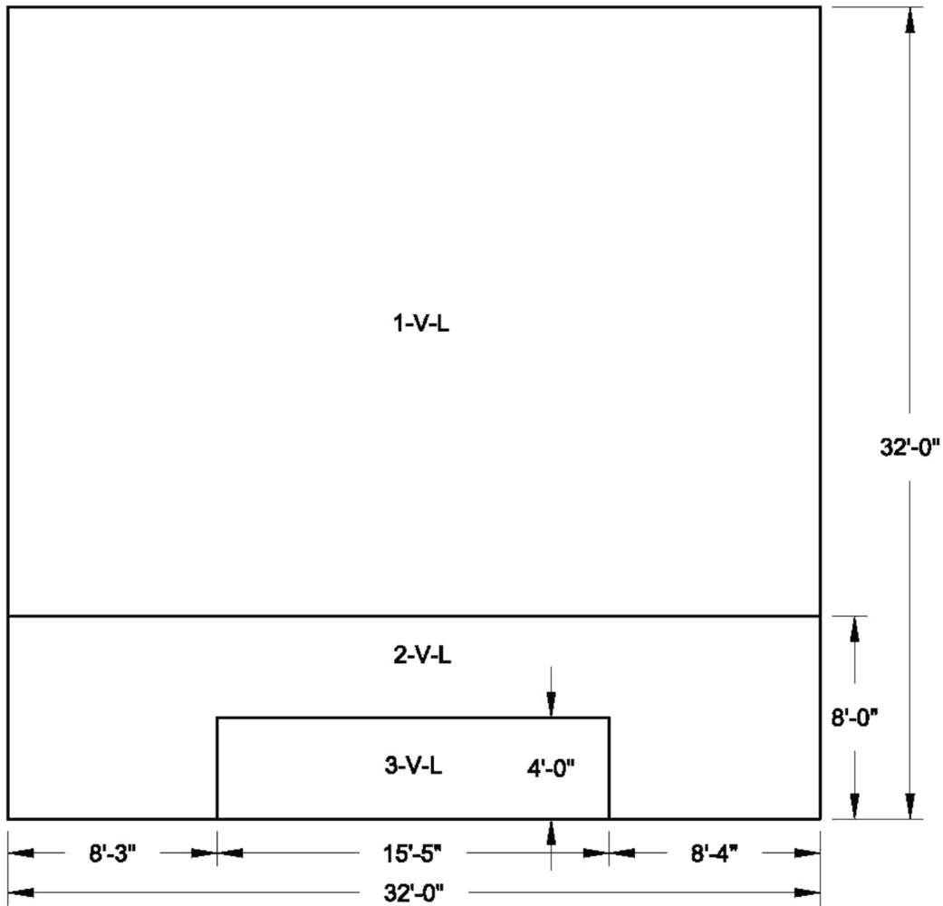
Figure 3H.6-186 Wall 12 Looking From Outside Vertical Reinforcement Zones Near Side Face
