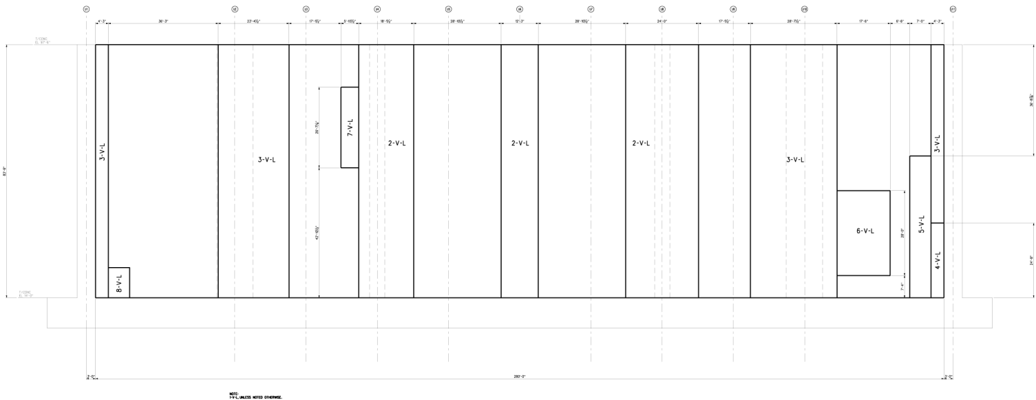
Figure 3H.6-88 Basin South Wall Looking North Vertical Reinforcement Zones Near Side Face
