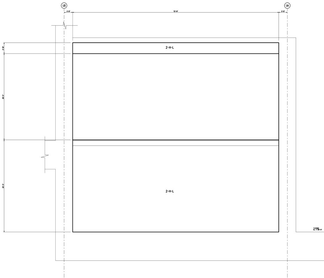
Figure 3H.6-78 Pumphouse Internal West Wall Looking West Horizontal Reinforcement Zones Far Side Face
