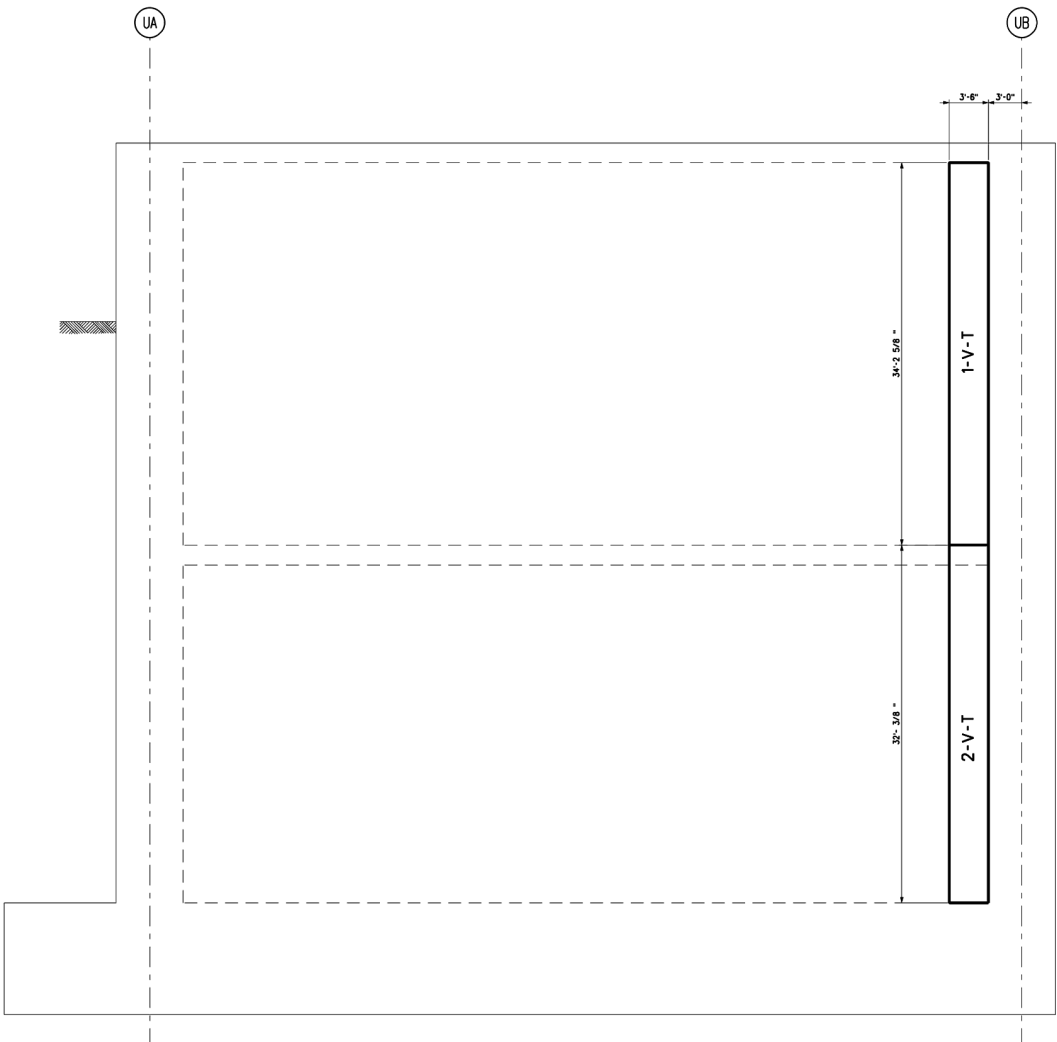
Figure 3H.6-71 Pumphouse West Wall Looking East Transverse Vertical Reinforcement Zones
