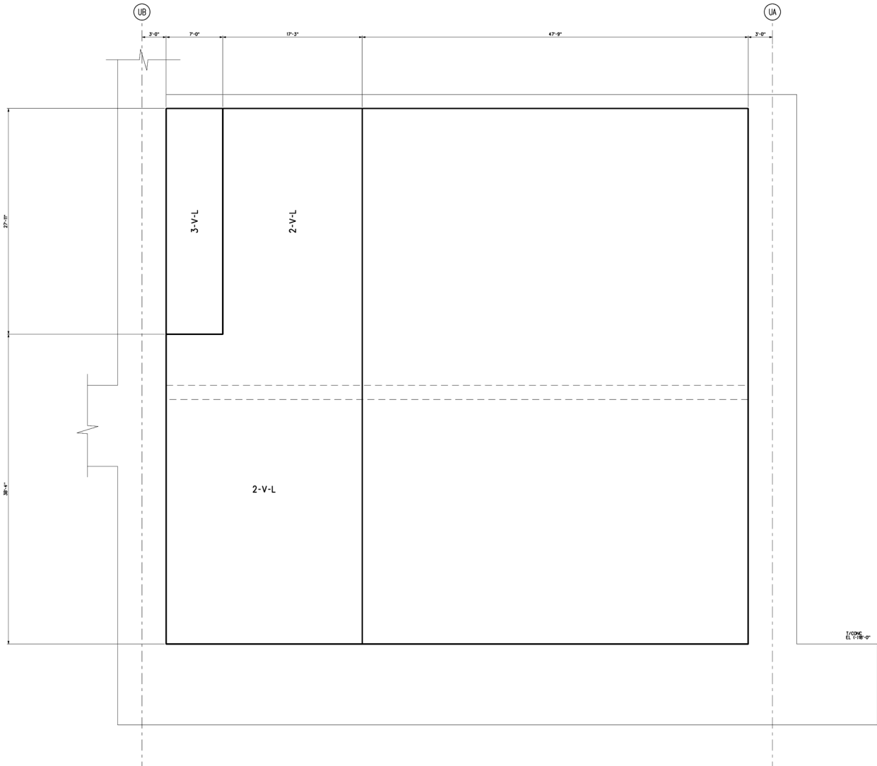
Figure 3H.6-60 Pumphouse East Wall Looking West Vertical Reinforcement Zones Far Side Face
