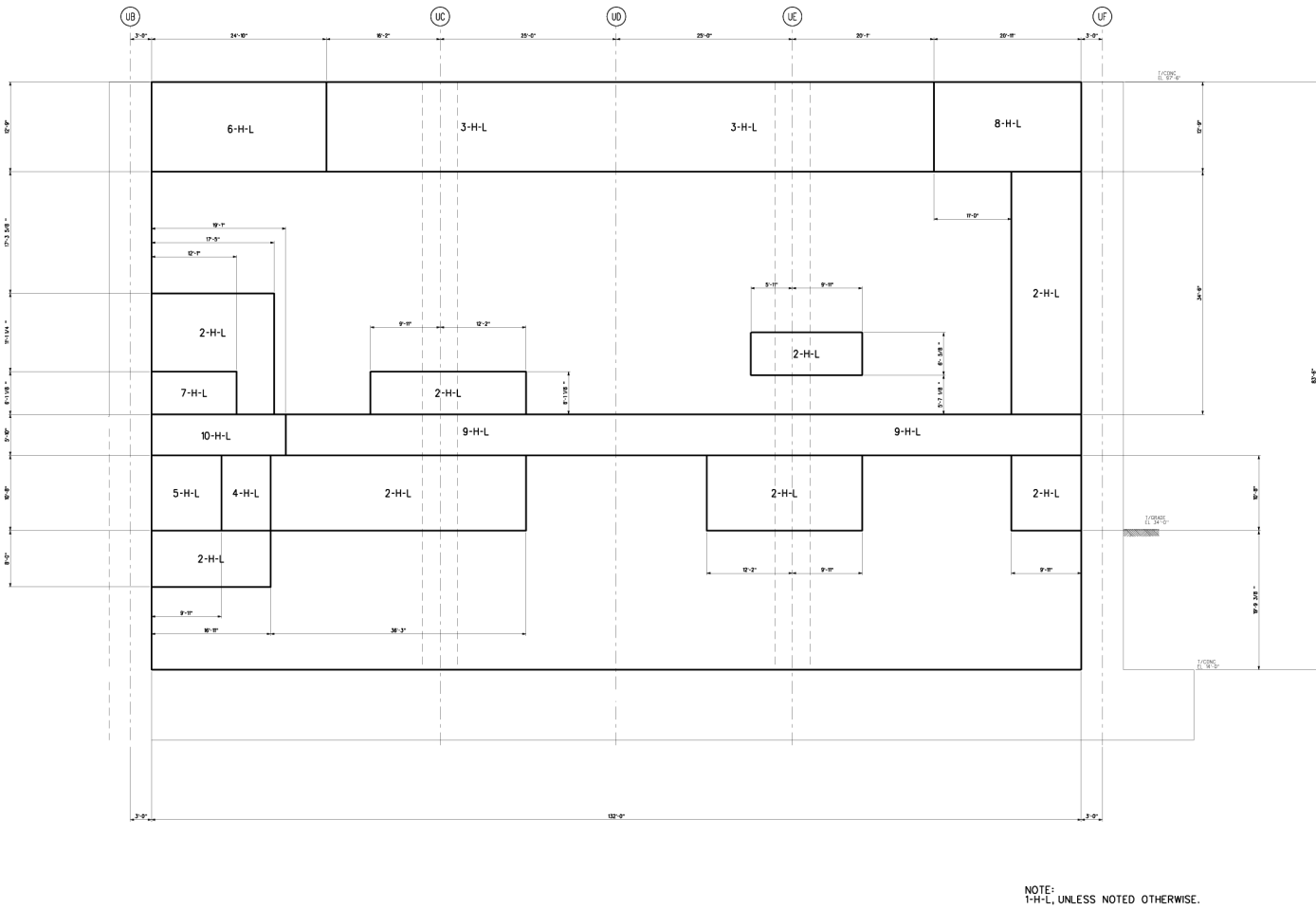
Figure 3H.6-99 Basin West Wall Looking East Horizontal Reinforcement Zones Far Side Face
