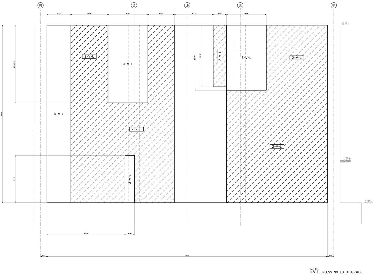
Figure 3H.6-98 Basin West Wall Looking East Vertical Reinforcement Zones Near Side Face
