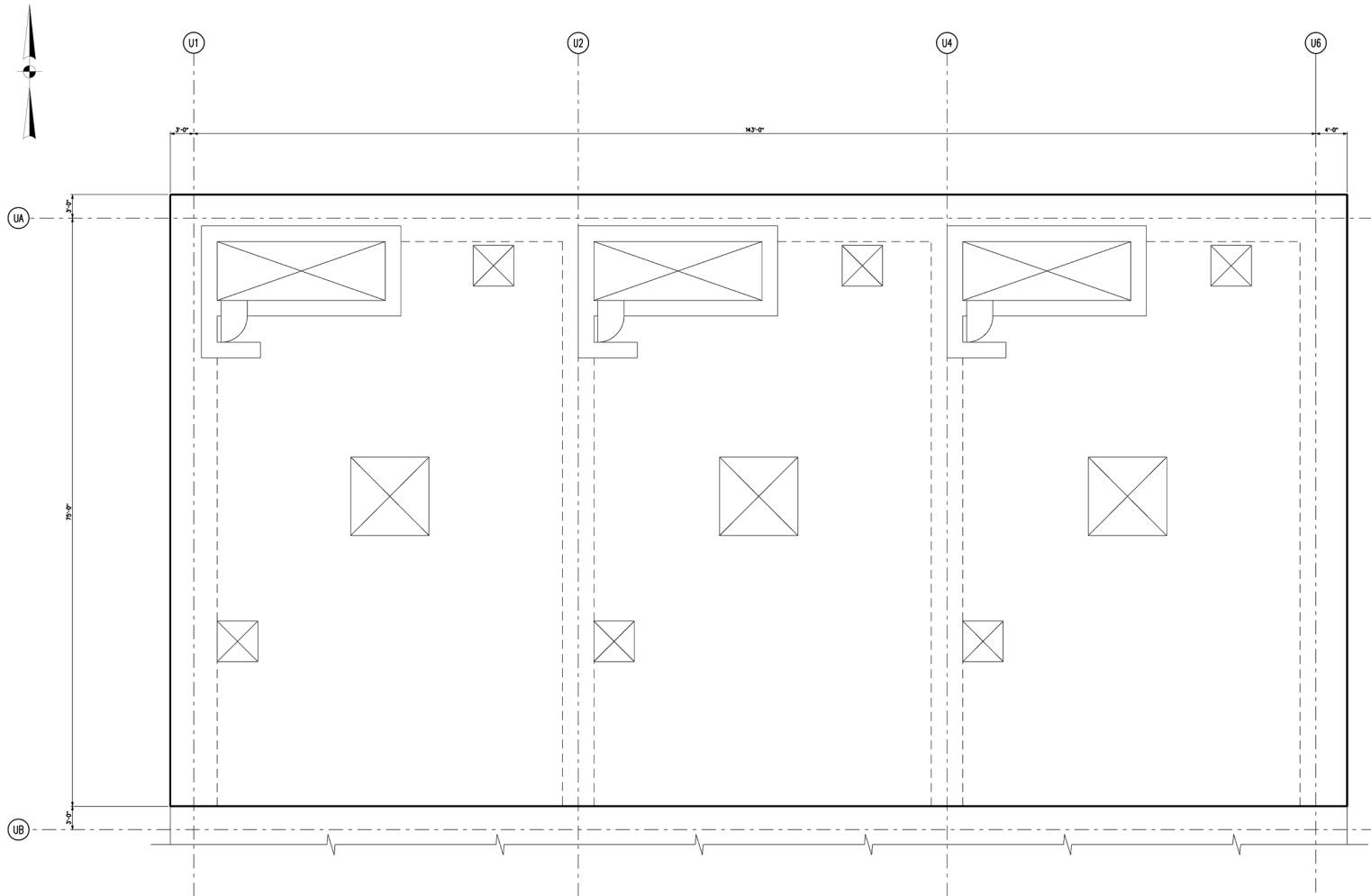
Figure 3H.6-134 Pumphouse Roof East/West Reinforcement Zones Top Face
