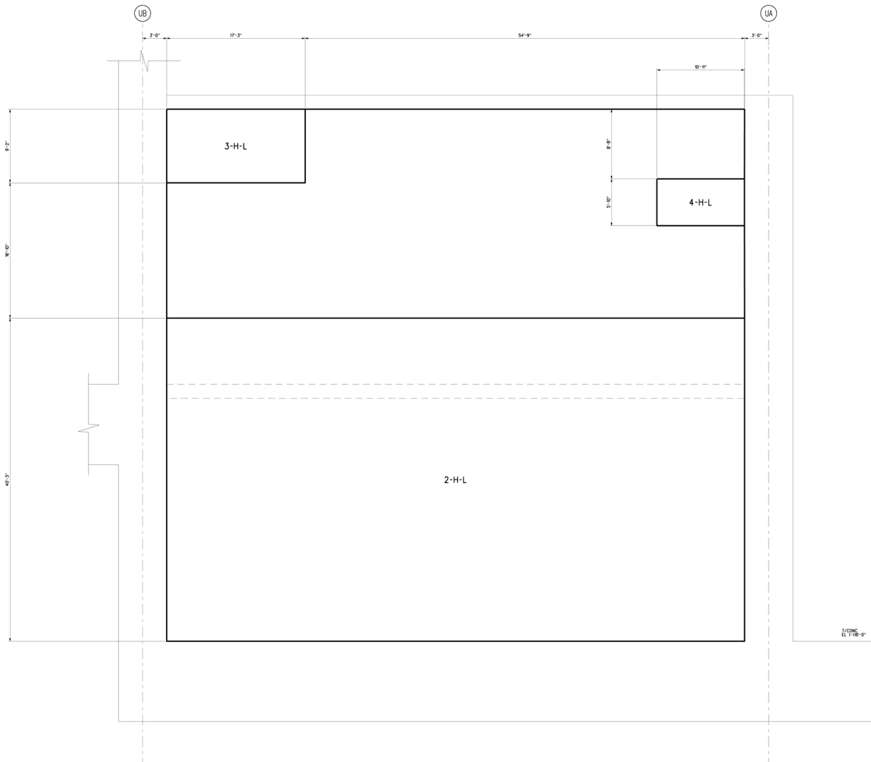
Figure 3H.6-59 Pumphouse East Wall Looking West Horizontal Reinforcement Zones Far Side Face
