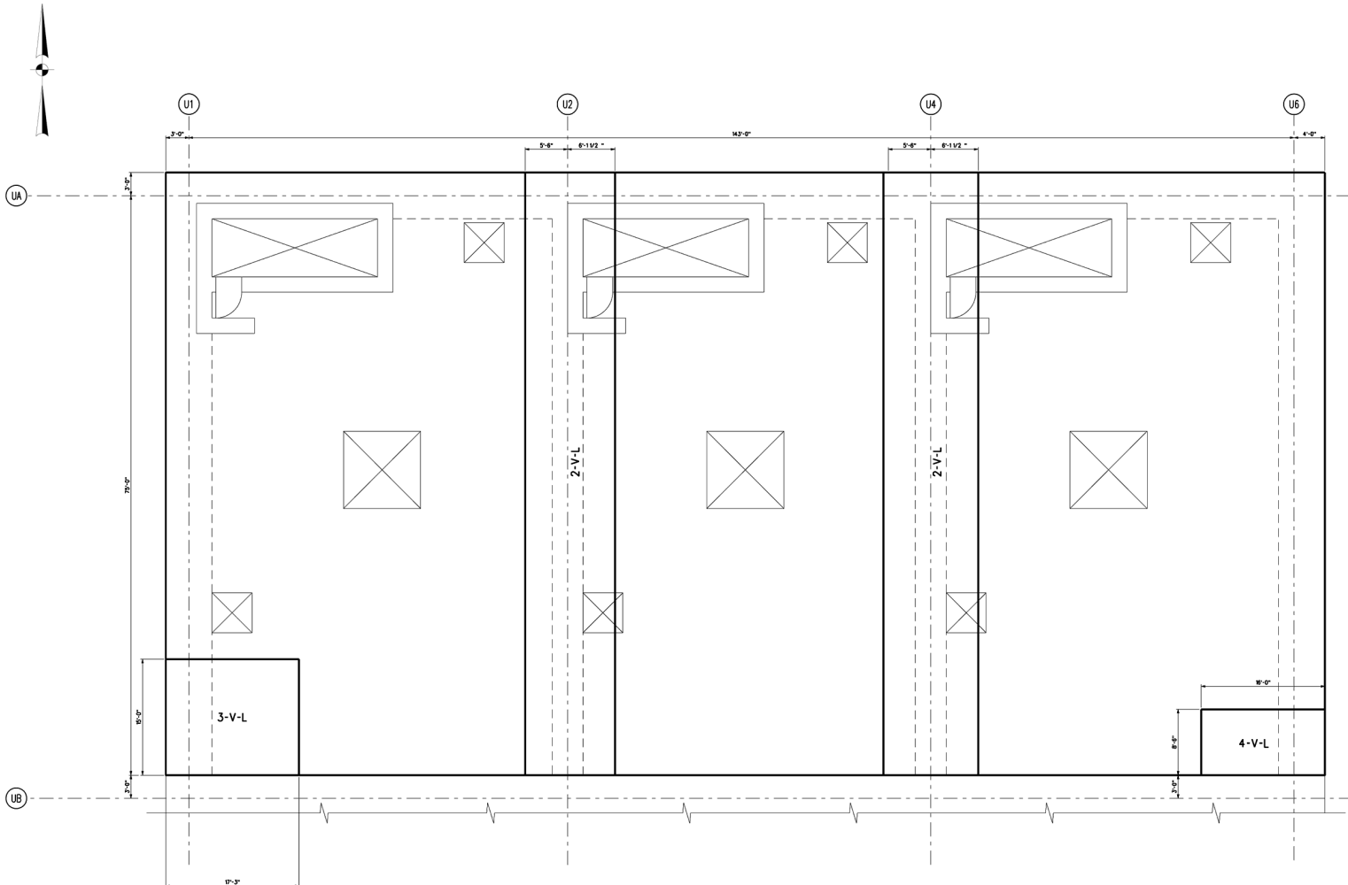
Figure 3H.6-135 Pumphouse Roof North/South Reinforcement Zones Top Face
