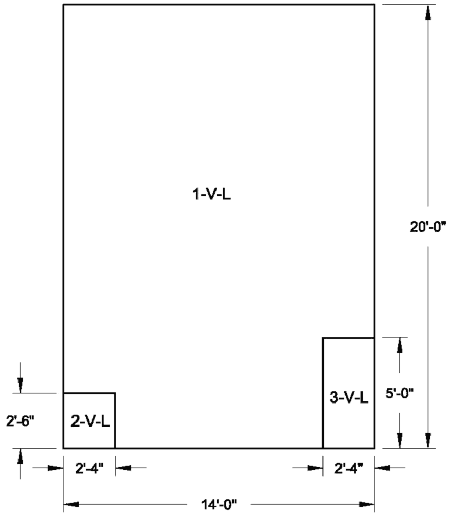
Figure 3H.6-178 Wall 10 Looking From Outside Vertical Reinforcement Zones Near Side Face
