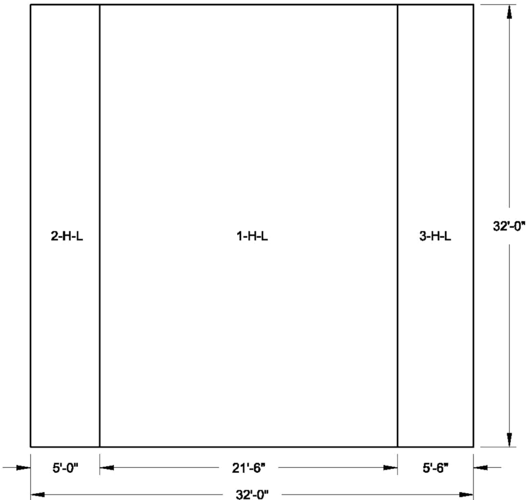
Figure 3H.6-190 Wall 13 Looking From Outside Horizontal Reinforcement Zones Near Side Face
