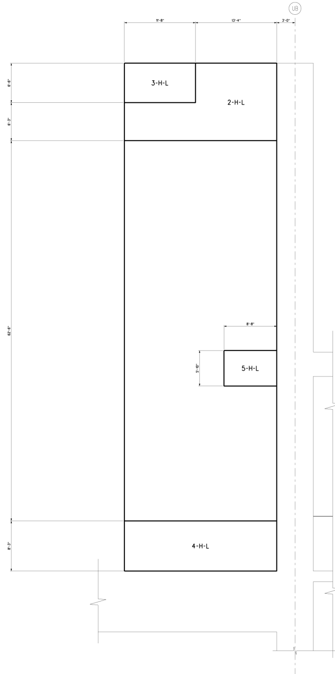
Figure 3H.6-102 Basin North Buttress Looking West & Basin South Buttress Looking East Horizontal Reinforcement Zones Near & Far Side Faces
