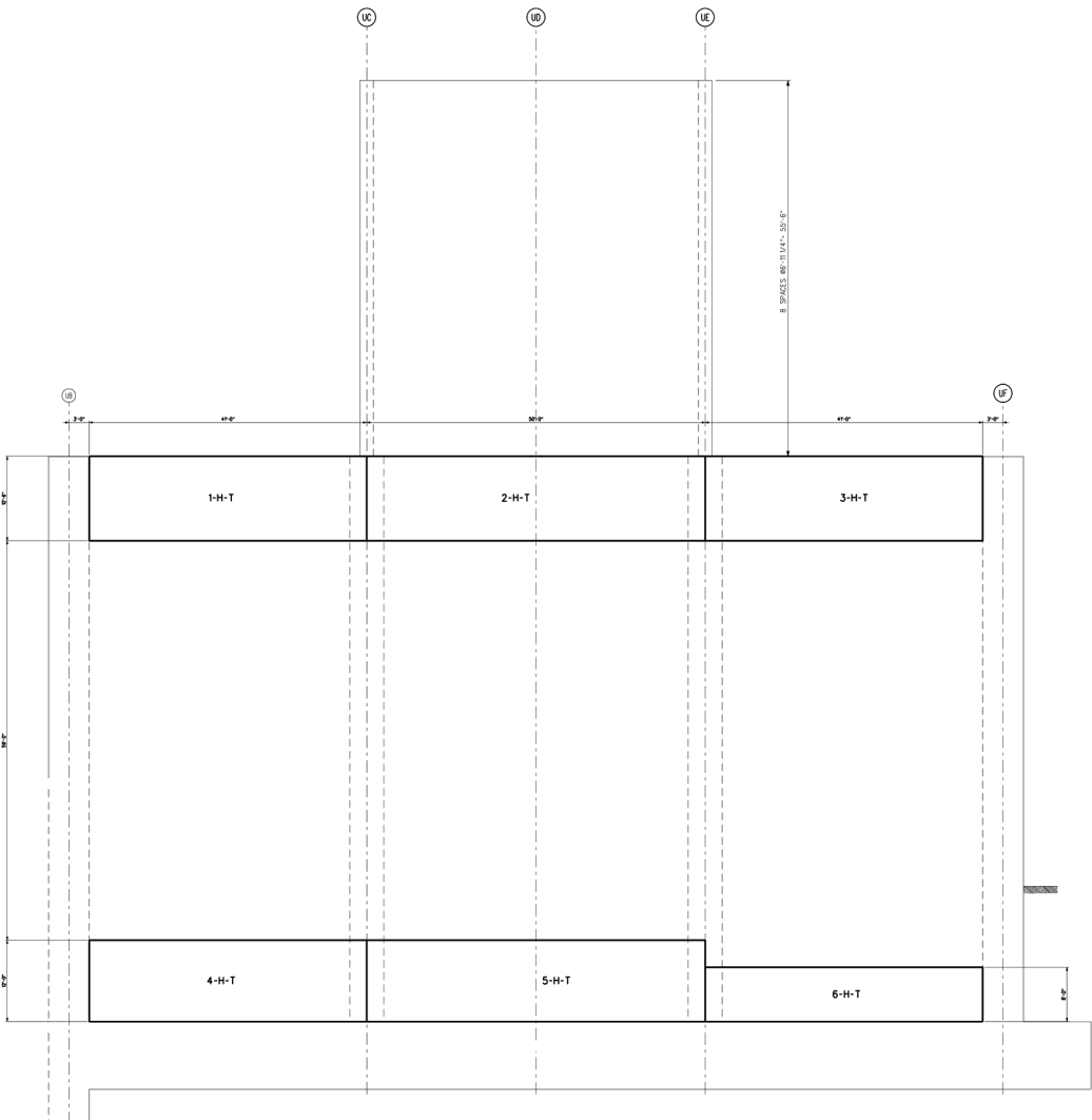
Figure 3H.6-101 Basin/Fan West Wall Looking East Transverse Horizontal Reinforcement Zones
