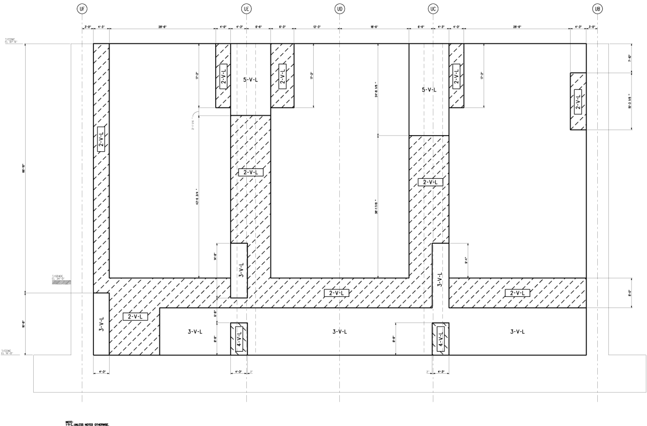
Figure 3H.6-95 Basin East Wall Looking West Vertical Reinforcement Zones Far Side Face
