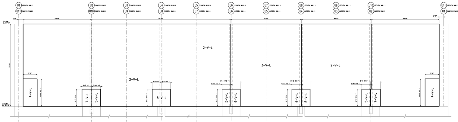
Figure 3H.6-109 Fan North (and South) Wall Looking South (North) Vertical Reinforcement Zones Near Side Face
