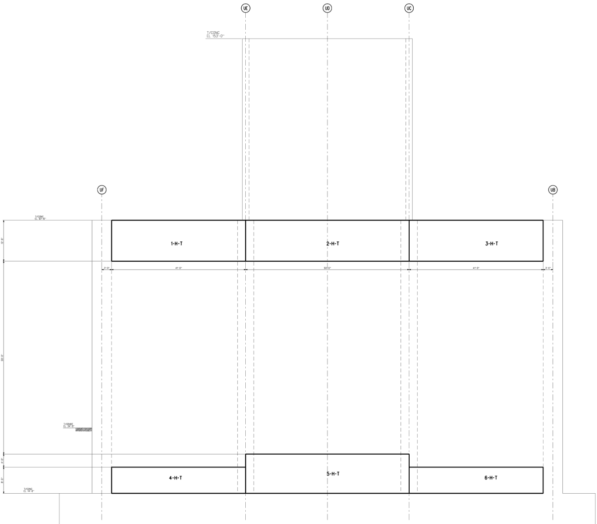
Figure 3H.6-96 Basin/Fan East Wall Looking West Transverse Horizontal Reinforcement Zones
