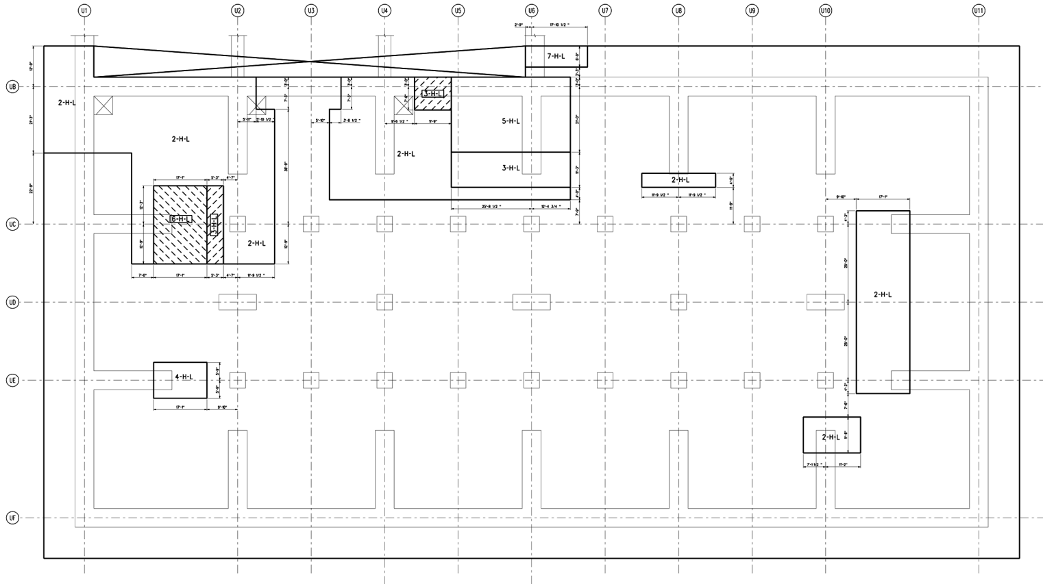
Figure 3H.6-129 Ultimate Heat Sink Basin Base Mat Plan East/West Reinforcement Zones Top Face
