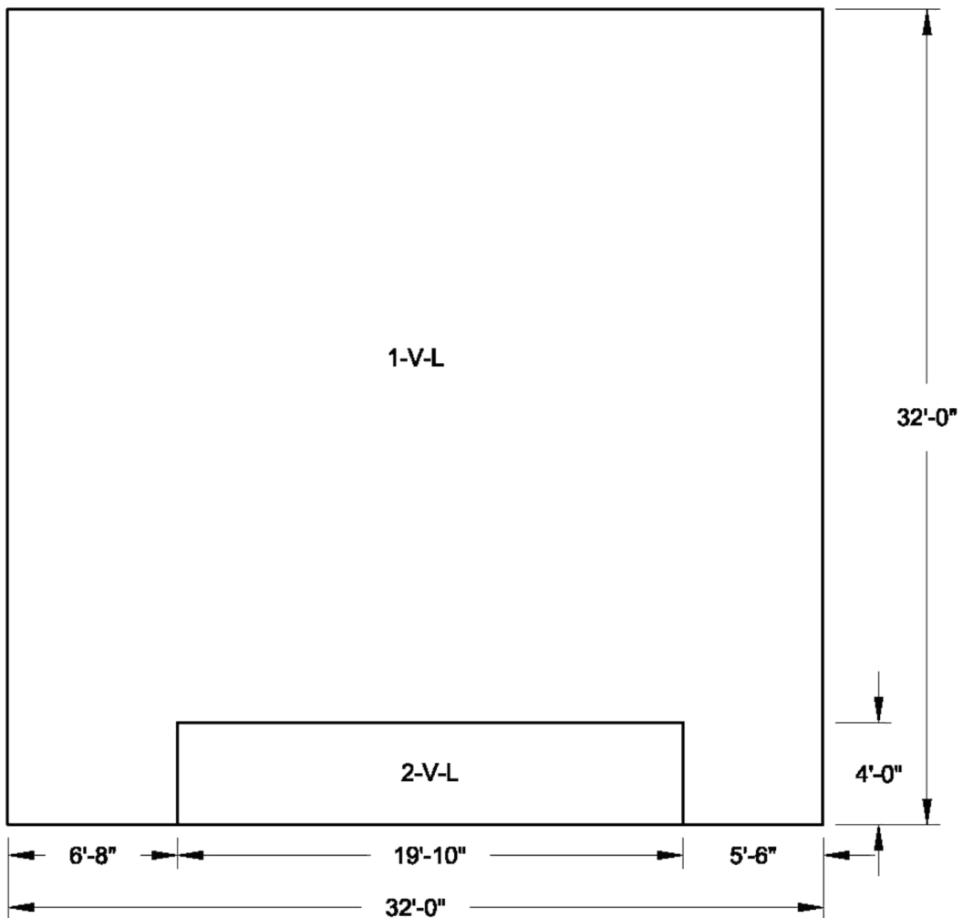
Figure 3H.6-191 Wall 13 Looking From Outside Vertical Reinforcement Zones Near Side Face
