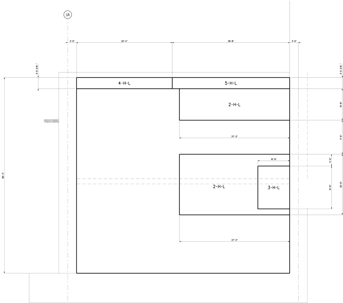
Figure 3H.6-69 Pumphouse West Wall Looking East Horizontal Reinforcement Zones Far Side Face
