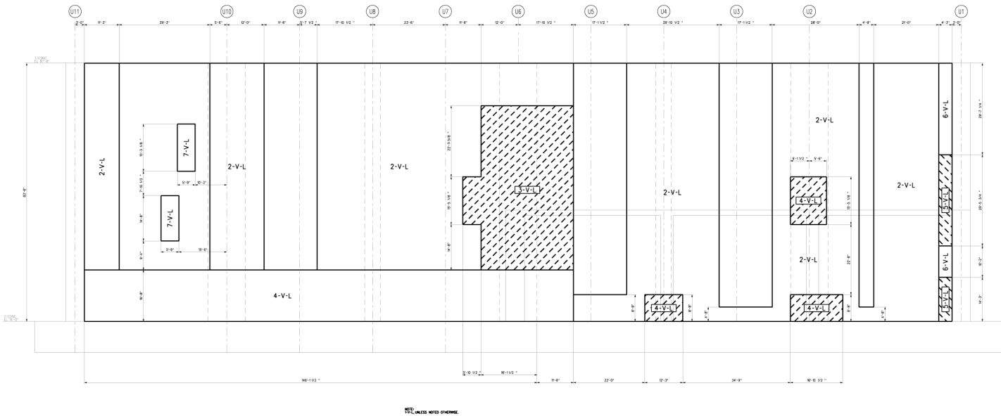
Figure 3H.6-85 Basin North Wall Looking South Vertical Reinforcement Zones Far Side Face
