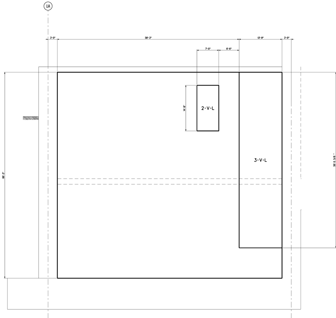
Figure 3H.6-68 Pumphouse West Wall Looking East Vertical Reinforcement Zones Near Side Face
