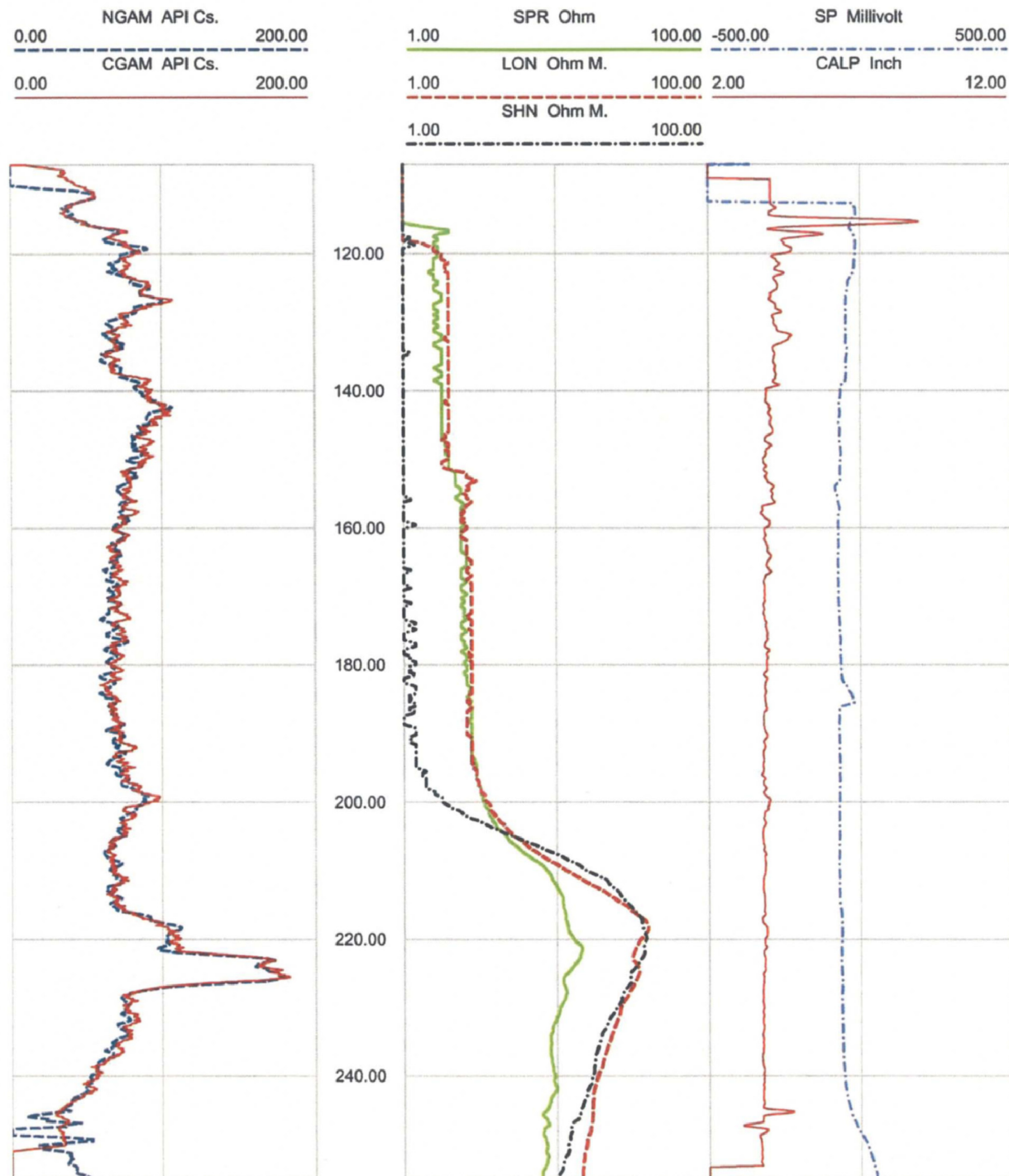
Figure 19. Boring B-608 (DH) lower section, Caliper, Natural gamma, Resistivity and SP logs
