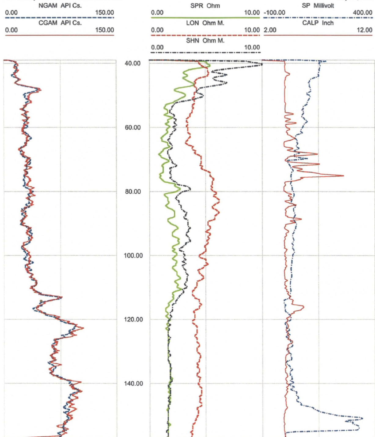
Figure 15. Boring B-604 (DH) lower section, Caliper, Natural gamma, Resistivity and SP logs
