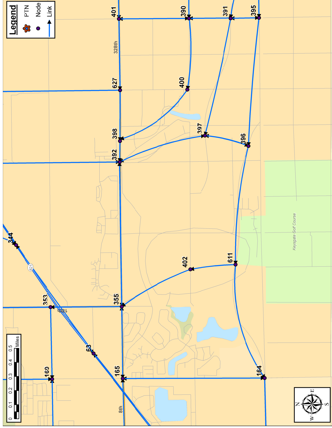
Figure K-14. Turkey Point Plant Site Link-Node Analysis Network Inset 13
