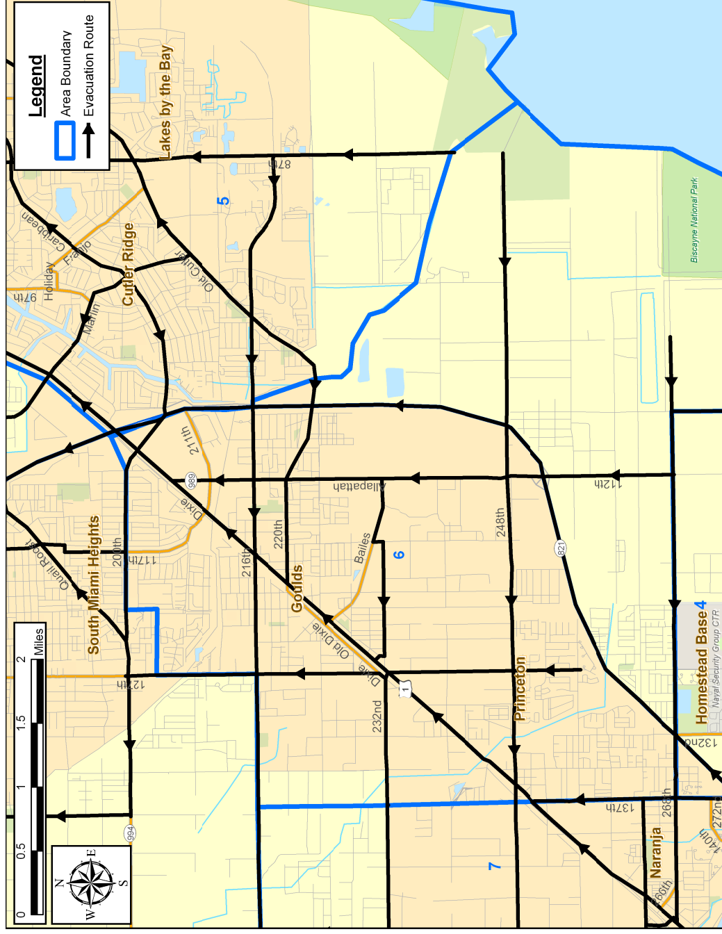
Figure 10-5. Evacuation Routes for Area 6
