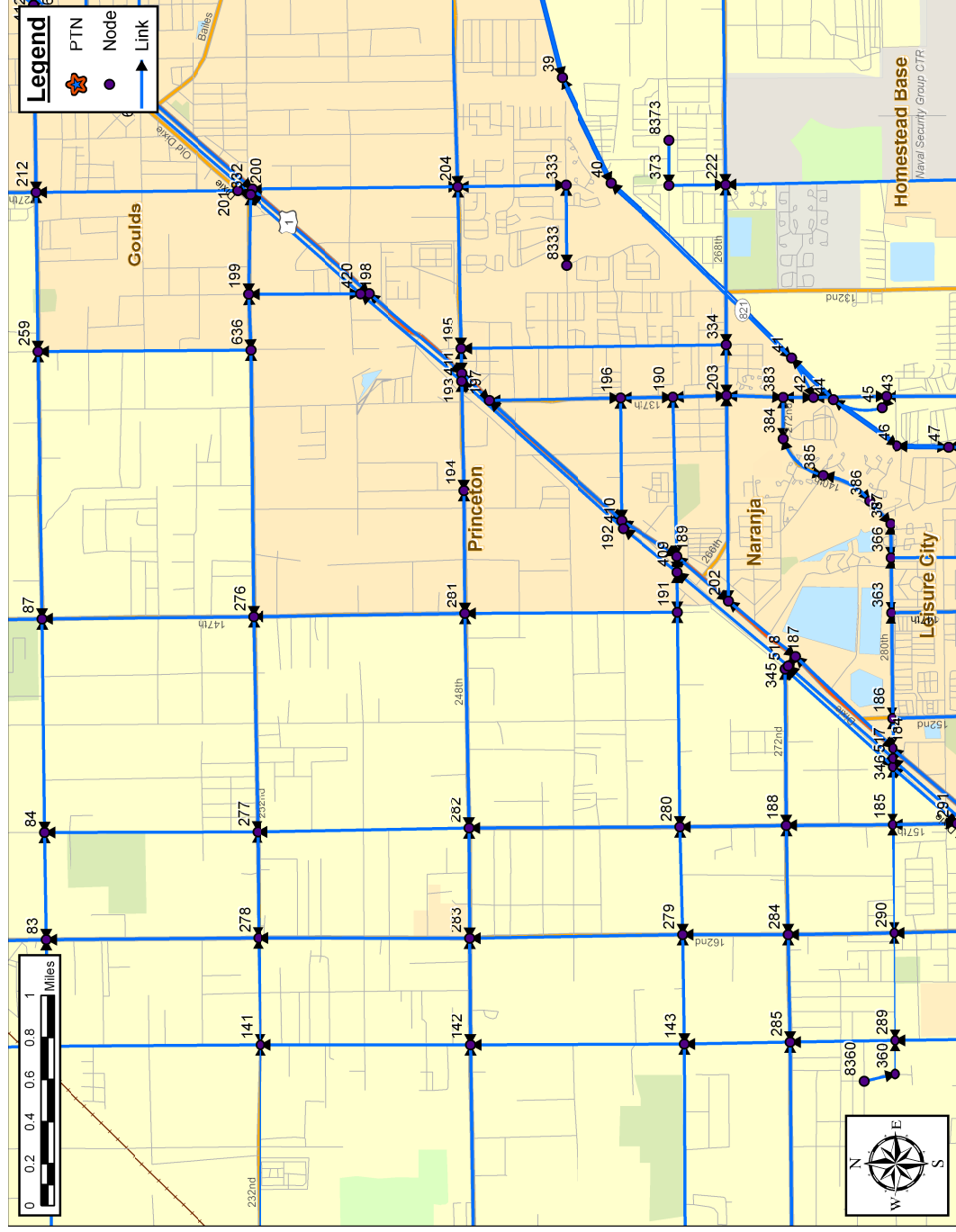
Figure K-9. Turkey Point Plant Site Link-Node Analysis Network Inset 8
