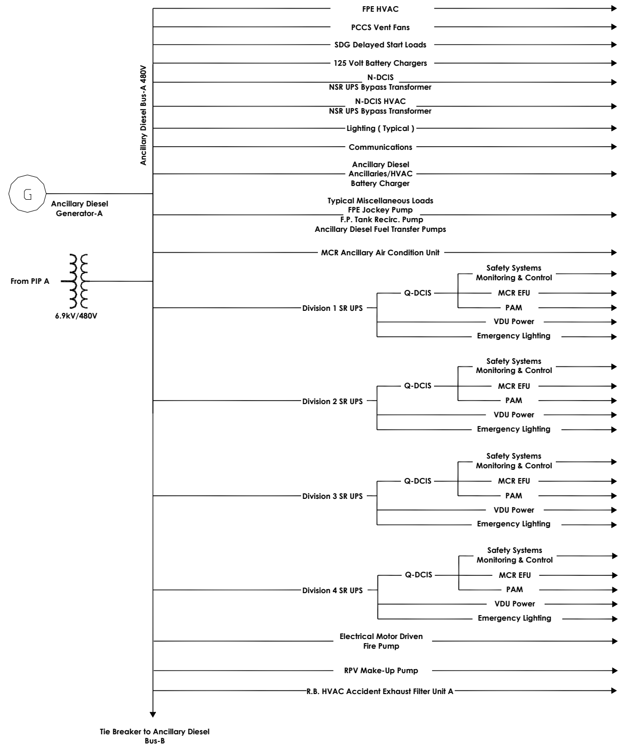
Figure 8.3-3. Ancillary Power Functional Figure Sh 1 of 1
