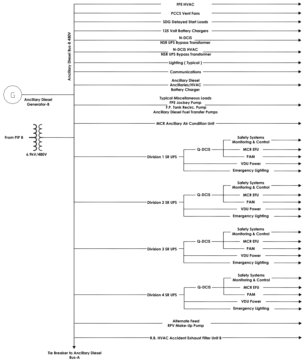
Figure 8.3-3. Ancillary Power Functional Figure Sh 1 of 1
