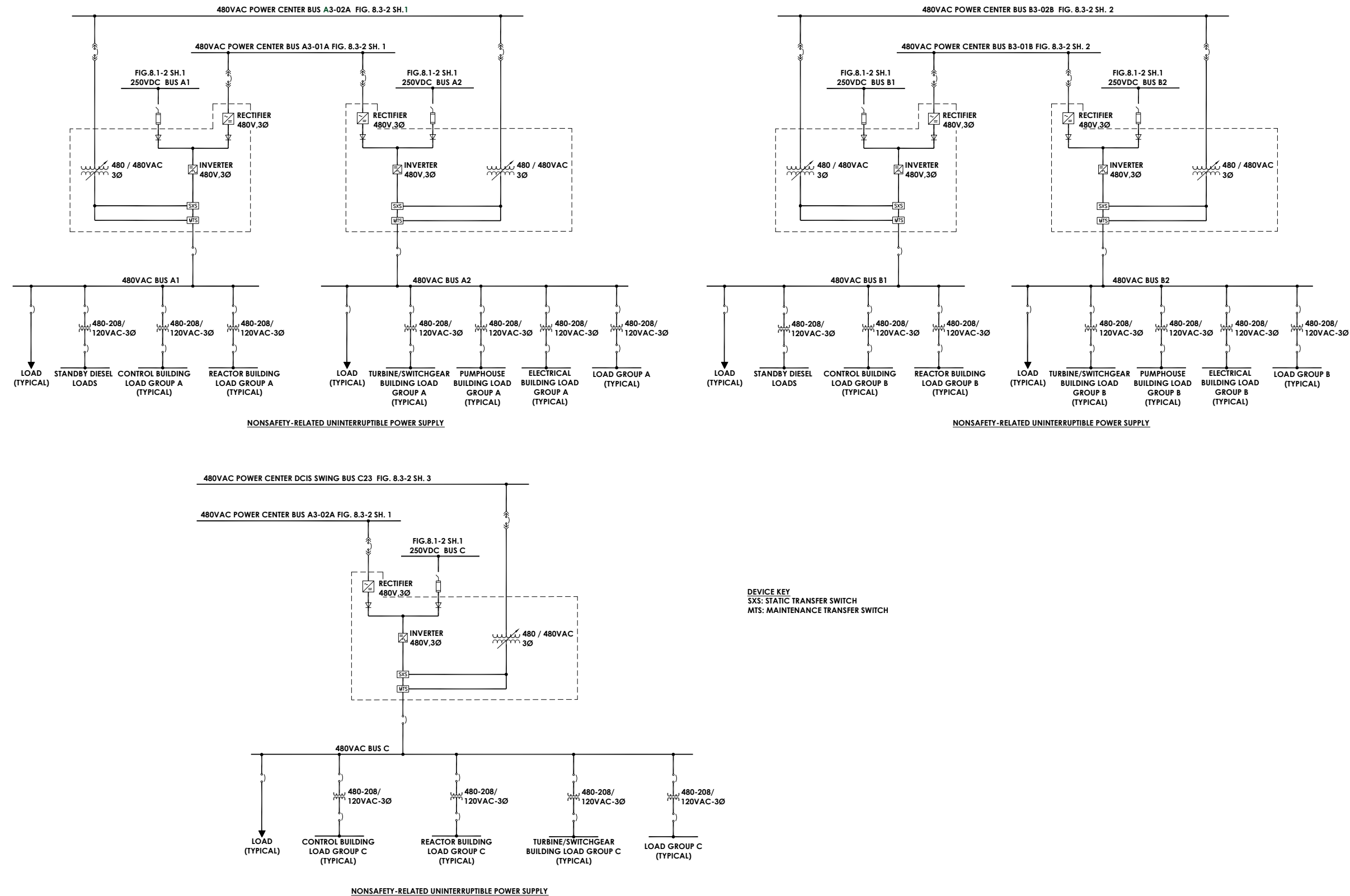
Figure 8.1-5. Uninterruptible AC Power Supply (Nonsafety-Related) Sh 1 of 2
