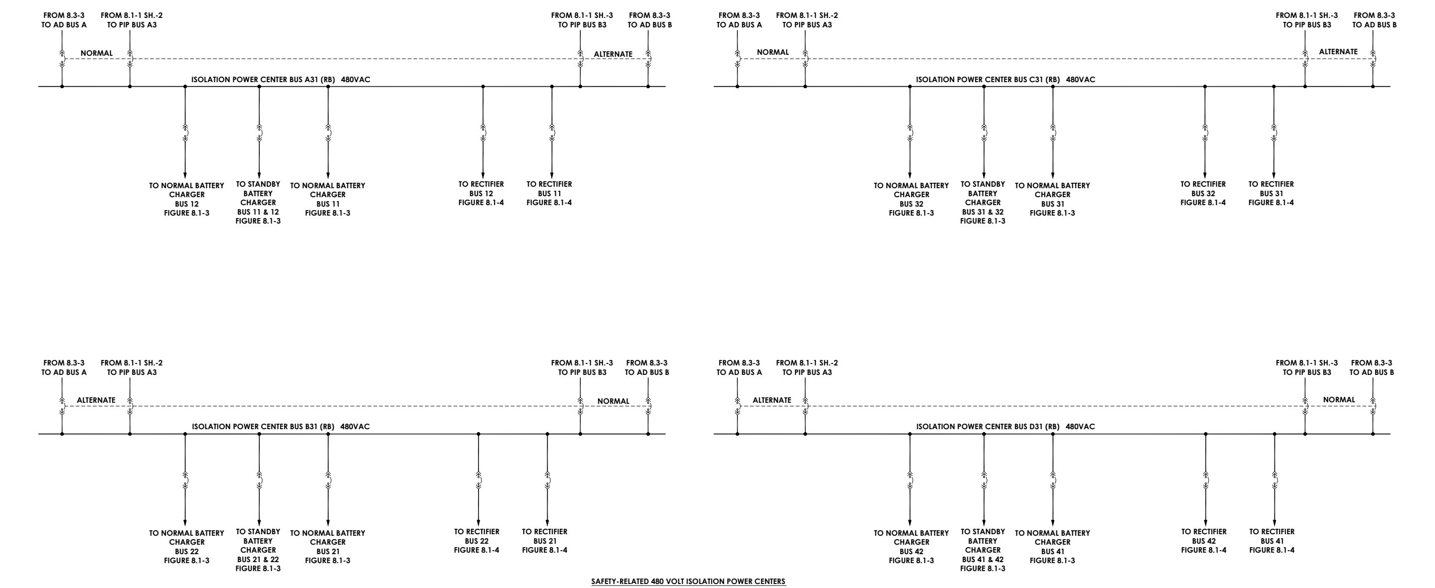
Figure 8.3-1. Safety-Related 480 Volt Power Centers Sh 1 of 1
