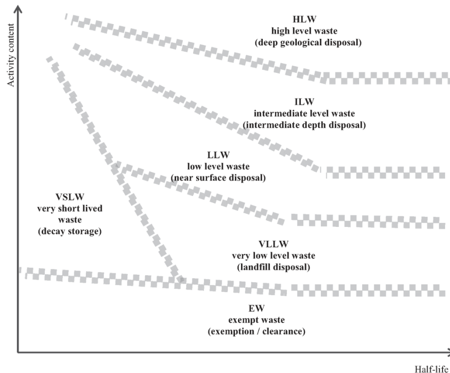
Figure 1. Conceptual Illustration of IAEA Waste Classification System
