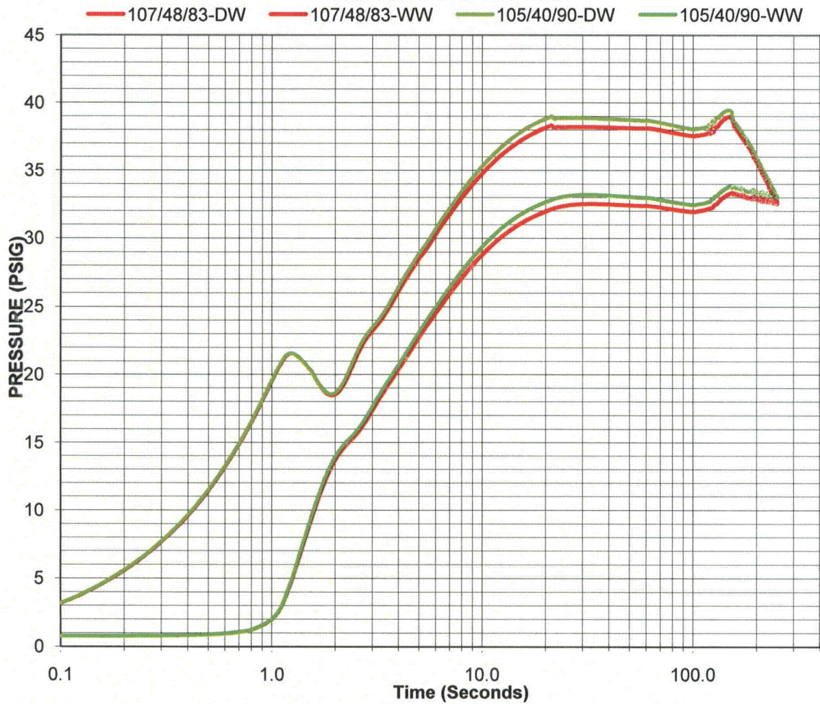
FIGURE 3 - CASE 2 & 2B - EPU GOTHIC PRESSURE RESPONSE - 105/40/90 VS. 107/48/83
