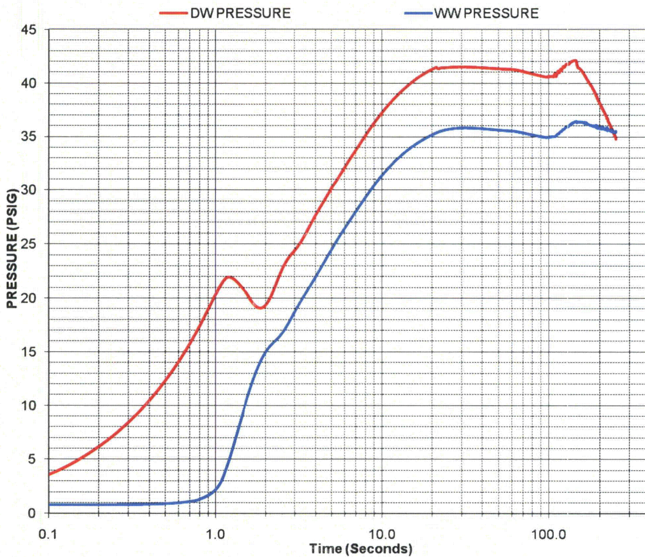
FIGURE 4 - CASE 3 - EPU PRESSURE RESPONSE (70/20/90)
