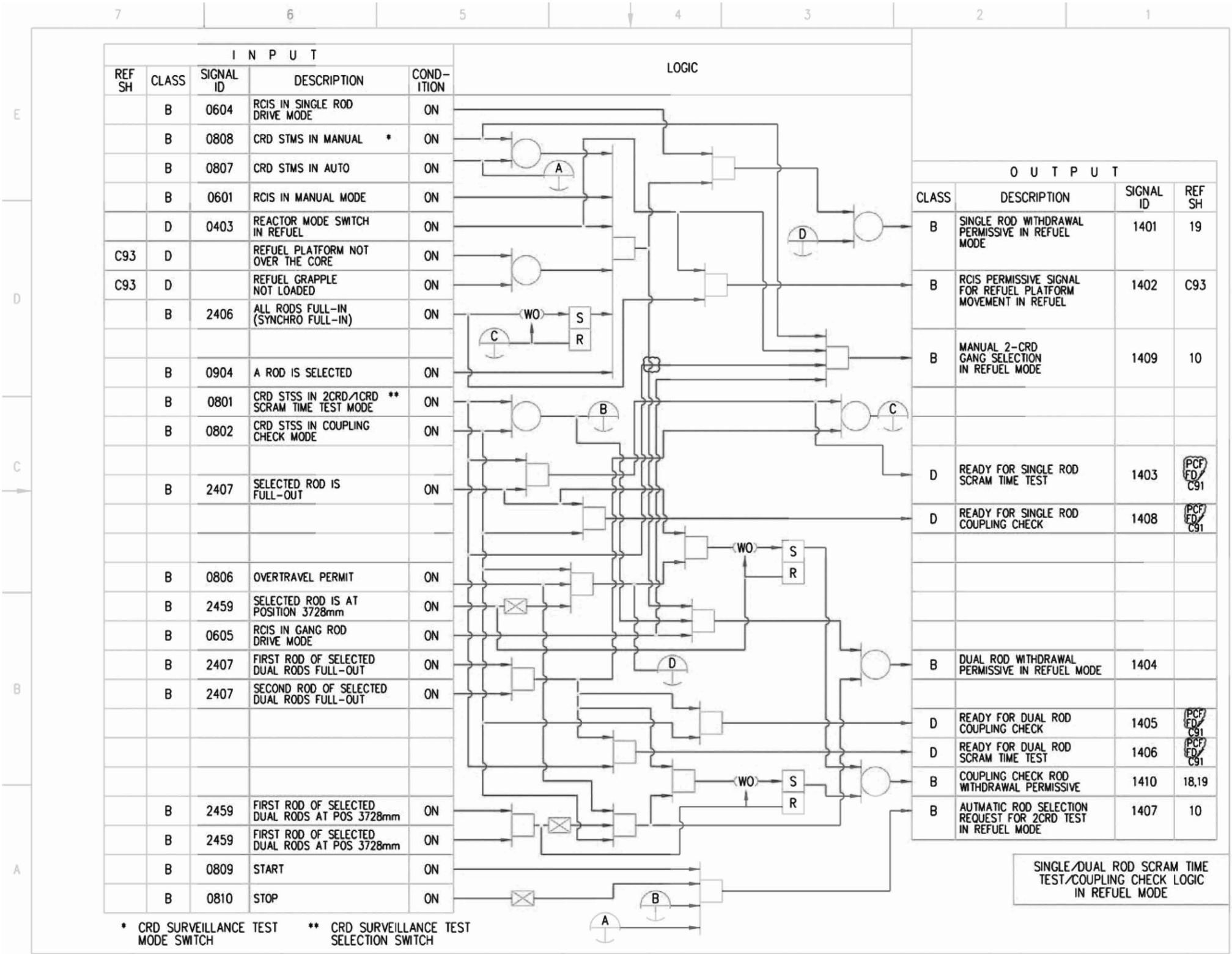
Figure 7.7-3 – Rod Control and Information System IBD (Sheet 14 of 87)
