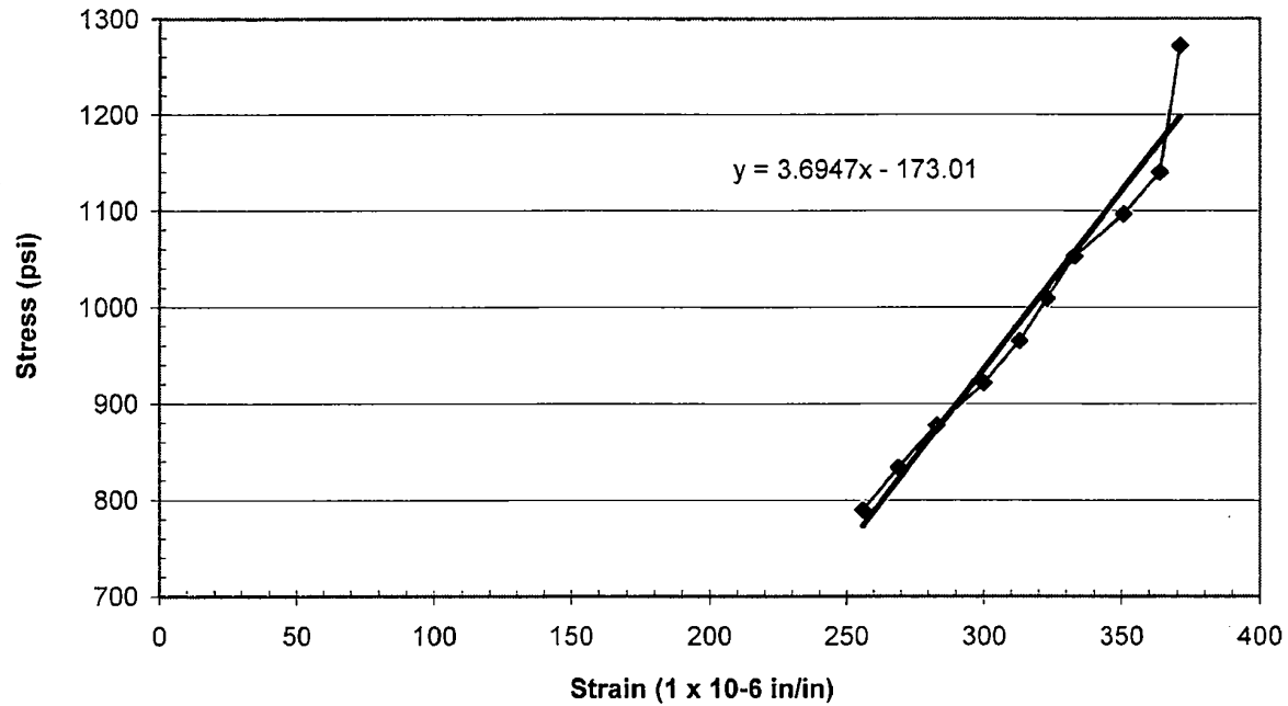
Tangent Modulus Corresponding to 40%-60% of Ultimate Strength B-610 R-7 49.9-50.7
