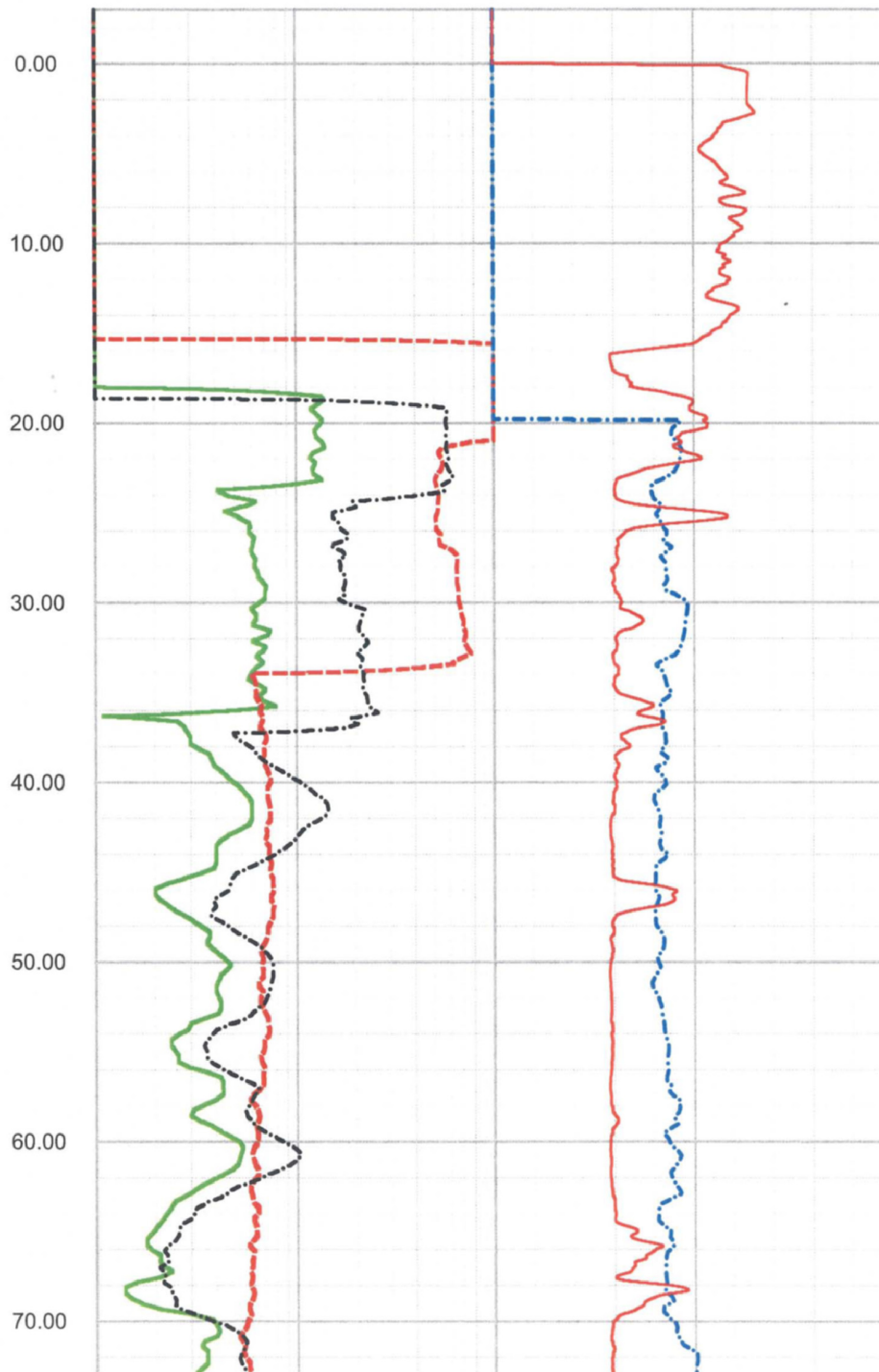
FPL Turkey Point COL Boring B-701 (DH) upper section ELOG, Caliper and Natural Gamma rev 1 Sheet 1 of 3
