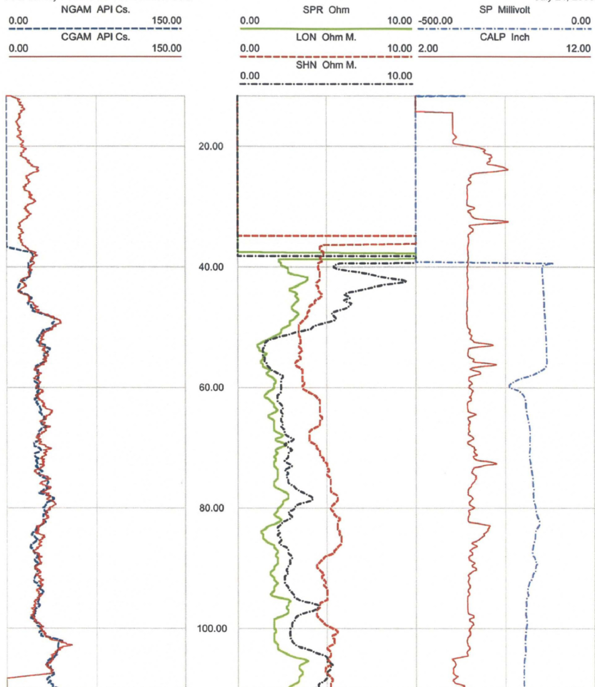
Figure 22. Boring B-610 (DH) upper section, Caliper, Natural gamma, Resistivity and SP logs
