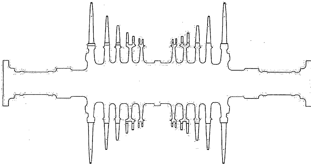
Figure 2-1 Typical Integral Rotor Structure
