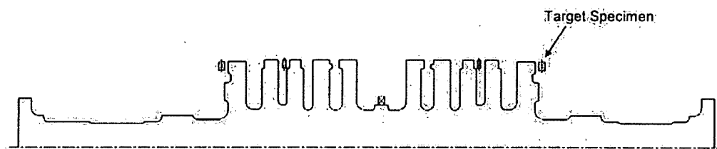
Figure 2.1-1 Typical Integral Rotor Material Test Locations
