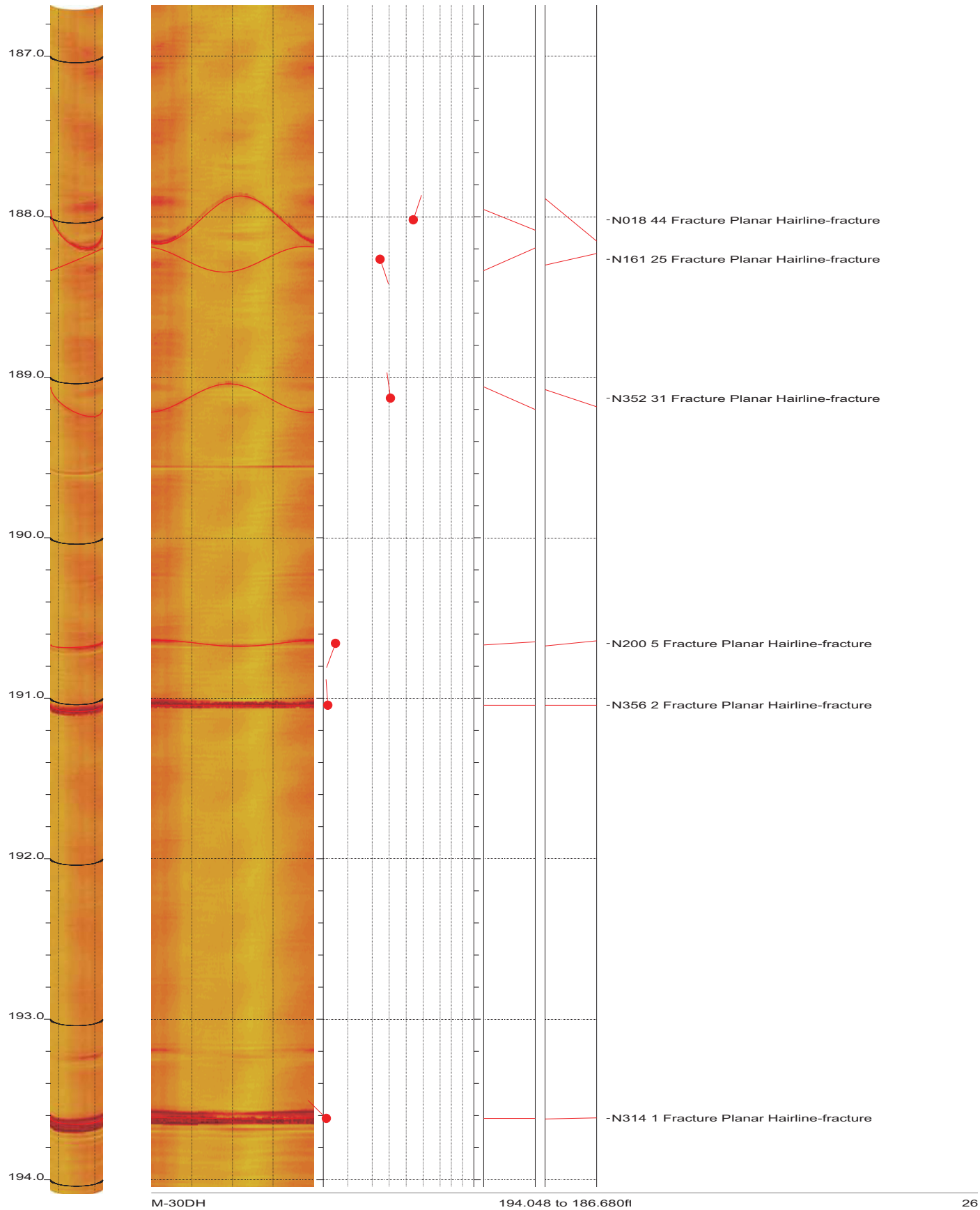
North Anna Boring M-30DH Acoustic Televiewer Dips rev 1 Sheet 26 of 27
