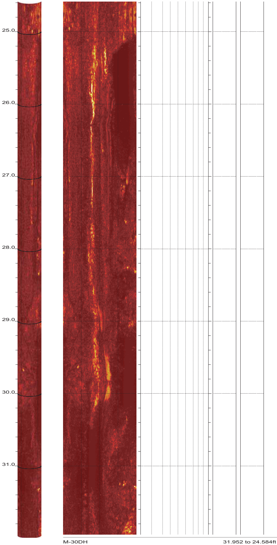
North Anna Boring M-30DH Acoustic Televiewer Dips rev 1 Sheet 4 of 27
