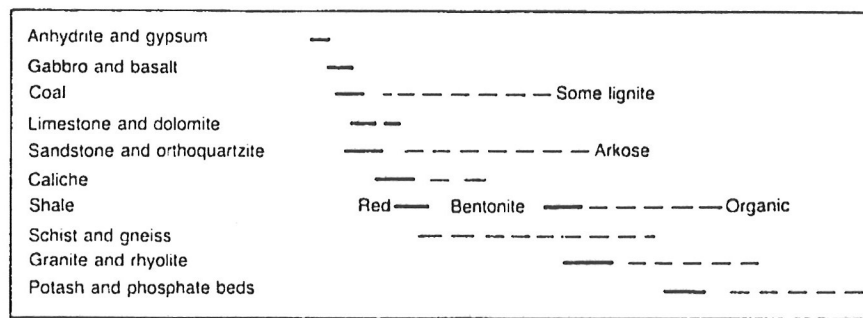
RADIOACTIVITY INCREASES → FIG. 6 Range of Relative Gamma Activity of Common Rocks
