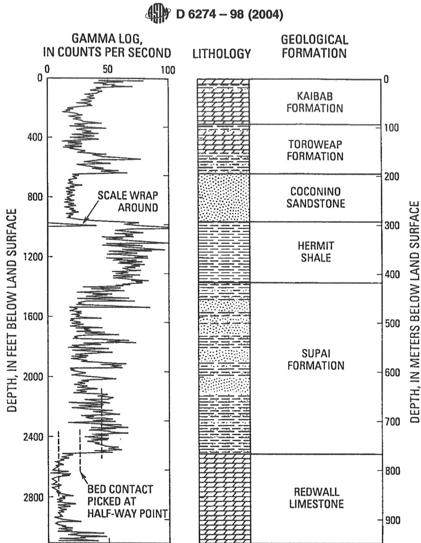
FIG. 1 Example of a Gamma Log From Near the South Rim of the Grand Canyon
