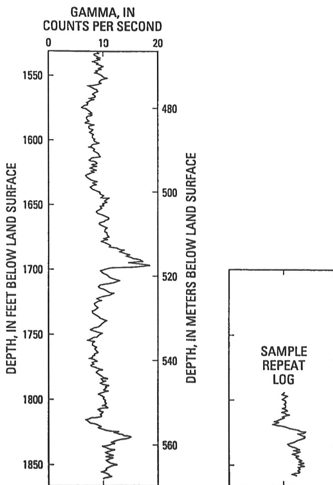
FIG. 5 Example of a Gamma Log From a Basalt Formation of Very Low Gamma Activity
