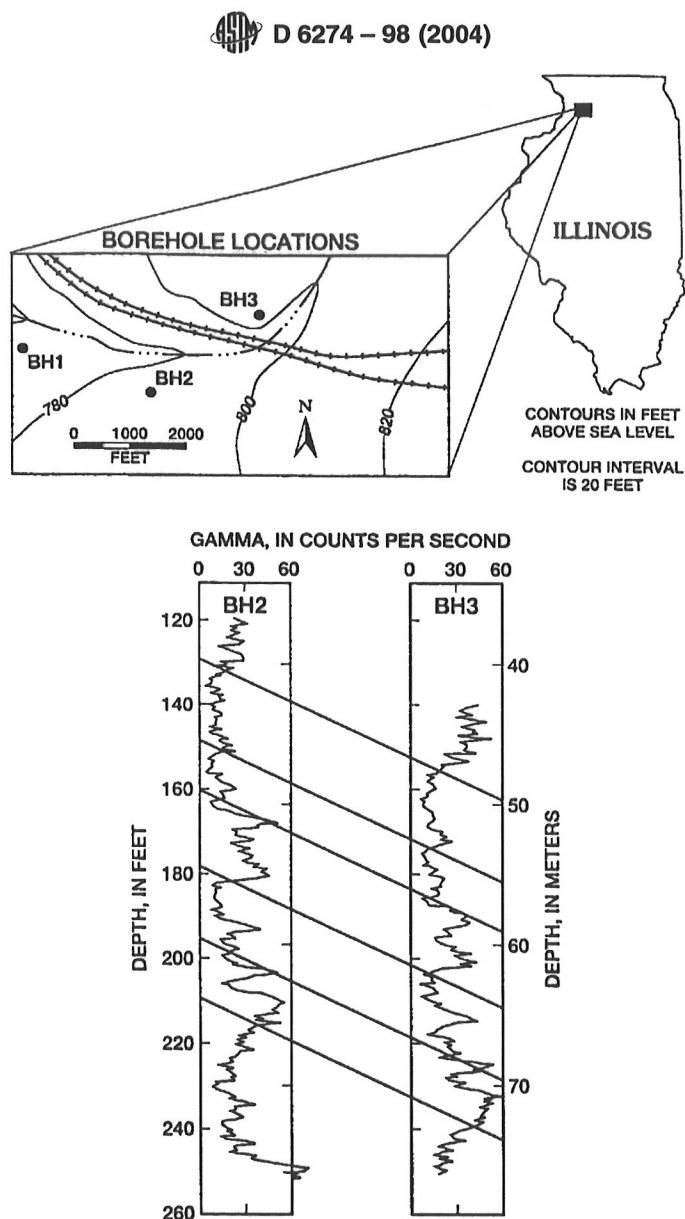
FIG. 2 Example of Gamma Logs From Two Boreholes
