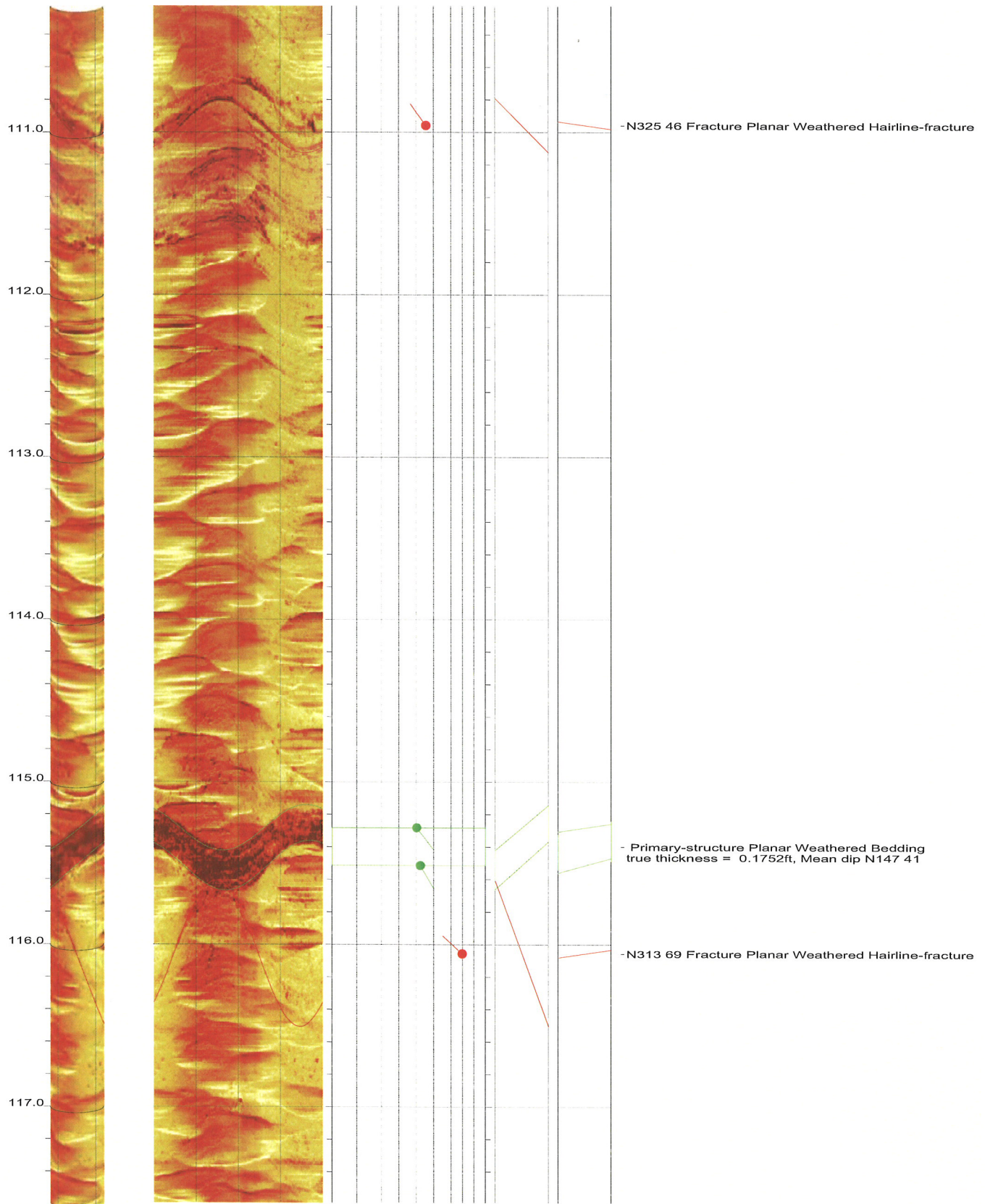
North Anna COL Boring B-909 Acoustic Televiwer Dips Sheet 16 of 28
