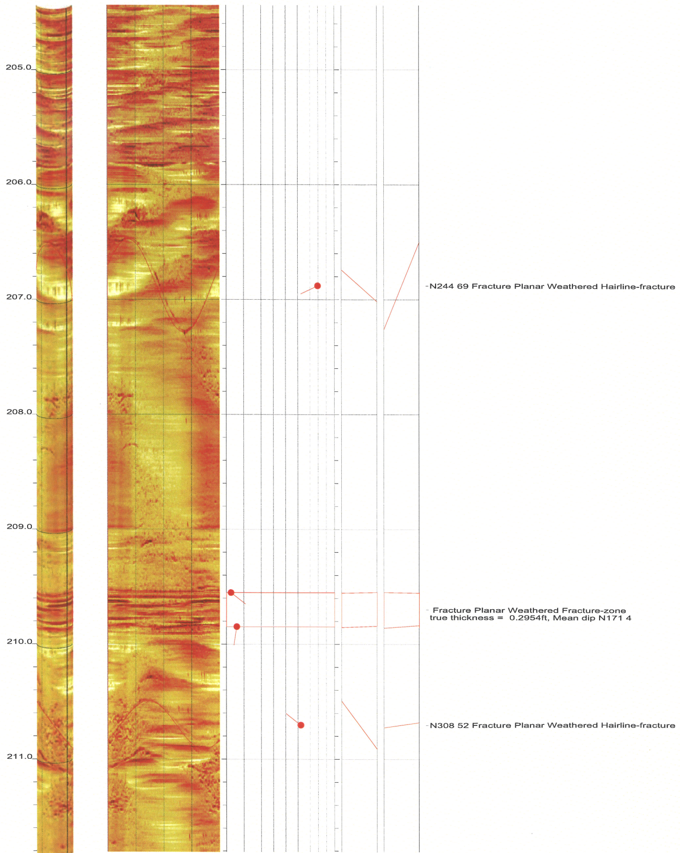
North Anna COL Boring B-901 Acoustic Televiewer Dips Sheet 24 of 36
