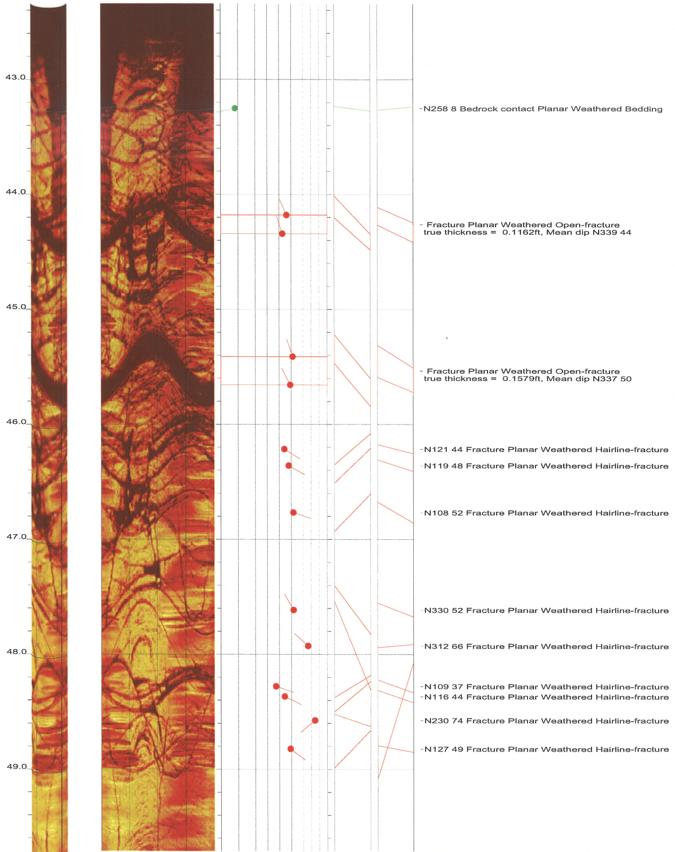
North Anna COL Boring B-901 Acoustic Televiewer Dips Sheet 2 of 36
