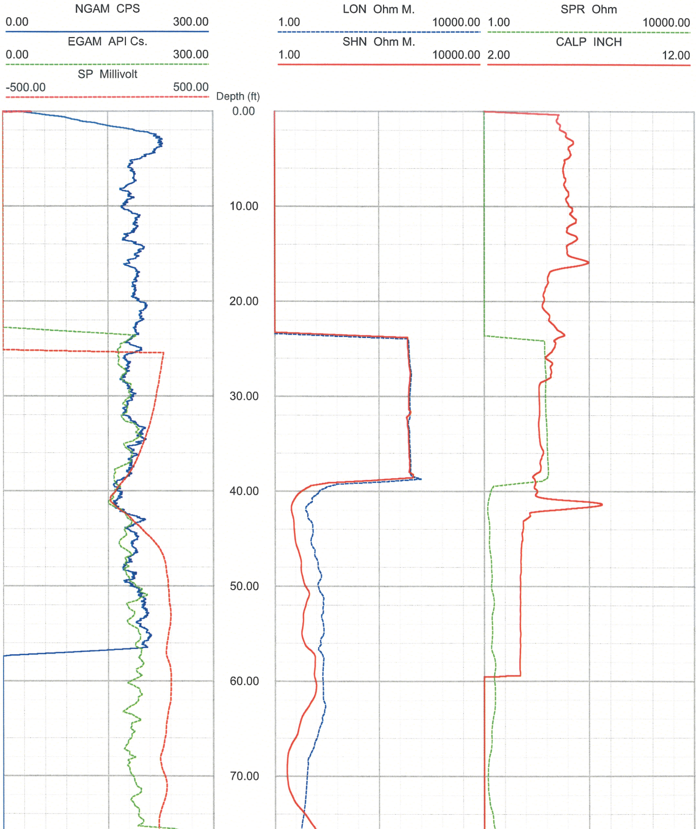
North Anna COL Boring B-901 upper section ELOG, Caliper and Gamma Sheet 2 of 3
