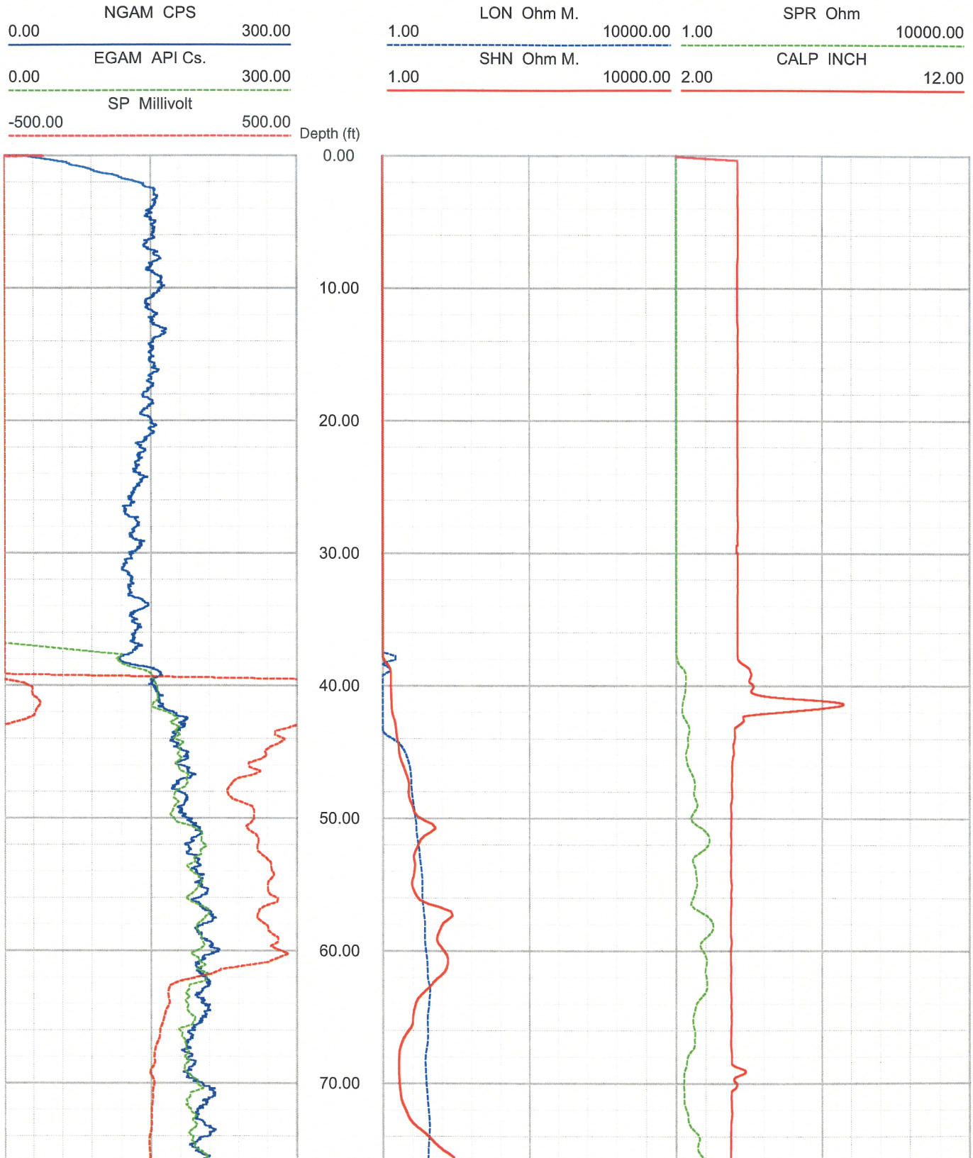
North Anna COL Boring B-901 lower section ELOG, Caliper and Gamma Sheet 2 of 5
