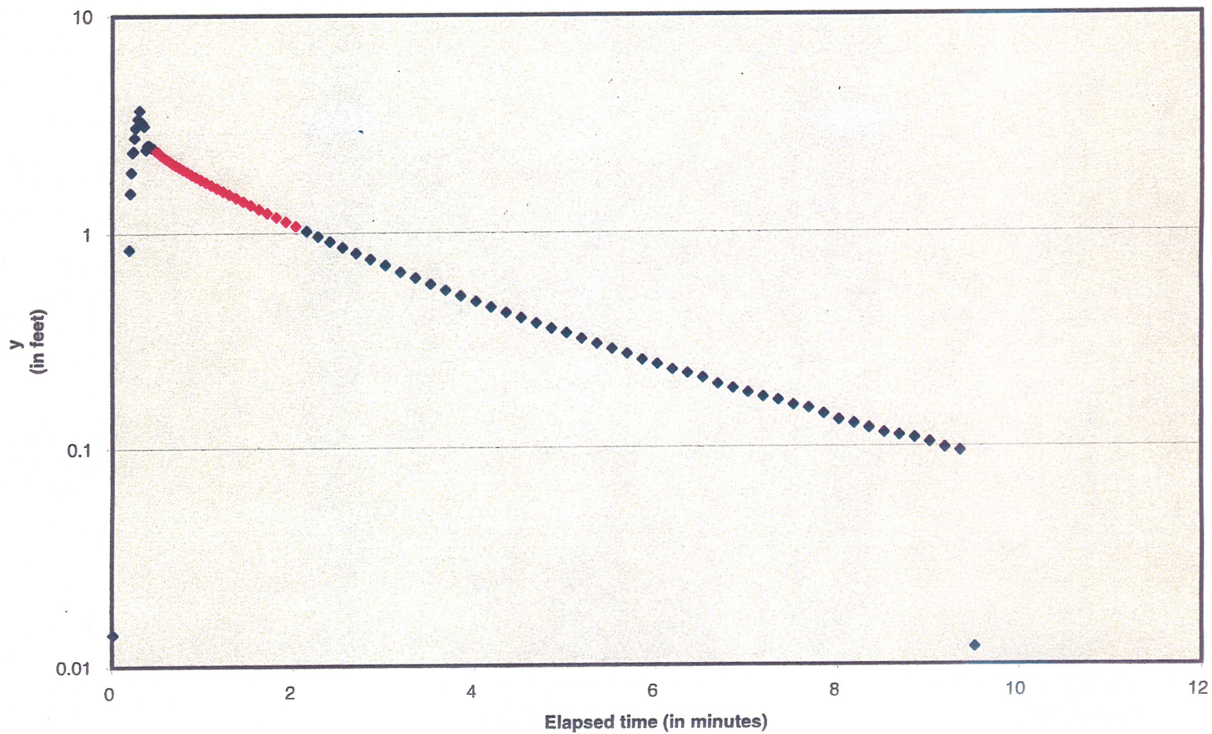
OW-947 (slug-in) Recovery vs. Time
