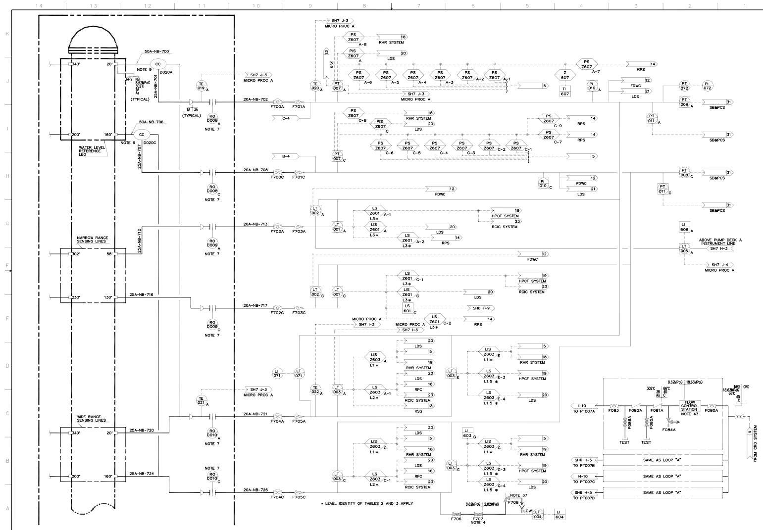
FIGURE 5.1-3 NUCLEAR BOILER SYSTEM P&ID (Sheet 5 of 11) ABWR DCD/Tier 2 Rev.5
