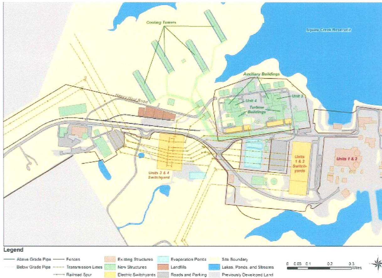
Figure 2.1-201 Site Plot Plan
