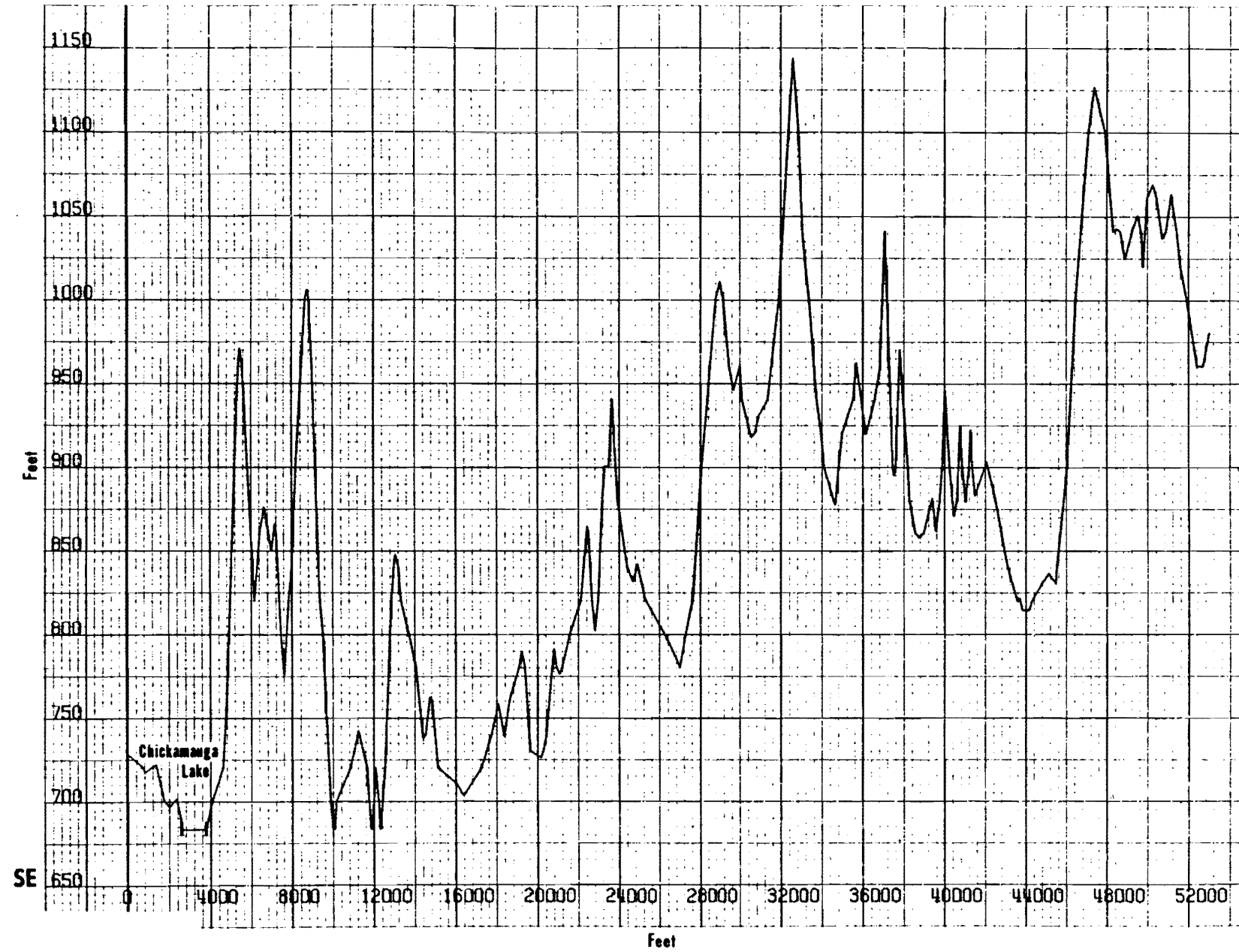
WATTS BAR NUCLEAR PLANT FINAL SAFETY ANALYSIS REPORT TOPOGRAPHY WITHIN 10 MILE RADIUS Figure 2.3-20
