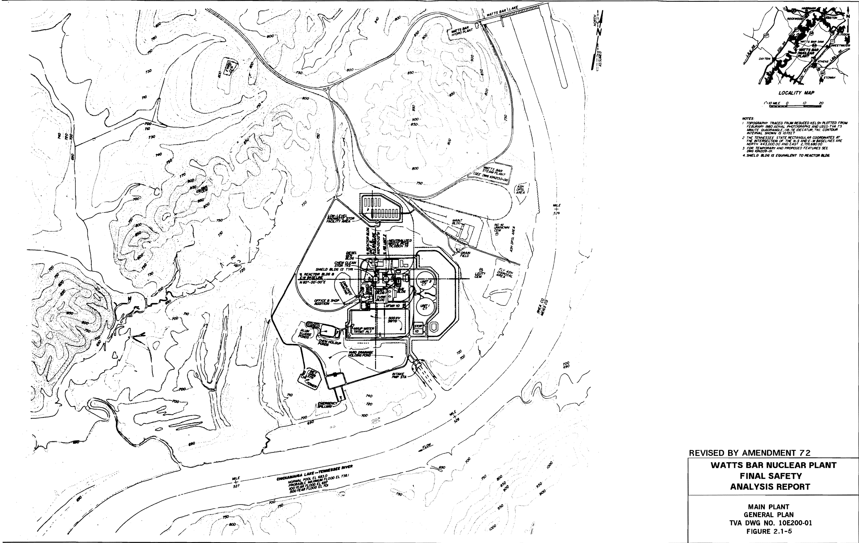
Figure 2.1-5 Main Plant General Plan
