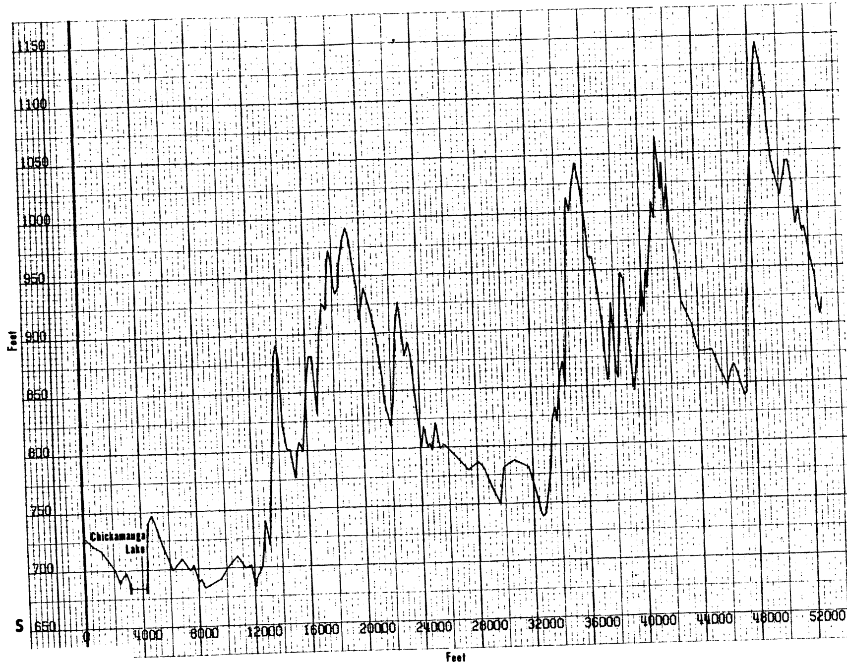
WATTS BAR NUCLEAR PLANT FINAL SAFETY ANALYSIS REPORT TOPOGRAPHY WITHIN 10 MILE RADIUS Figure 2.3-22
