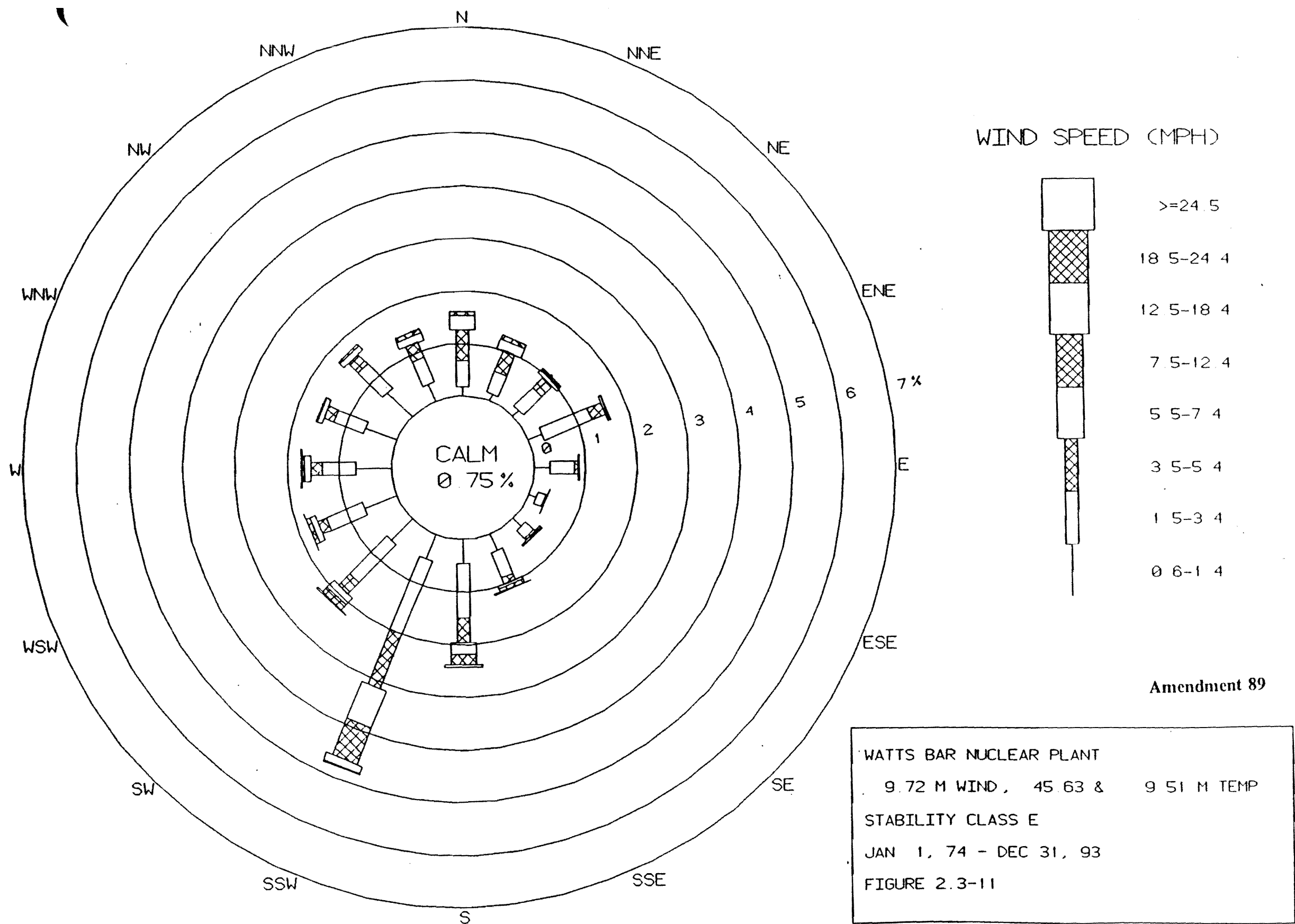
Figure 2.3-11 Wind Speed at 9.72 Meters for Stability Class E, Watts Bar Nuclear Plant, January 1, 1974 -December 31, 1993
