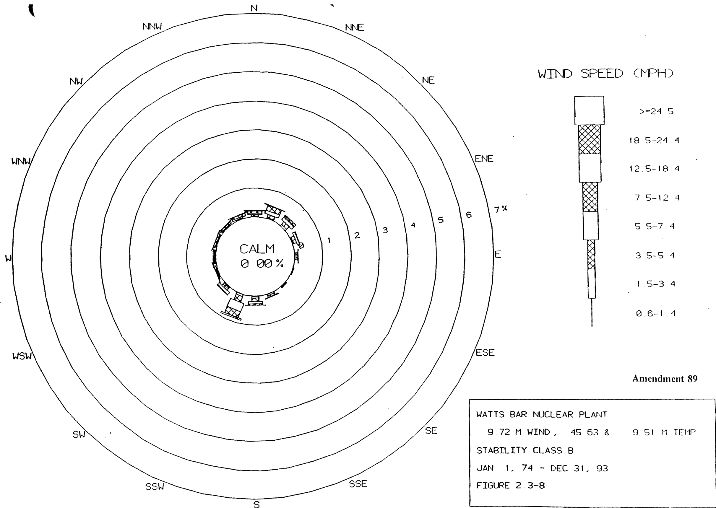
Figure 2.3-8 Wind Speed at 9.72 Meters for Stability Class B, Watts Bar Nuclear Plant, January 1, 1974 - December 31, 1993
