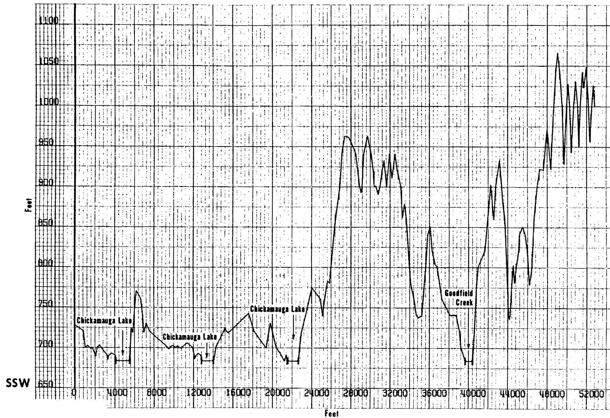
WATTS BAR NUCLEAR PLANT FINAL SAFETY ANALYSIS REPORT TOPOGRAPHY WITHIN 10 MILE RADIUS Figure 2.3-23
