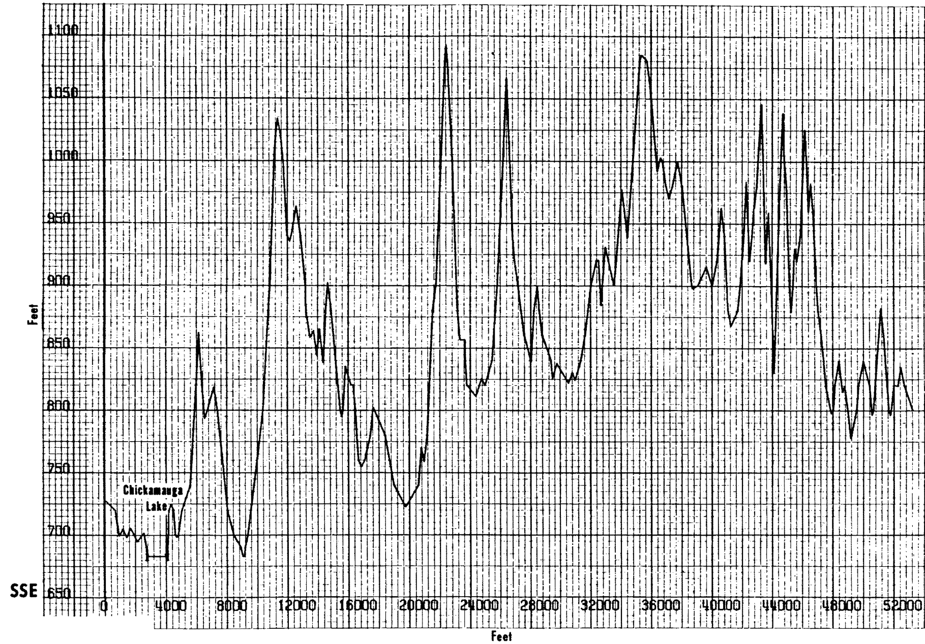
WATTS BAR NUCLEAR PLANT FINAL SAFETY ANALYSIS REPORT TOPOGRAPHY WITHIN 10 MILE RADIUS Figure 2.3-21
