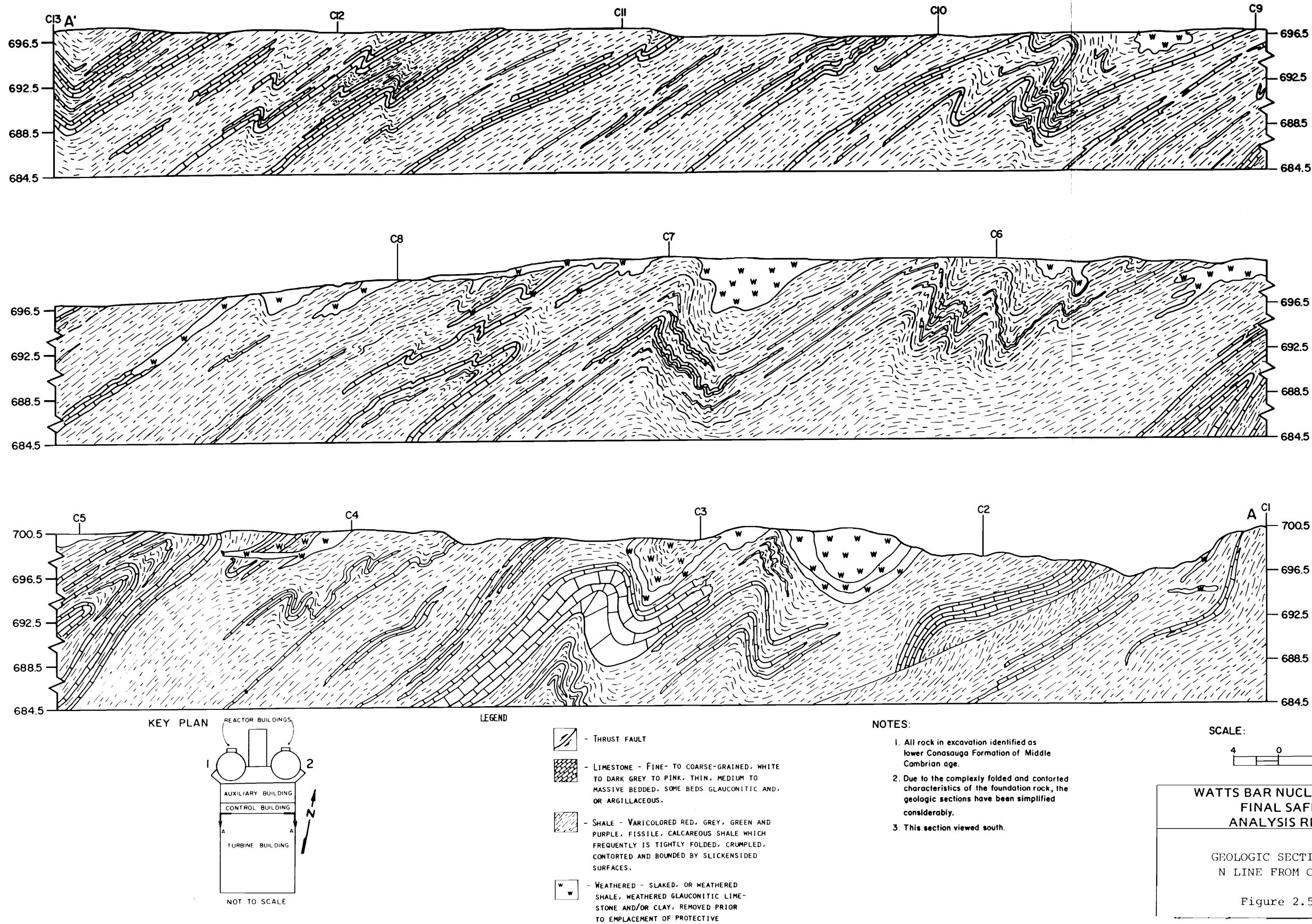
Figure 2.5-113 Geologic Section Along N Line From C1 To C13
