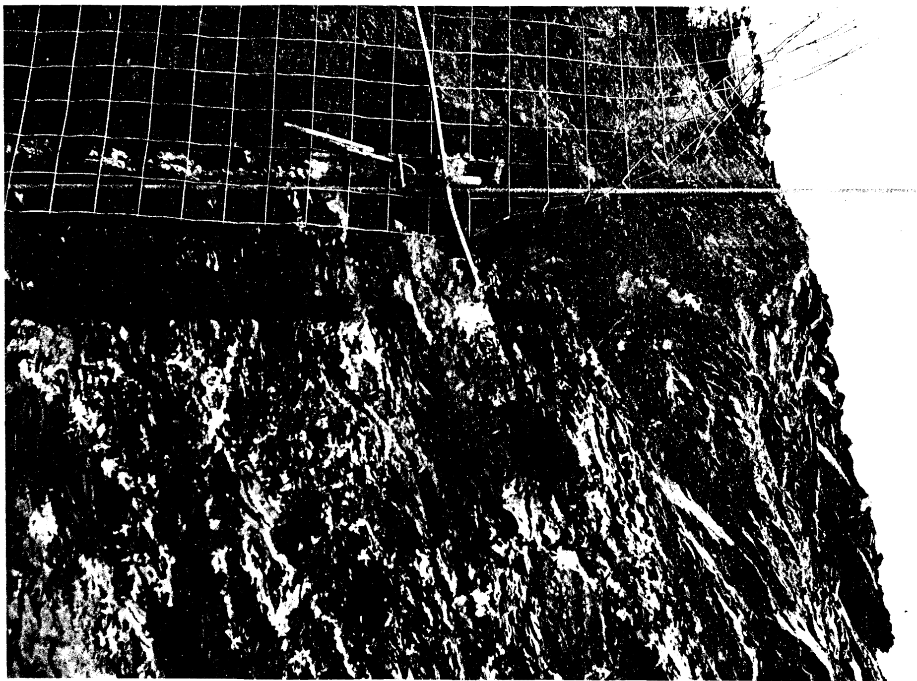
Watts Bar Nuclear Plant Tennessee Valley Authority 88906-H December 13, 1973 Gary W. Krantz, Knoxville Fault in Auxiliary Building Wall, approximately 9 feet west of A5 and 6 feet south of east-west reactor centerline. Fault continues across SE perimeter of Reactor #1. Viewed southwest.
