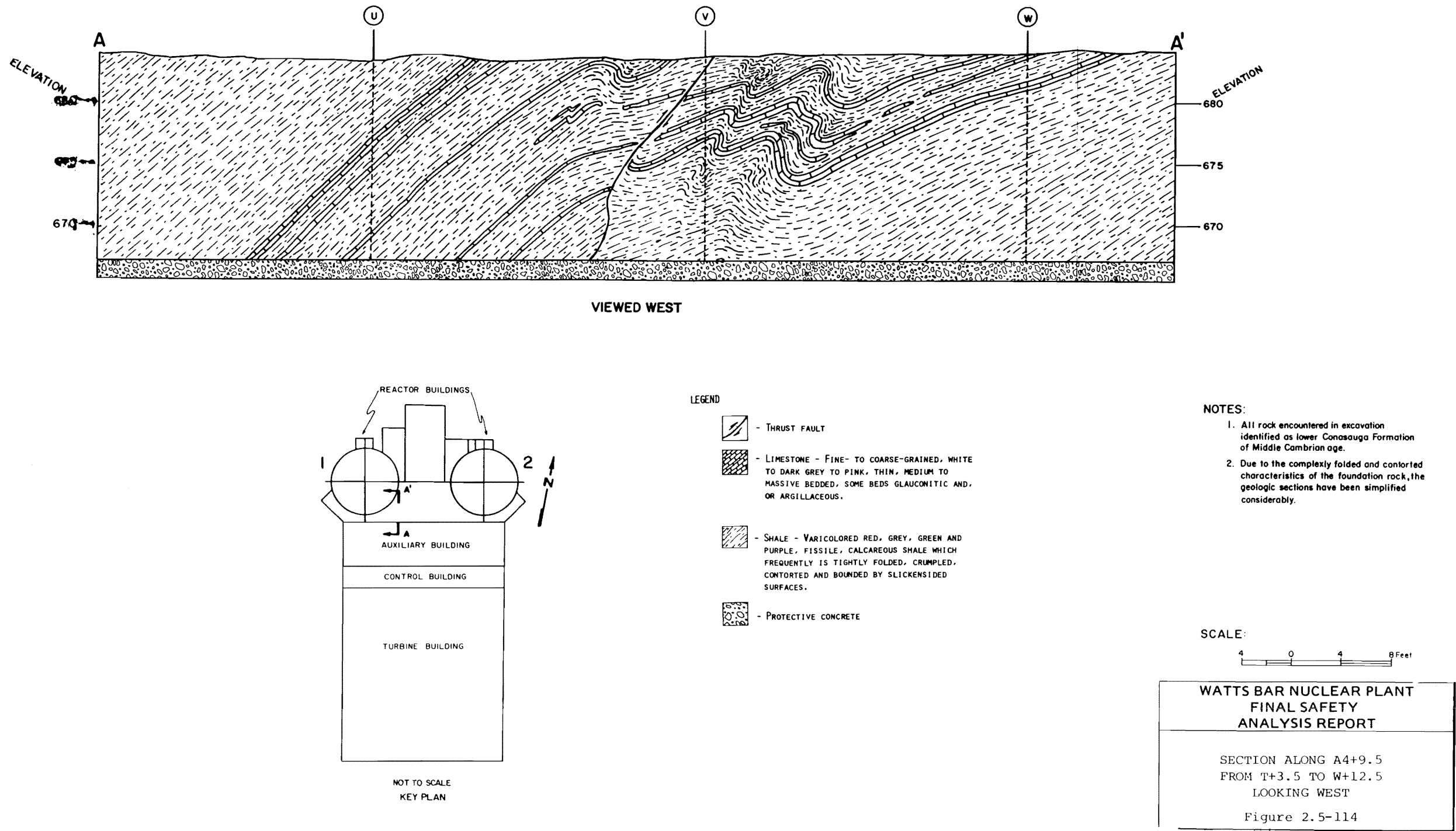
Figure 2.5-114 Section Along A4+9.5 From T+3.5 To W+12.5
