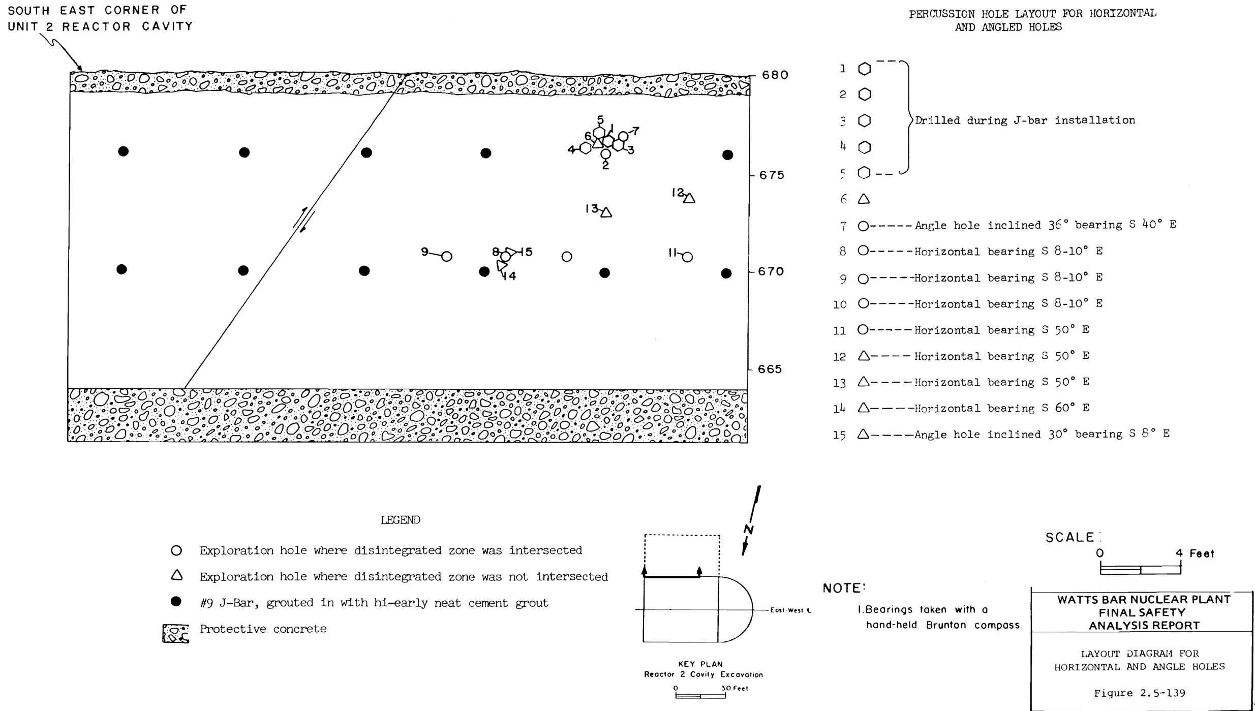
Figure 2.5-139 Layout Diagram For Horizontal and Angle Holes
