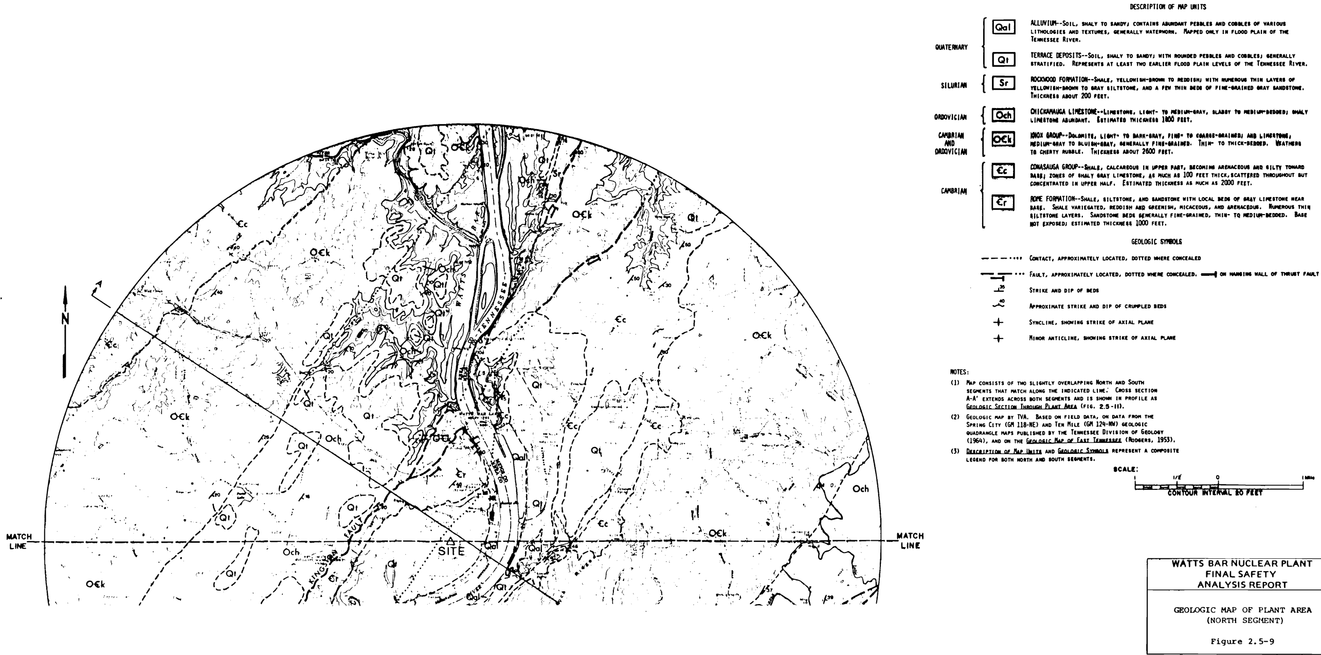
Figure 2.5-9 Geologic Map Of Plant Area (North Segment)
