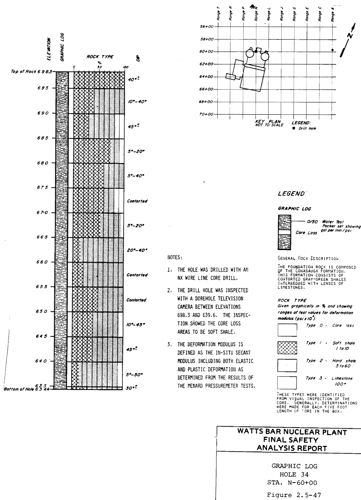
Figure 2.5-47 Graphic Log Hole 34 Sta. N-60+00
