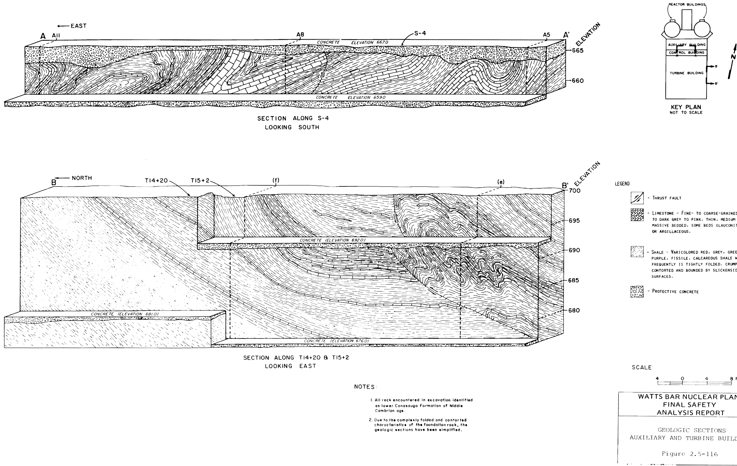
Figure 2.5-116 Geologic Sections Auxiliary And Turbine Buildings
