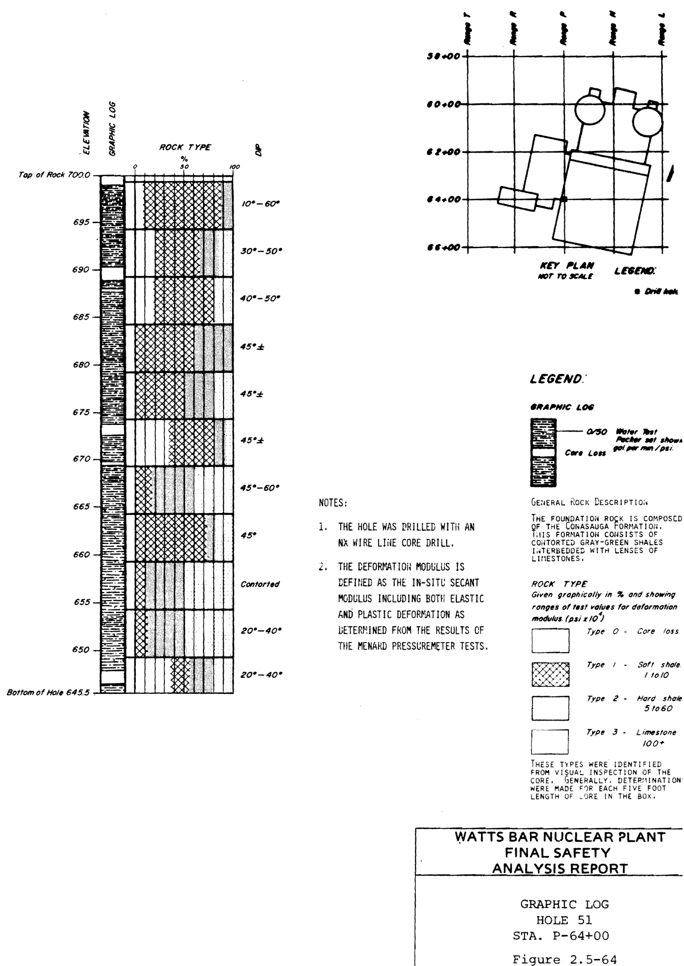
Figure 2.5-64 Graphic Log Hole 51 Sta. P-64+00
