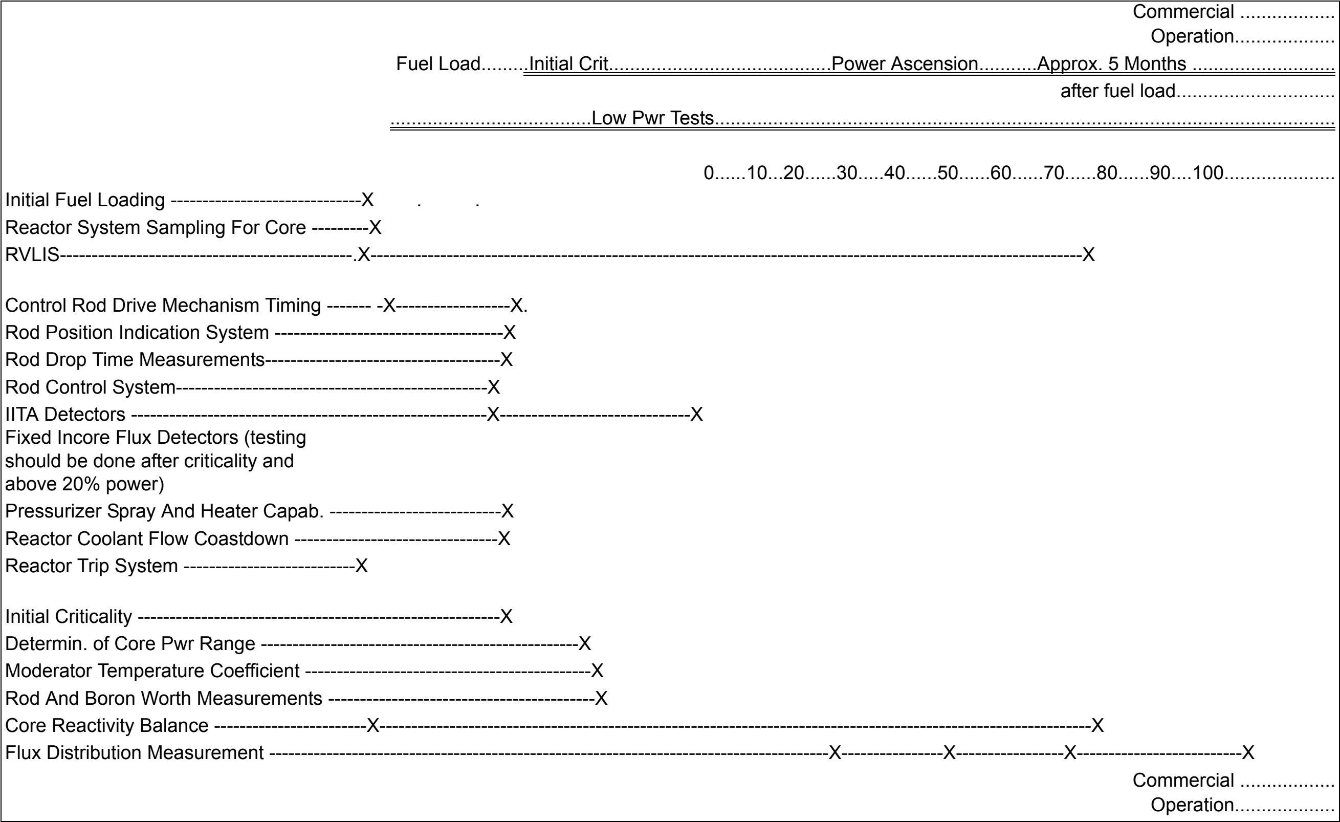
(Page 1 of 2) Figure 14.2-2 Power Ascension Test Schedule
