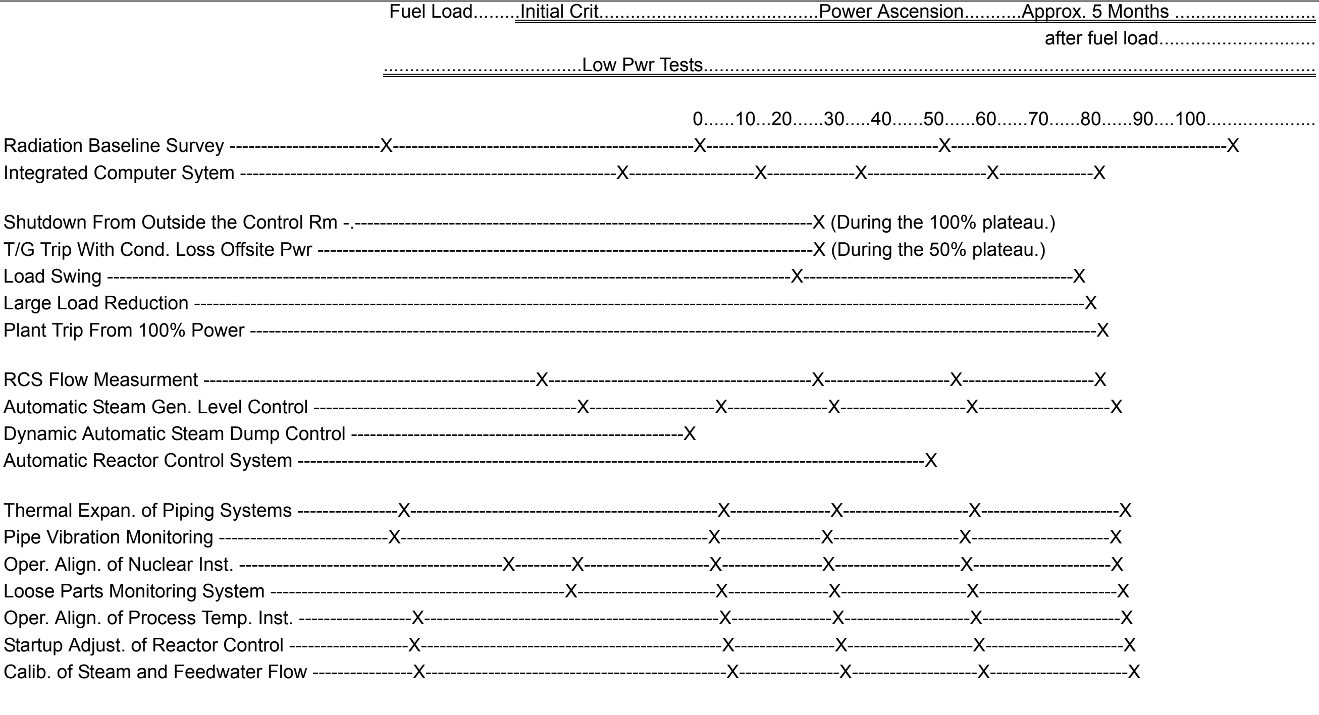
(Continued) (Page 2 of 2) Figure 14.2-2 Power Ascension Test Schedule
