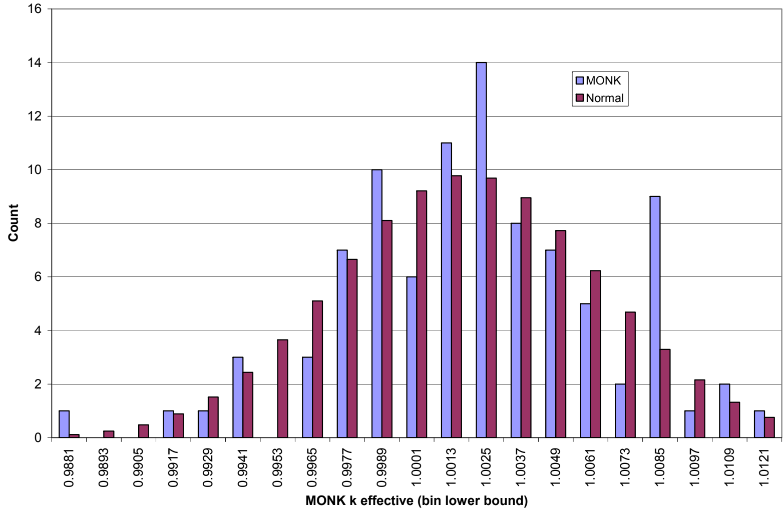
Figure 6-1: MONK8A k_{\text{eff}} Histogram
