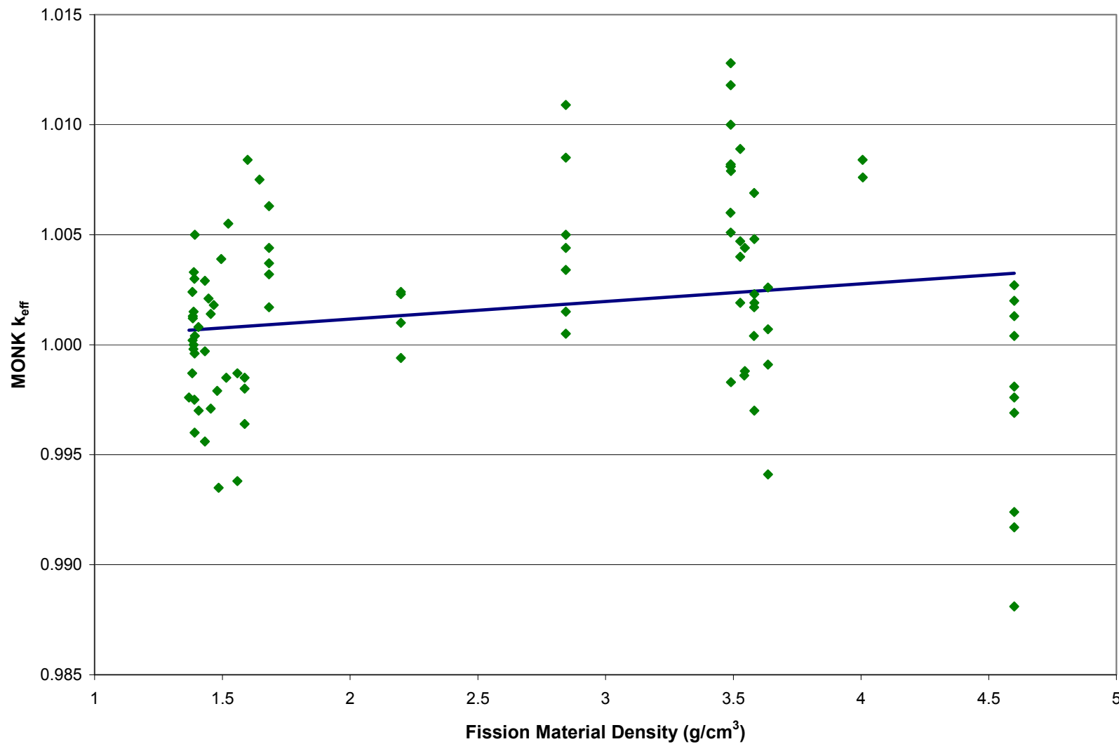
Figure 6-2: Plot of MONK8A k_{\text{eff}} vs. Fission Material Density [ g/cm 3 ]
