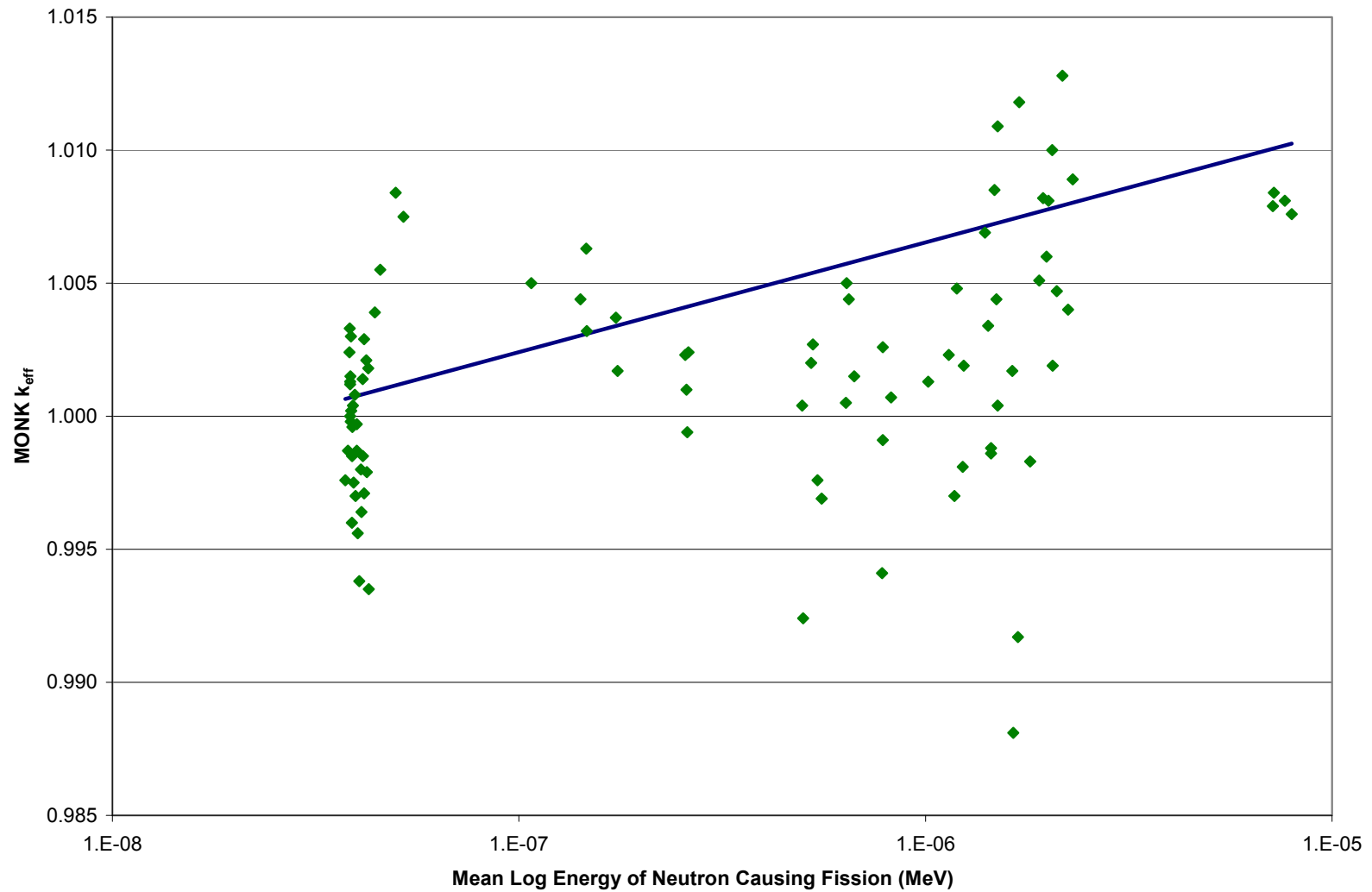
Figure 6-6: Plot of MONK8A k_{\text{eff}} vs. Mean Log Energy of Neutron Causing Fission (MLENCF)
