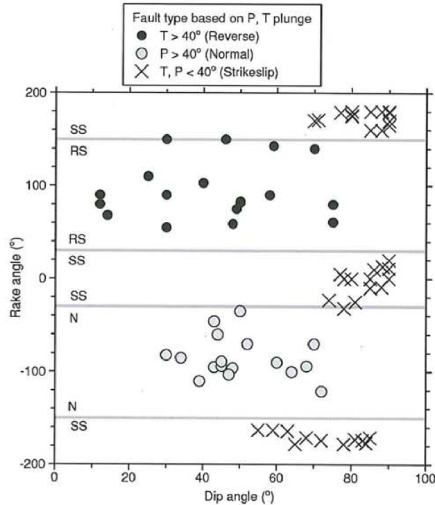
Figure 1. Distribution of the data we used in rake-angle and dip-angle space. The horizontal gray lines indicate boundaries between fault types used by BJS97, and the symbols and colors indicate our classification based on the plunges of the P - and T -axes (our classification scheme is indicated in the legend; see Appendix D in BA07).
