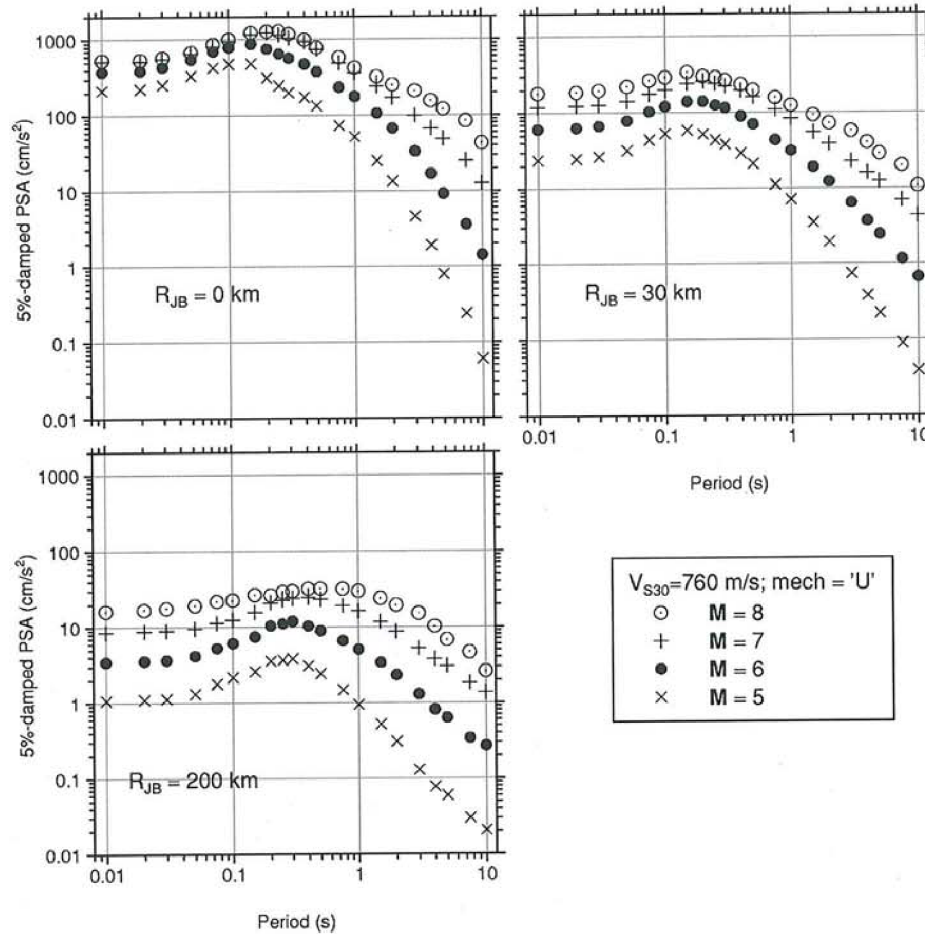
Figure 10. PSA from our equations, as function of period. The spectra are shown for three distances and four magnitudes, for fault type unspecified and V_{S30} = 760 \text{ m/s} .
