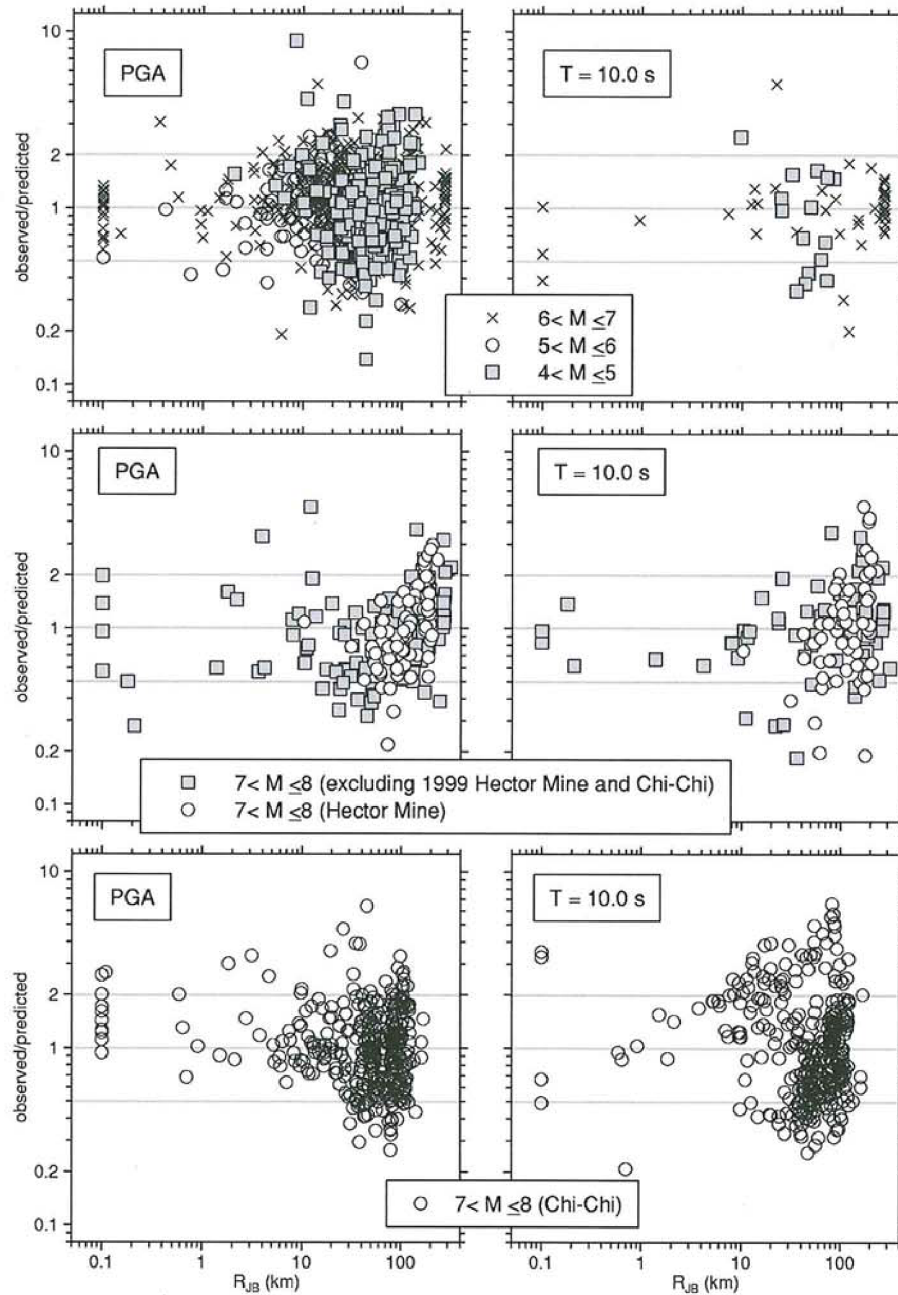
Figure 7. Stage 1 residuals, separated by magnitude, for PGA and T = 10 s PSA (these span the range of possibilities; see BA07 for more plots). The residuals for the 1999 Chi-Chi earthquake are shown separately, in the bottom two graphs.
