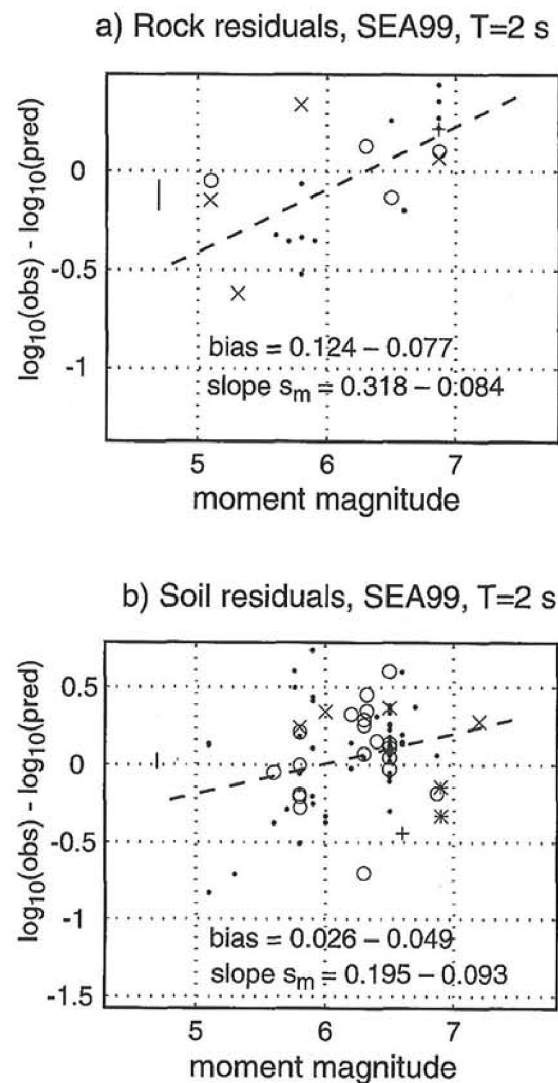
Figure 6. Dependence of SEA99 residuals on moment magnitude for a 2.0-sec period. Dashed line is maximum likelihood fit to points. Short vertical bar at M = 4.7 is mean bias \pm standard error of mean. Symbol type indicates distance r_{jb} : dot, 0–20 km; circle, 20–40 km; x, 40–60 km; +, 60–80 km; *, r_{jb} > 80 km. (a) Rock residuals. (b) Soil residuals.
