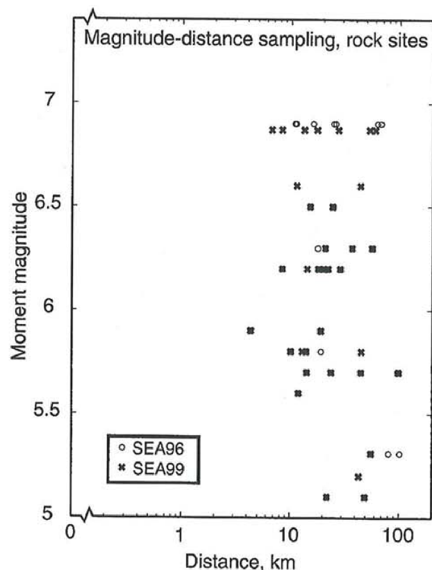
Figure 2. Magnitude-distance sampling for SEA99 ( \times symbols) and SEA96 (circles) for rock sites.
