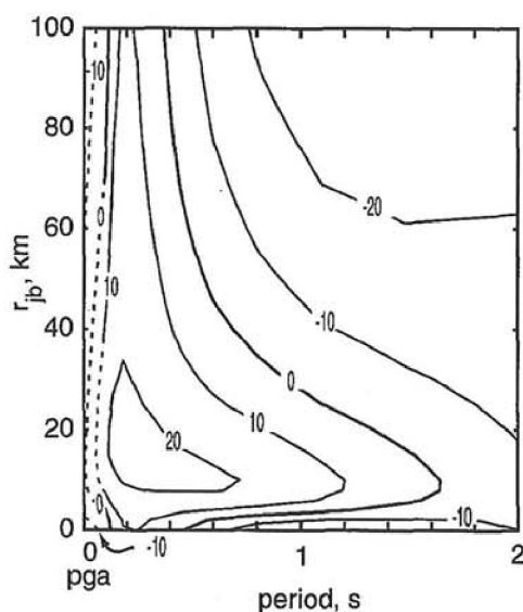
b) (\text{SEA99} / \text{SEA96} - 1) \times 100 (soil)
