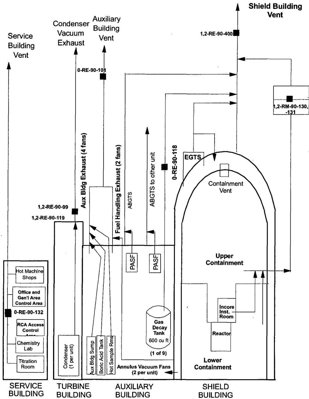
Figure 7.1 GASEOUS EFFLUENT RELEASE POINTS
