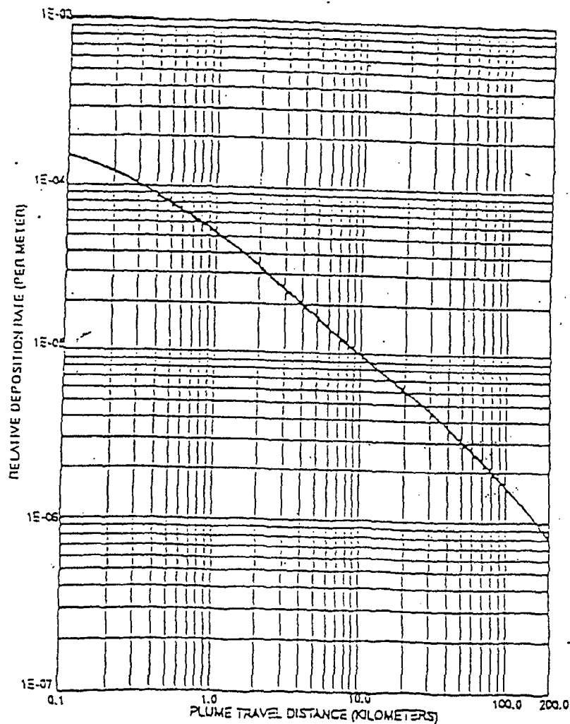
Figure 7.6 RELATIVE DEPOSITION FOR GROUND LEVEL RELEASES (All Stability Classes)
