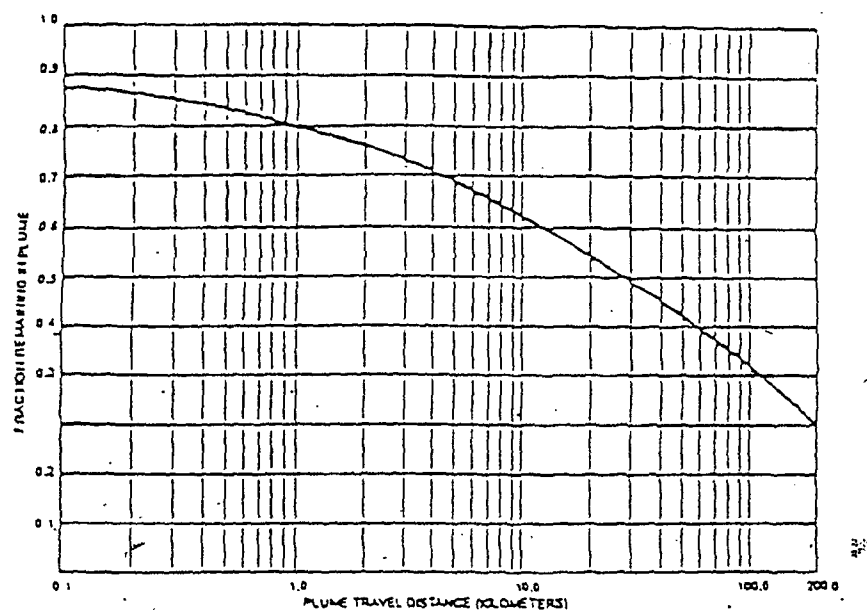
Figure 7.4 PLUME DEPLETION EFFECT FOR GROUND LEVEL RELEASES (All Stability Classes)
