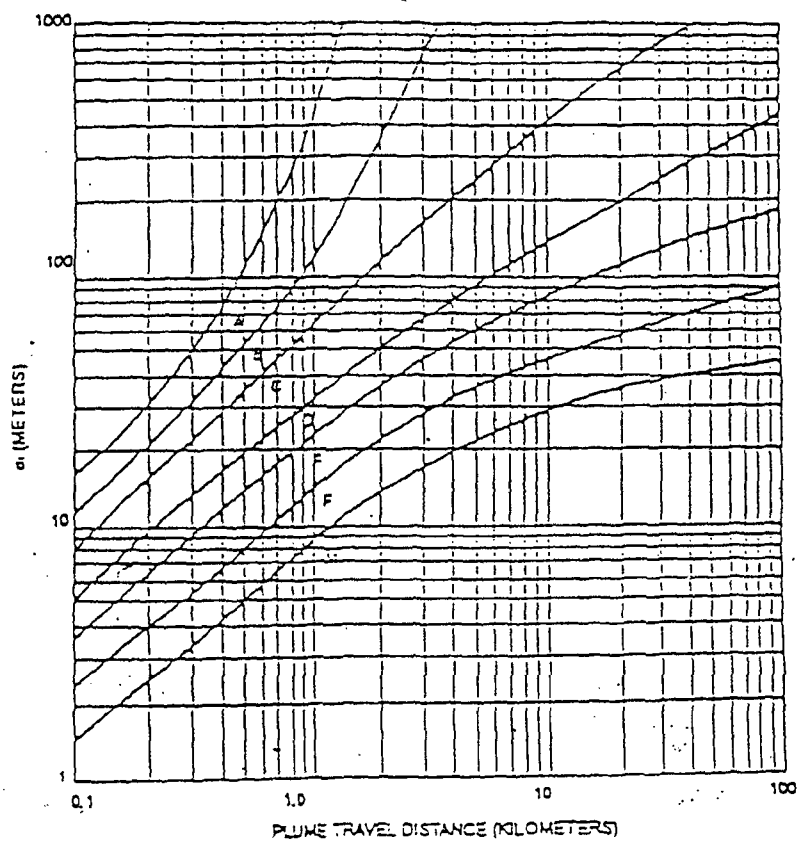
Figure 7.5 VERTICAL STANDARD DEVIATION OF MATERIAL IN A PLUME
