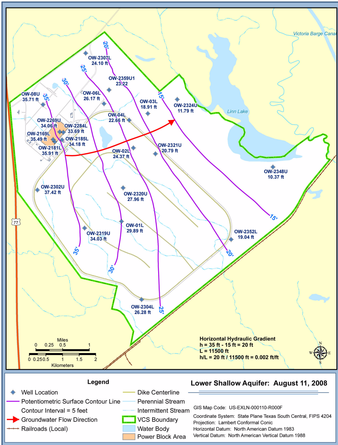
Figure 2.4.12-15 Potentiometric Surface Maps (Sheet 8 of 21)
