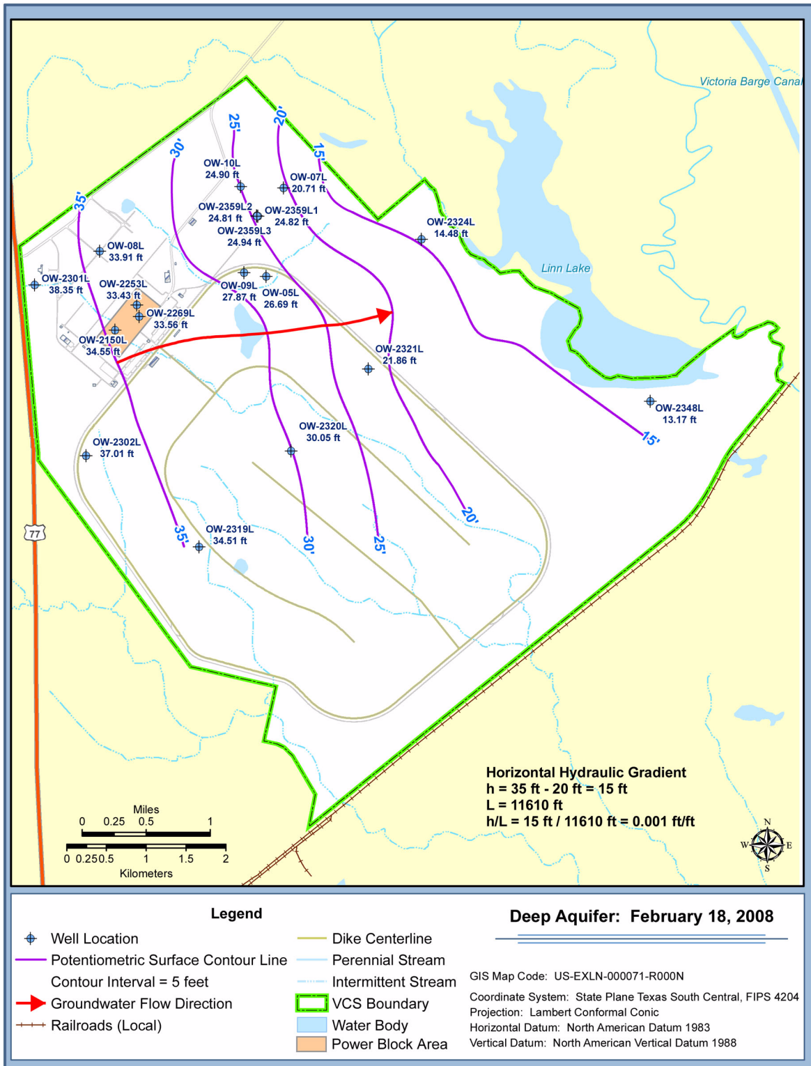
Figure 2.4.12-15 Potentiometric Surface Maps (Sheet 3 of 21)
