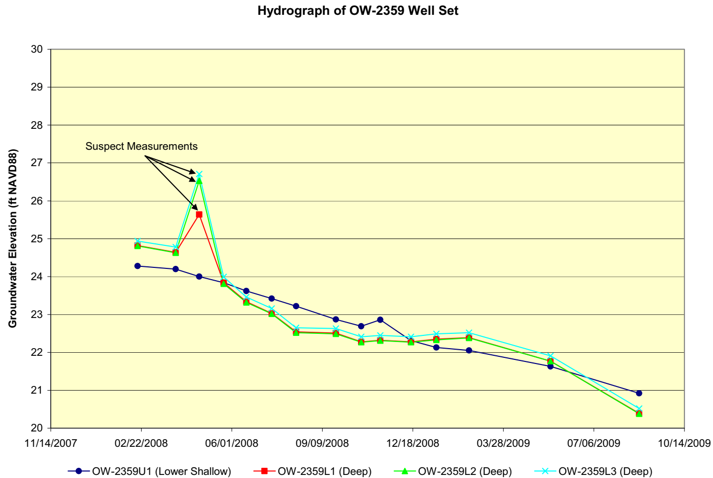
Figure 2.4.12-17 VCS Site Hydrographs; OW-2359U/L Well Set (Sheet 28 of 28)
