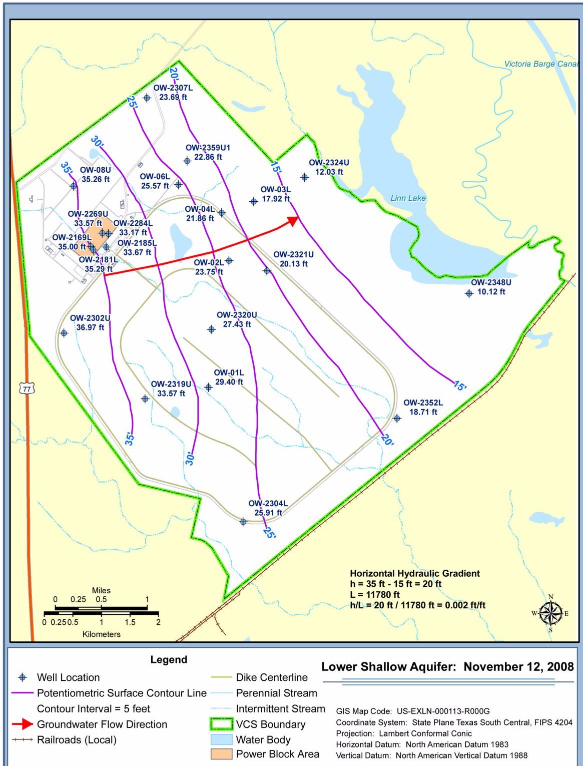
Figure 2.4.12-15 Potentiometric Surface Maps (Sheet 11 of 21)
