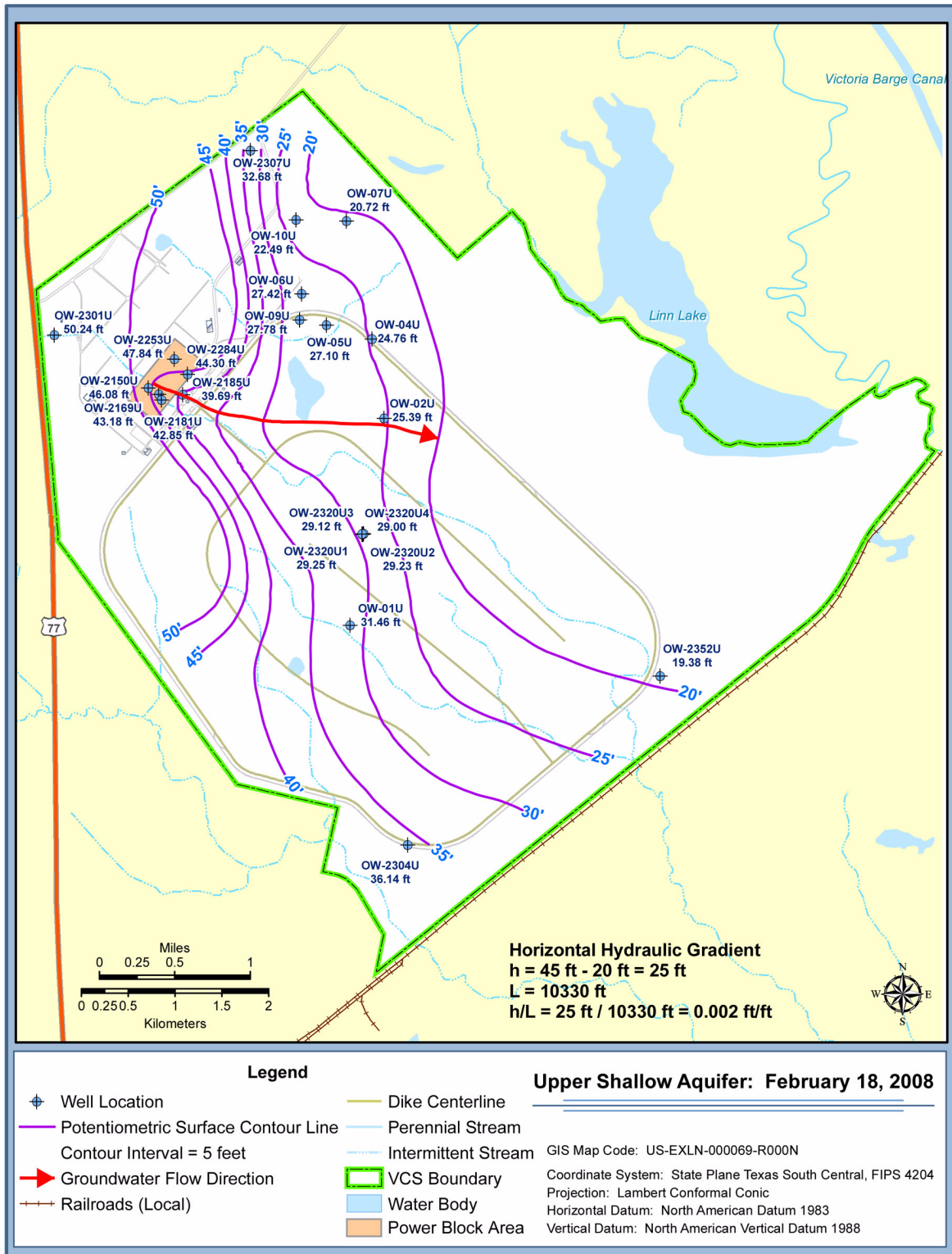
Figure 2.4.12-15 Potentiometric Surface Maps (Sheet 1 of 21)
