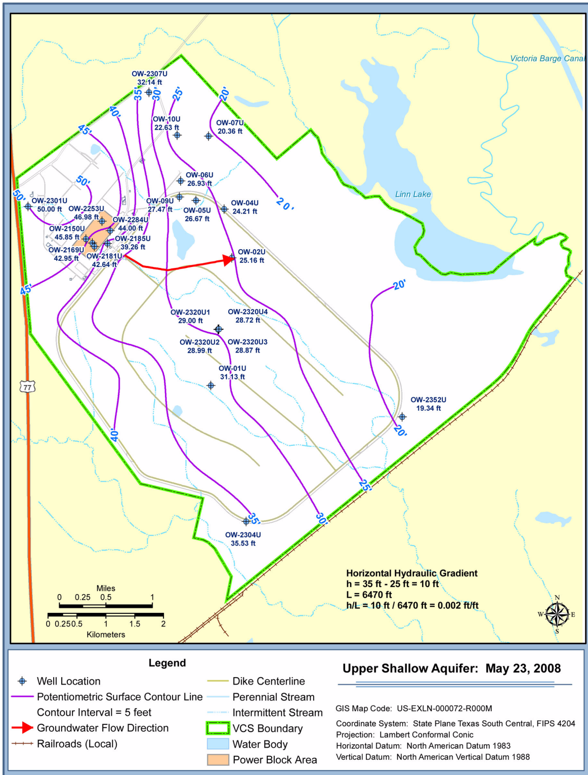
Figure 2.4.12-15 Potentiometric Surface Maps (Sheet 4 of 21)
