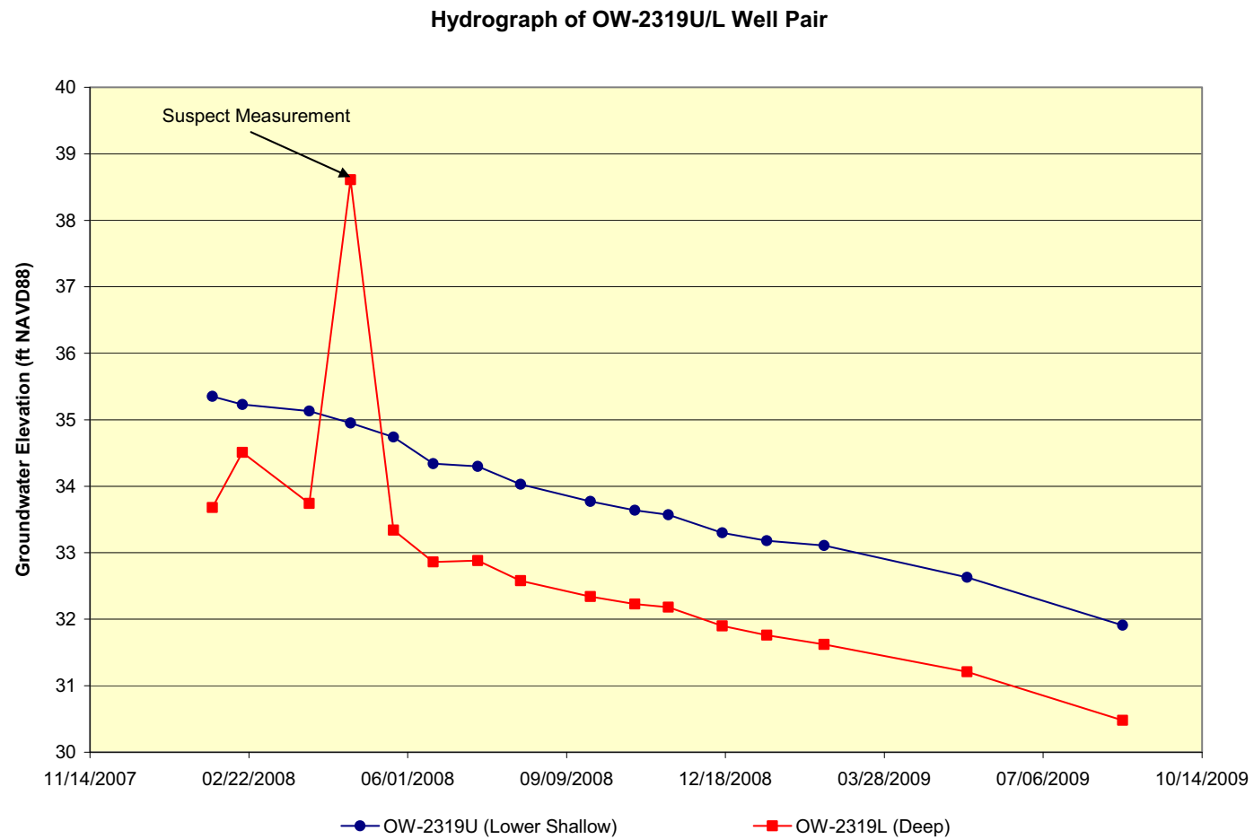
Figure 2.4.12-17 VCS Site Hydrographs; OW-2319U/L Well Pair (Sheet 22 of 28)
