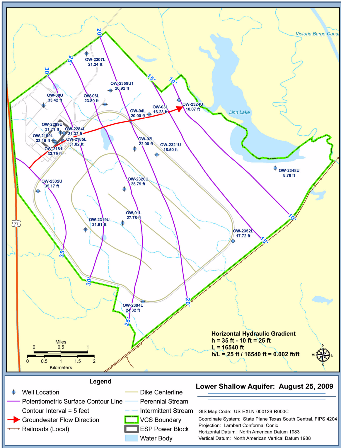
Figure 2.4.12-15 Potentiometric Surface Maps (Sheet 20 of 21)
