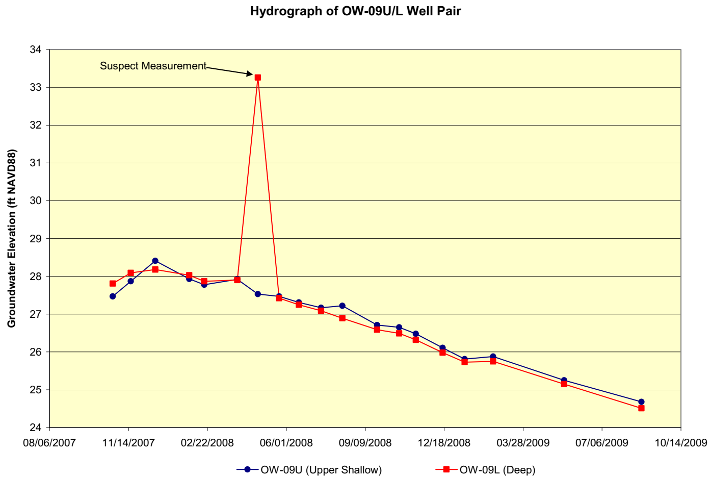
Figure 2.4.12-17 VCS Site Hydrographs; OW-09U/L Well Pair (Sheet 9 of 28)
