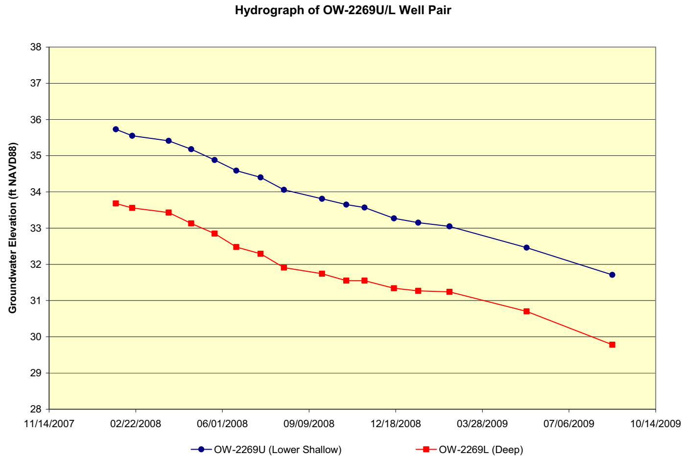
Figure 2.4.12-17 VCS Site Hydrographs; OW-2269U/L Well Pair (Sheet 16 of 28)
