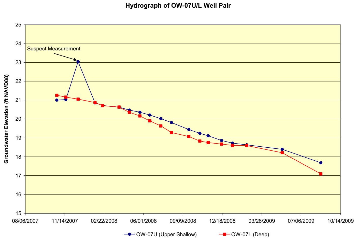
Figure 2.4.12-17 VCS Site Hydrographs; OW-07U/L Well Pair (Sheet 7 of 28)
