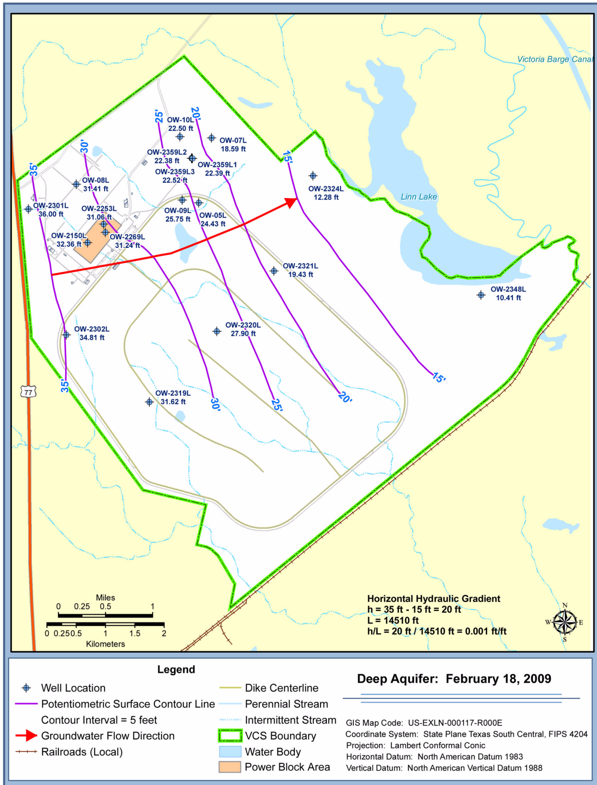
Figure 2.4.12-15 Potentiometric Surface Maps (Sheet 15 of 21)
