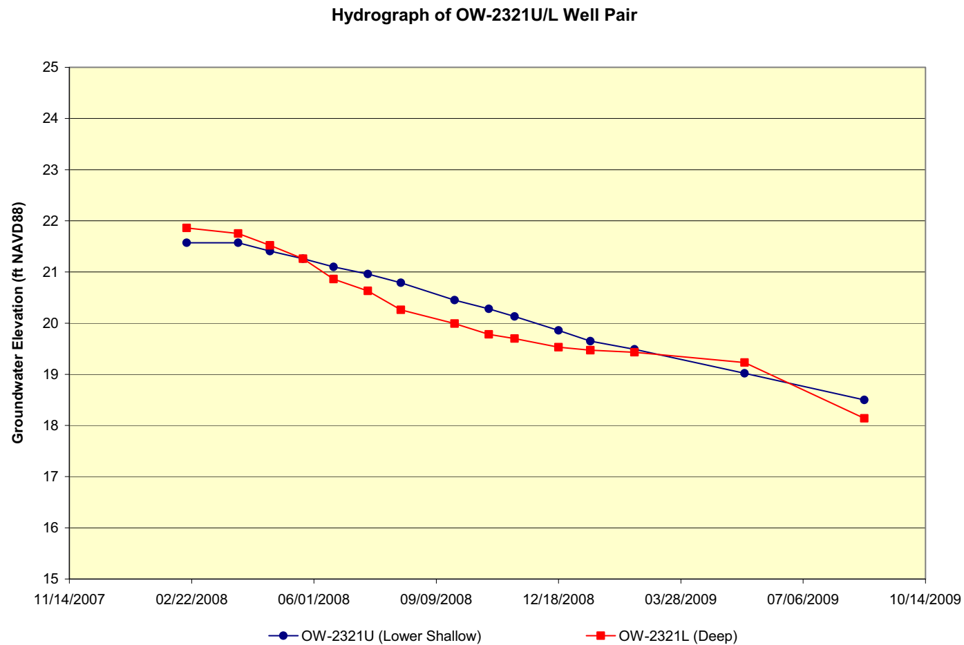
Figure 2.4.12-17 VCS Site Hydrographs; OW-2321U/L Well Pair (Sheet 24 of 28)
