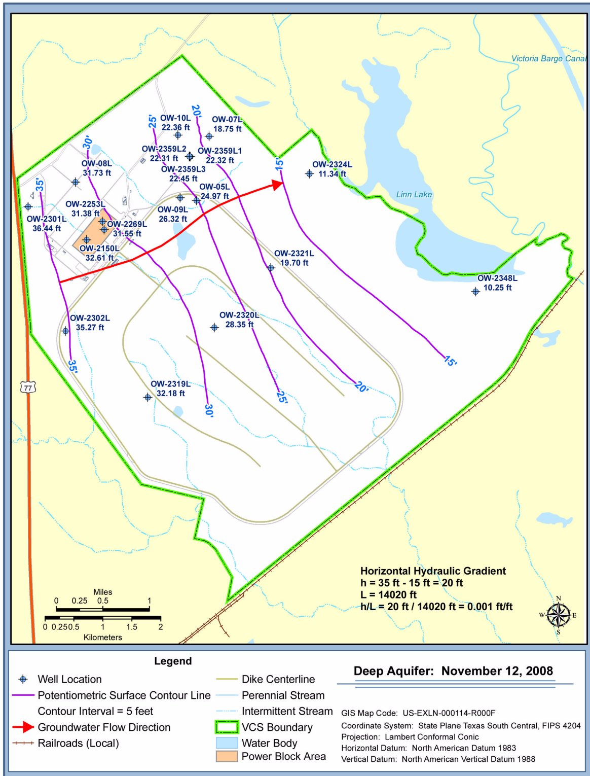
Figure 2.4.12-15 Potentiometric Surface Maps (Sheet 12 of 21)
