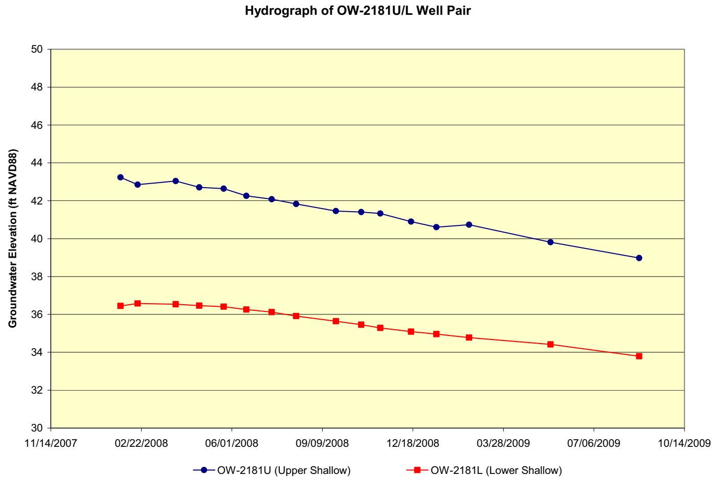
Figure 2.4.12-17 VCS Site Hydrographs; OW-2181U/L Well Pair (Sheet 13 of 28)
