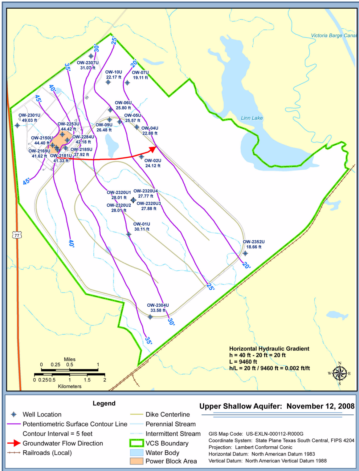
Figure 2.4.12-15 Potentiometric Surface Maps (Sheet 10 of 21)
