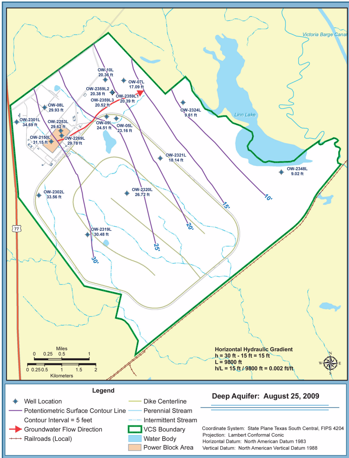
Figure 2.4.12-15 Potentiometric Surface Maps (Sheet 21 of 21)
