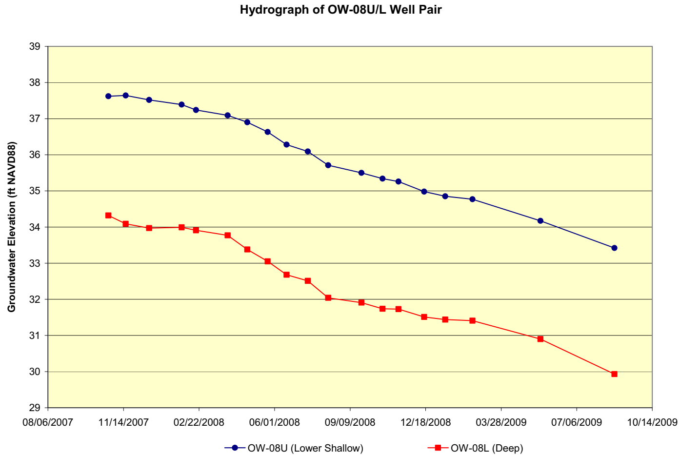
Figure 2.4.12-17 VCS Site Hydrographs; OW-08U/L Well Pair (Sheet 8 of 28)
