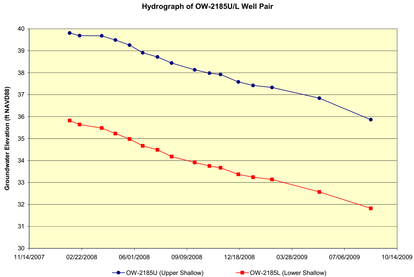
Figure 2.4.12-17 VCS Site Hydrographs; OW-2185U/L Well Pair (Sheet 14 of 28)
