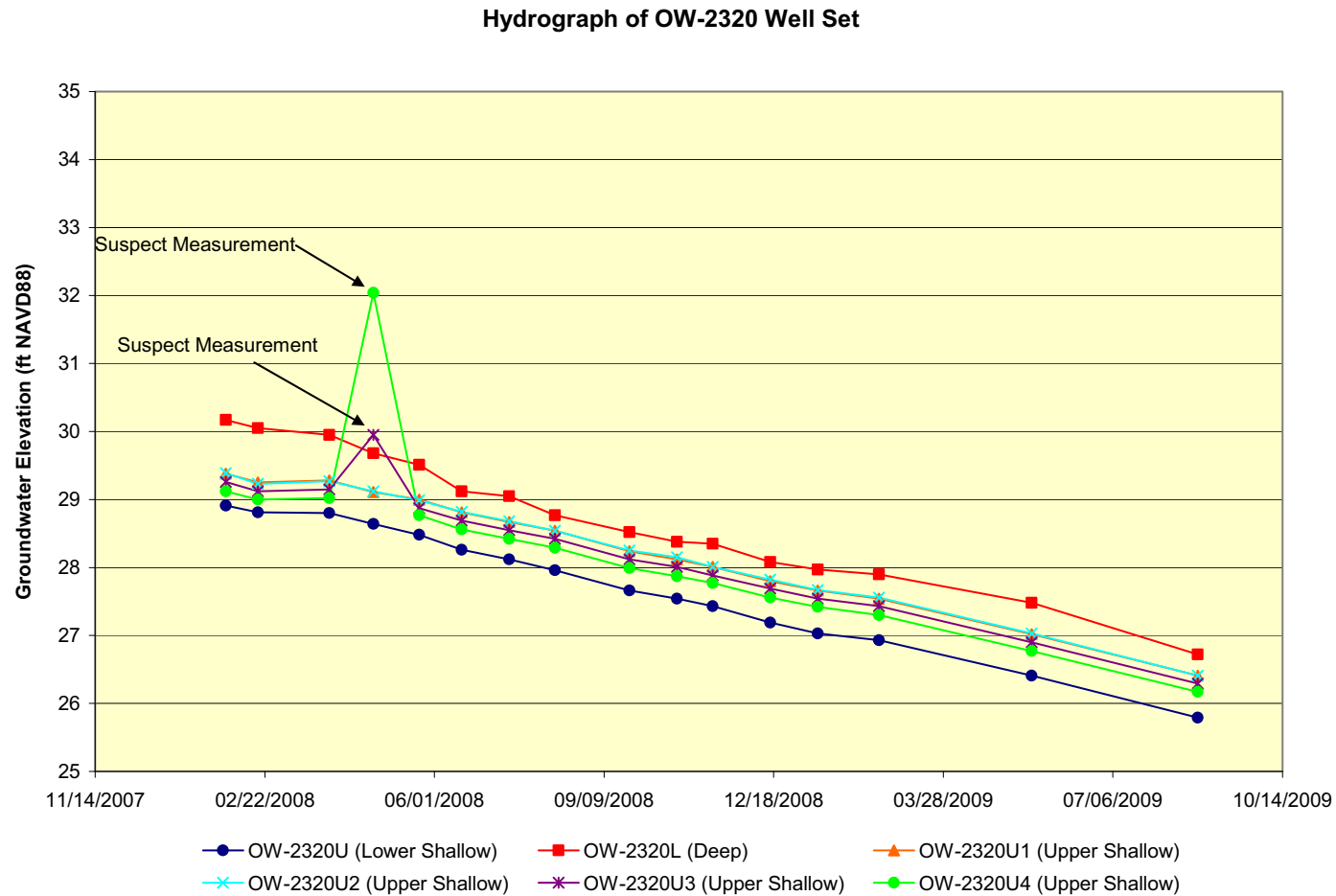
Figure 2.4.12-17 VCS Site Hydrographs; OW-2320U/L Well Set (Sheet 23 of 28)
