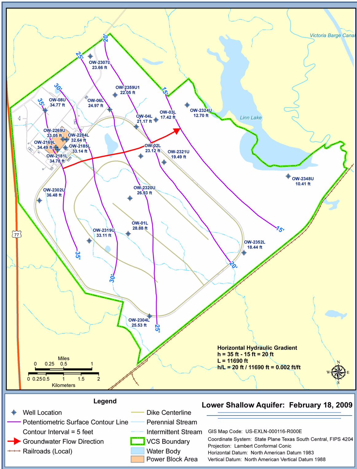
Figure 2.4.12-15 Potentiometric Surface Maps (Sheet 14 of 21)
