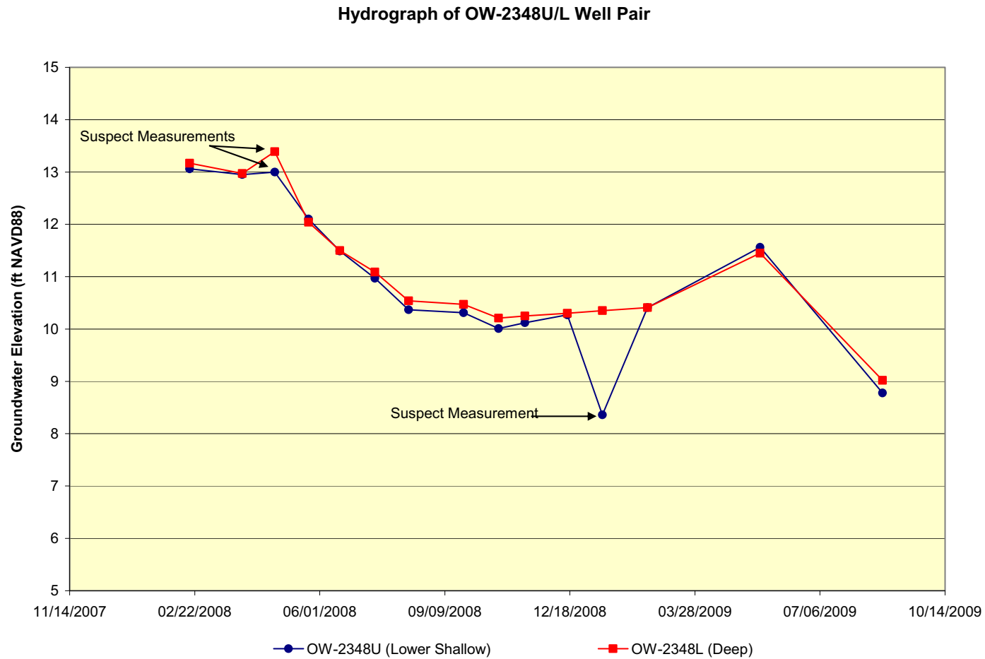
Figure 2.4.12-17 VCS Site Hydrographs; OW-2348U/L Well Pair (Sheet 26 of 28)
