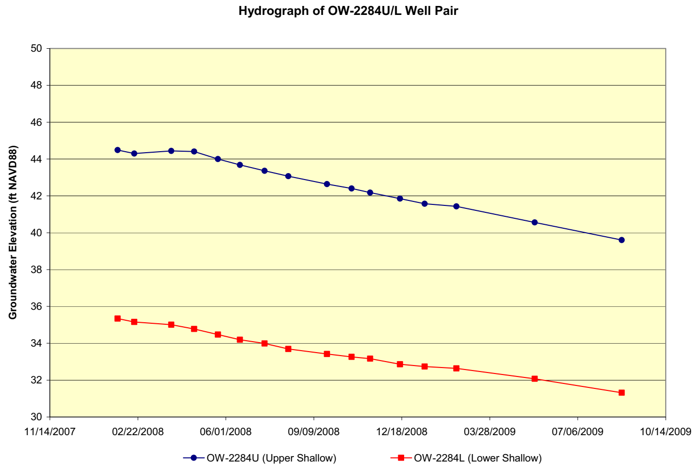
Figure 2.4.12-17 VCS Site Hydrographs; OW-2284U/L Well Pair (Sheet 17 of 28)
