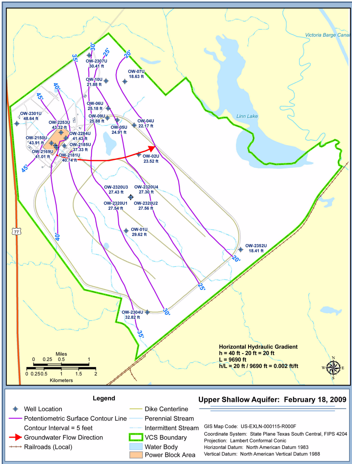
Figure 2.4.12-15 Potentiometric Surface Maps (Sheet 13 of 21)
