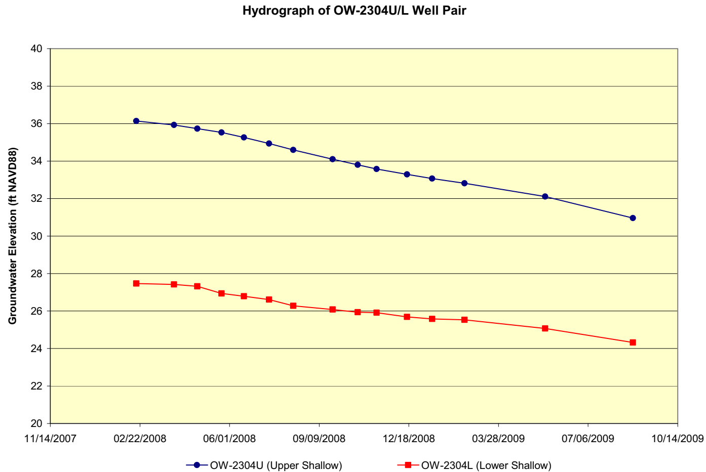
Figure 2.4.12-17 VCS Site Hydrographs; OW-2304U/L Well Pair (Sheet 20 of 28)
