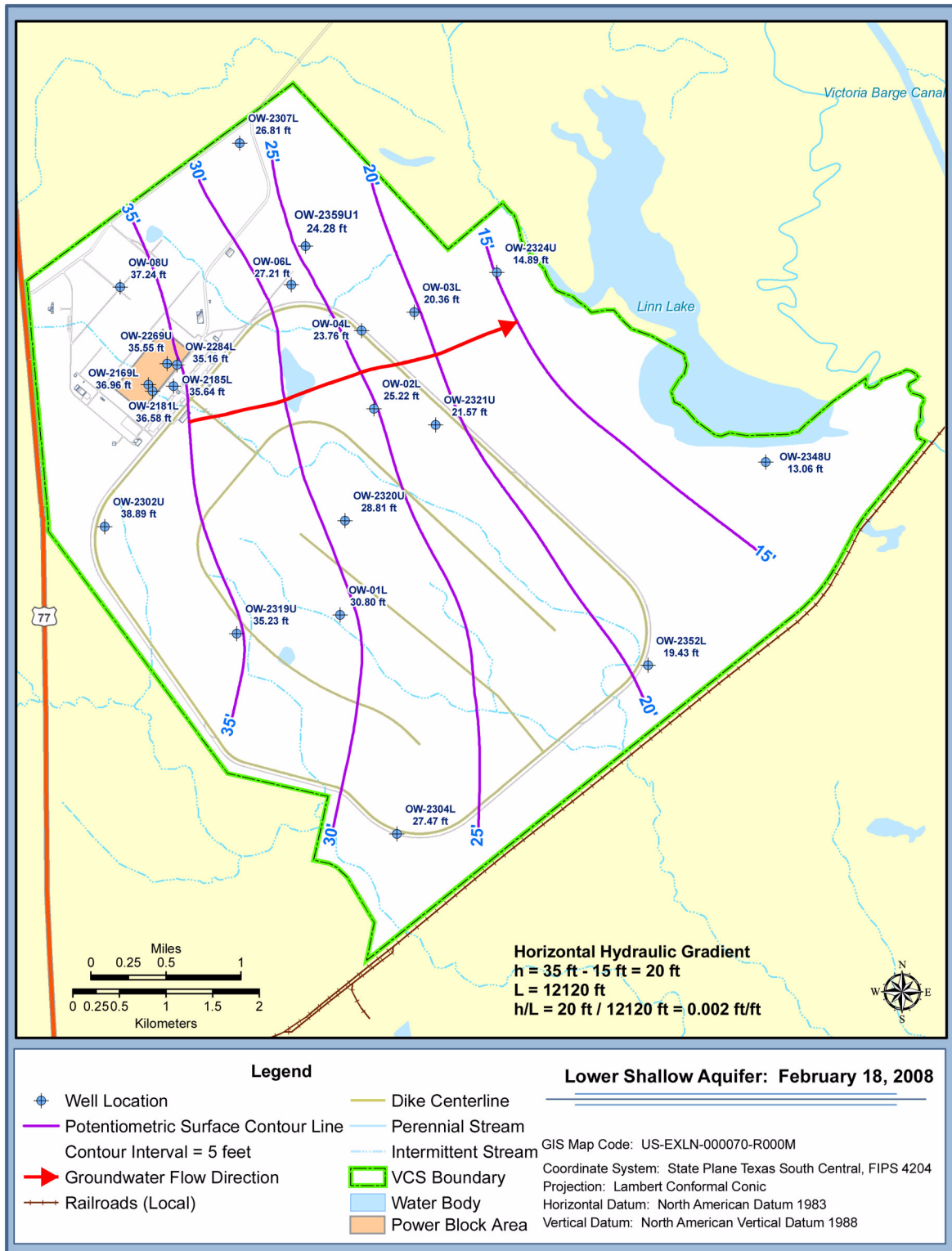
Figure 2.4.12-15 Potentiometric Surface Maps (Sheet 2 of 21)
