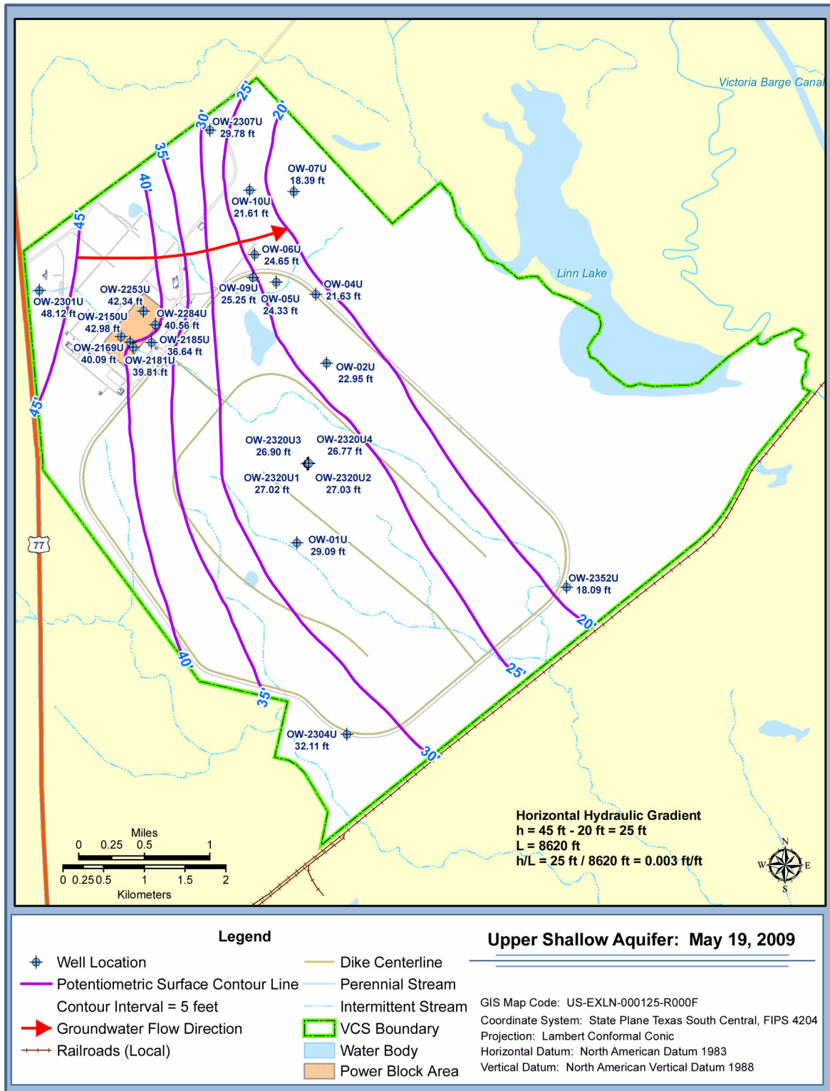
Figure 2.4.12-15 Potentiometric Surface Maps (Sheet 16 of 21)
