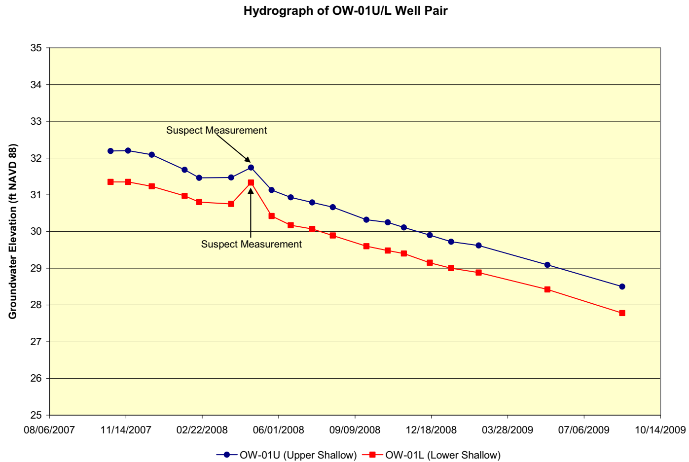
Figure 2.4.12-17 VCS Site Hydrographs; OW-01U/L Well Pair (Sheet 1 of 28)
