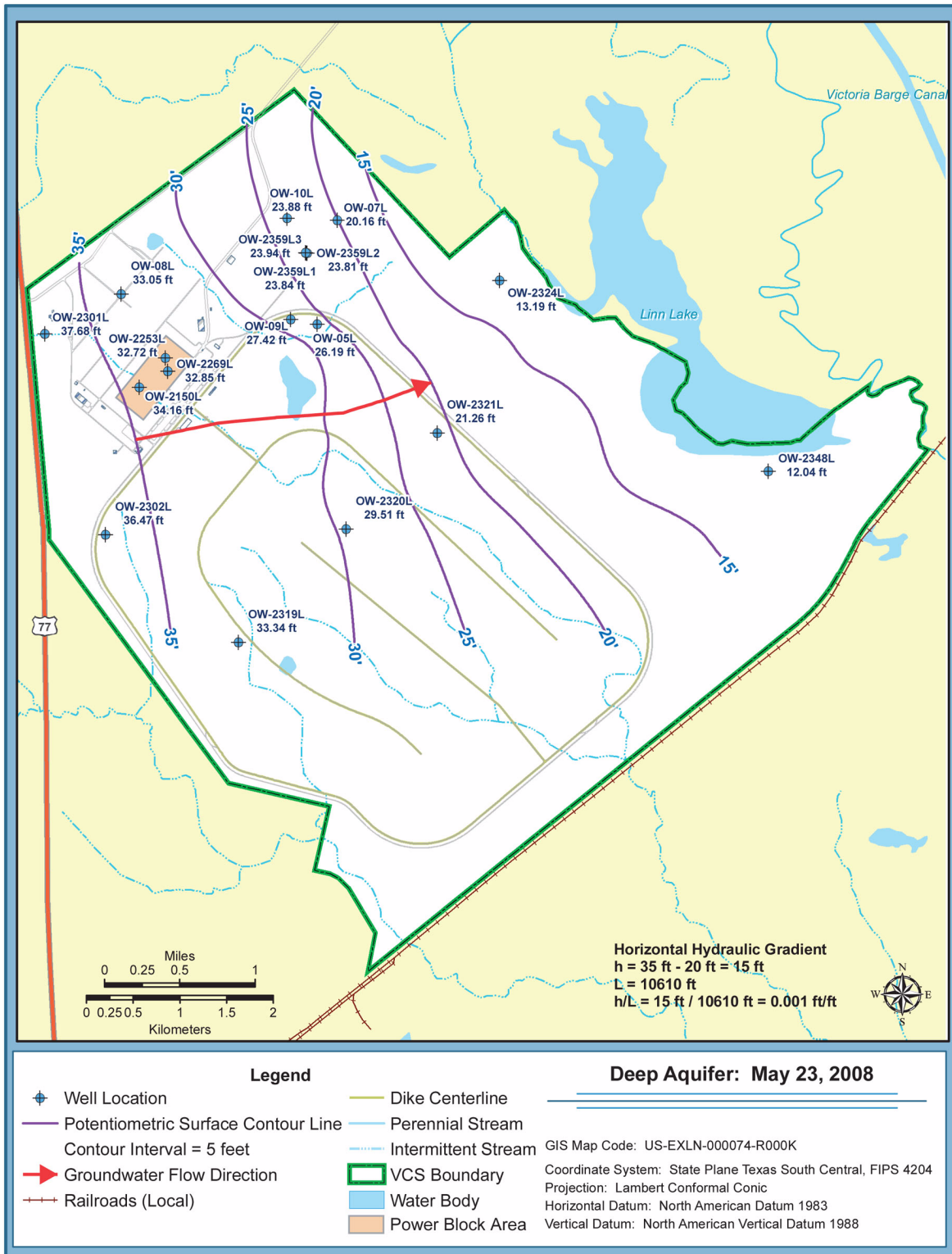
Figure 2.4.12-15 Potentiometric Surface Maps (Sheet 6 of 21)
