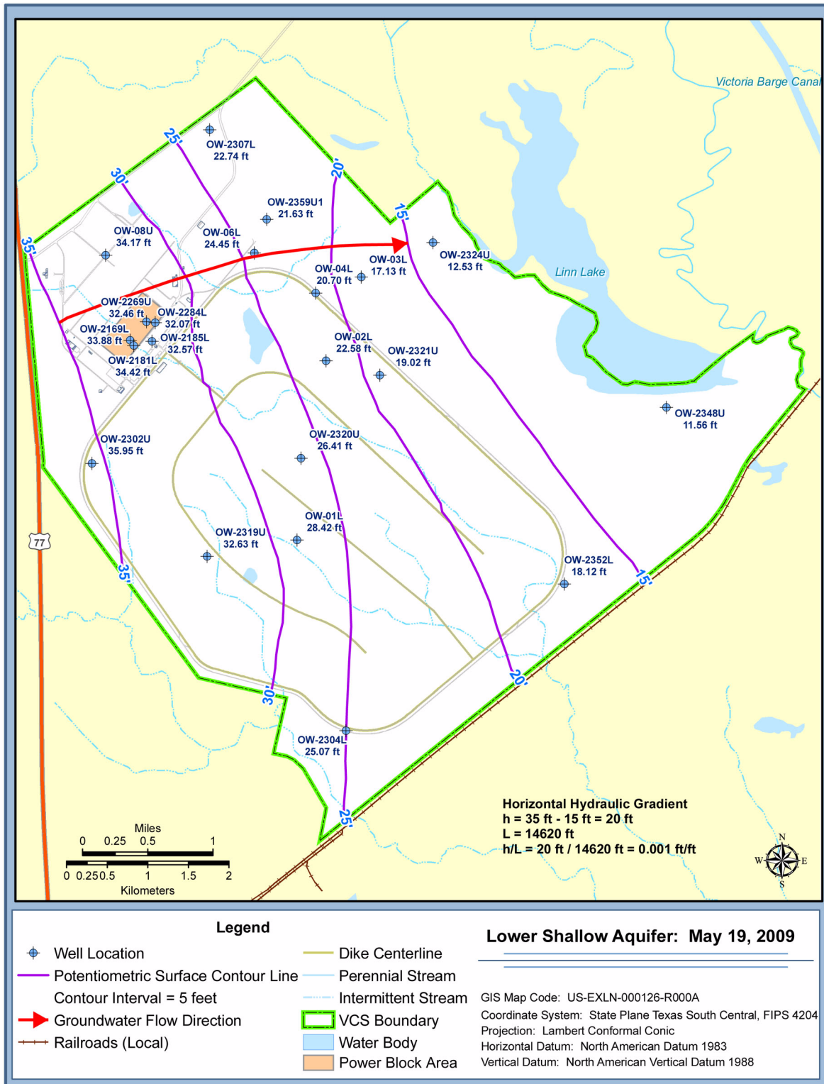
Figure 2.4.12-15 Potentiometric Surface Maps (Sheet 17 of 21)
