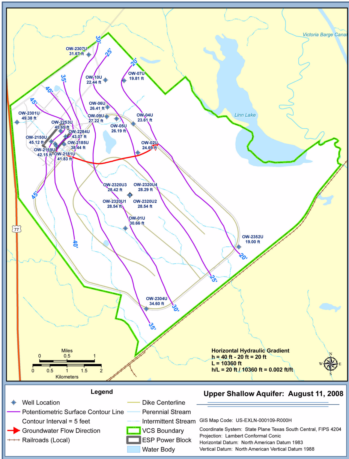
Figure 2.4.12-15 Potentiometric Surface Maps (Sheet 7 of 21)
