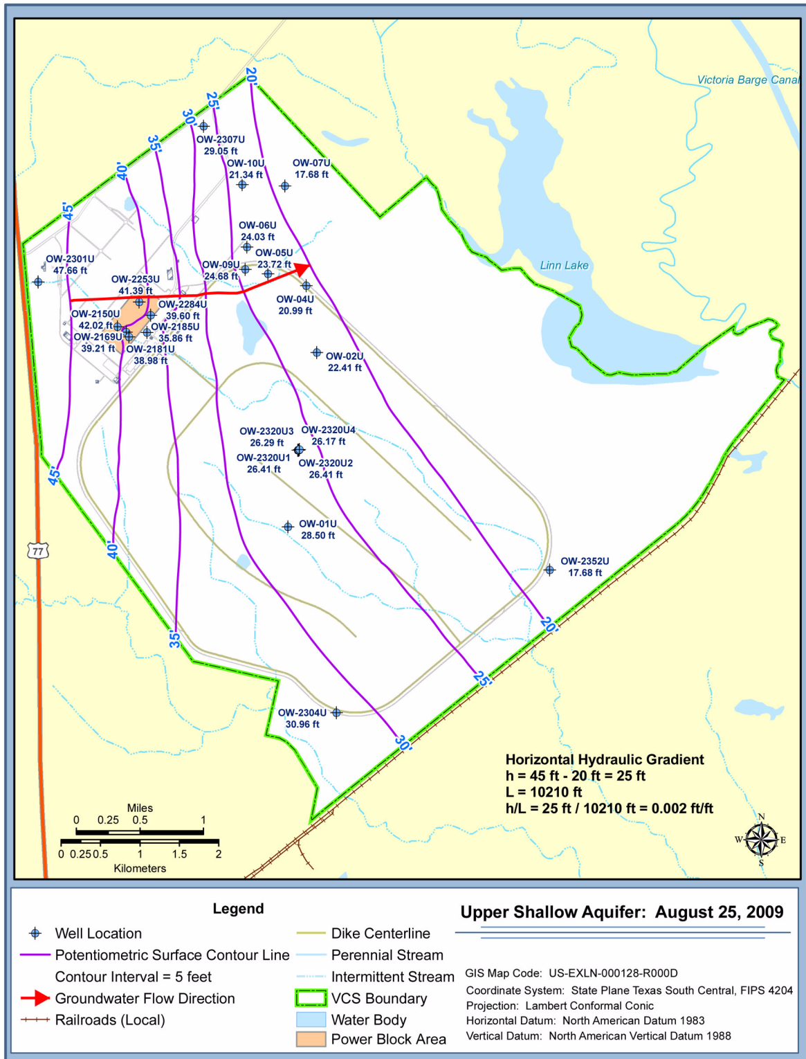
Figure 2.4.12-15 Potentiometric Surface Maps (Sheet 19 of 21)
