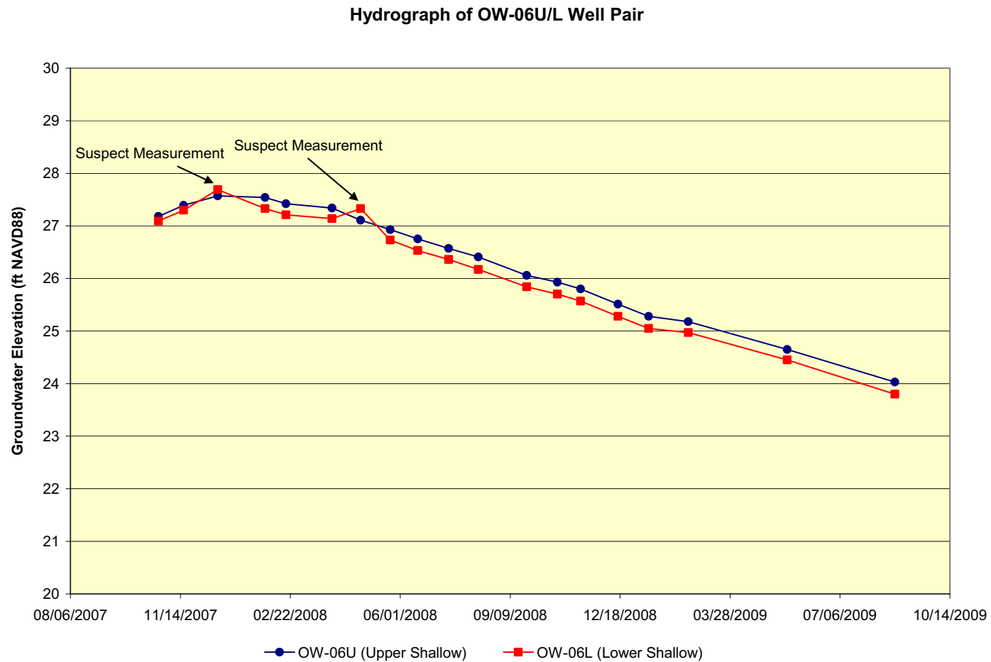
Figure 2.4.12-17 VCS Site Hydrographs; OW-06U/L Well Pair (Sheet 6 of 28)
