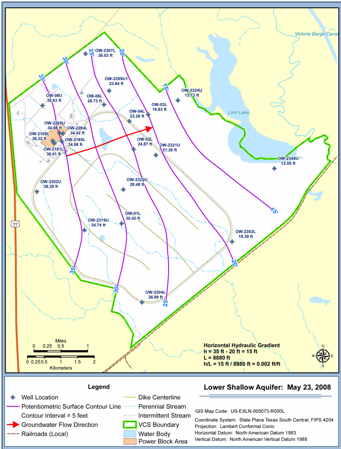
Figure 2.4.12-15 Potentiometric Surface Maps (Sheet 5 of 21)
