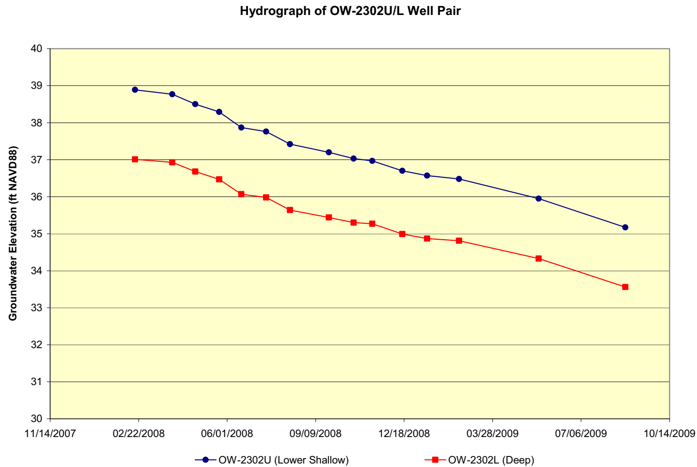
Figure 2.4.12-17 VCS Site Hydrographs; OW-2302U/L Well Pair (Sheet 19 of 28)
