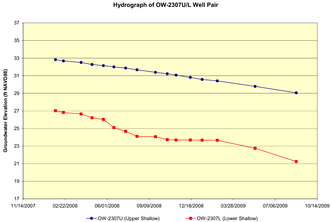
Figure 2.4.12-17 VCS Site Hydrographs; OW-2307U/L Well Pair (Sheet 21 of 28)
