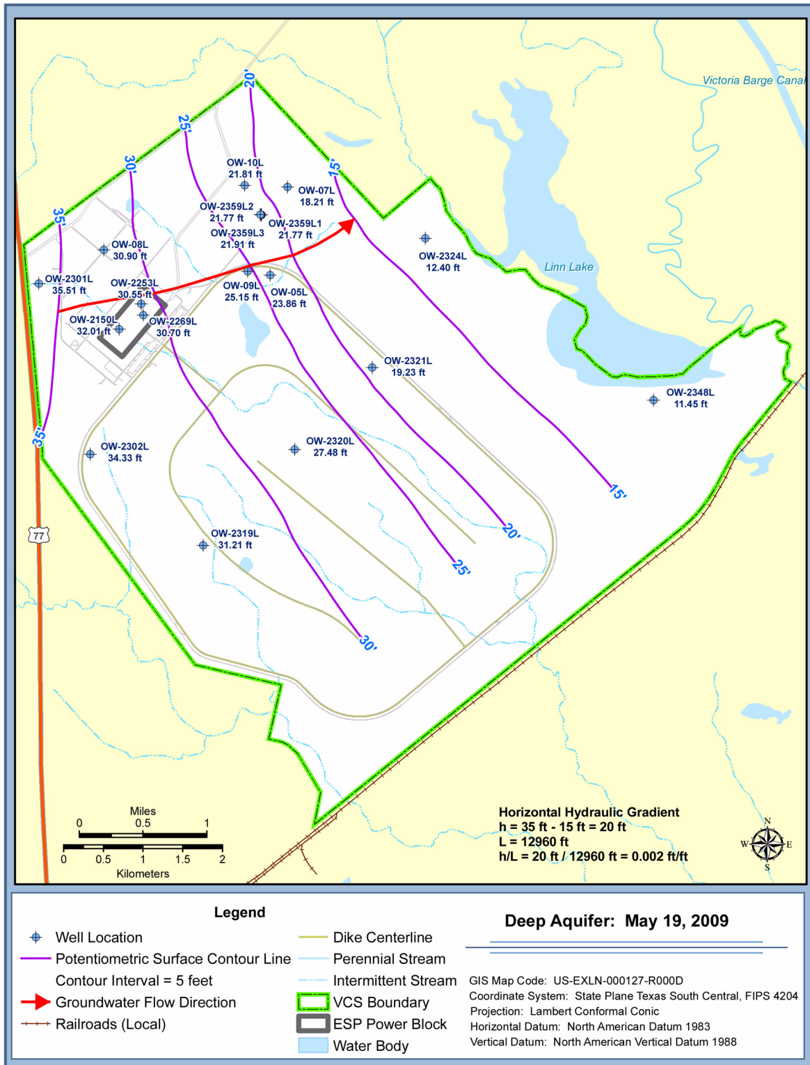
Figure 2.4.12-15 Potentiometric Surface Maps (Sheet 18 of 21)
