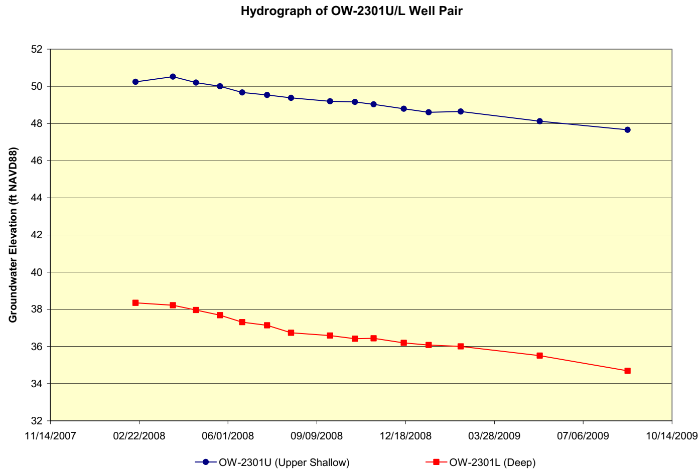
Figure 2.4.12-17 VCS Site Hydrographs; OW-2301U/L Well Pair (Sheet 18 of 28)
