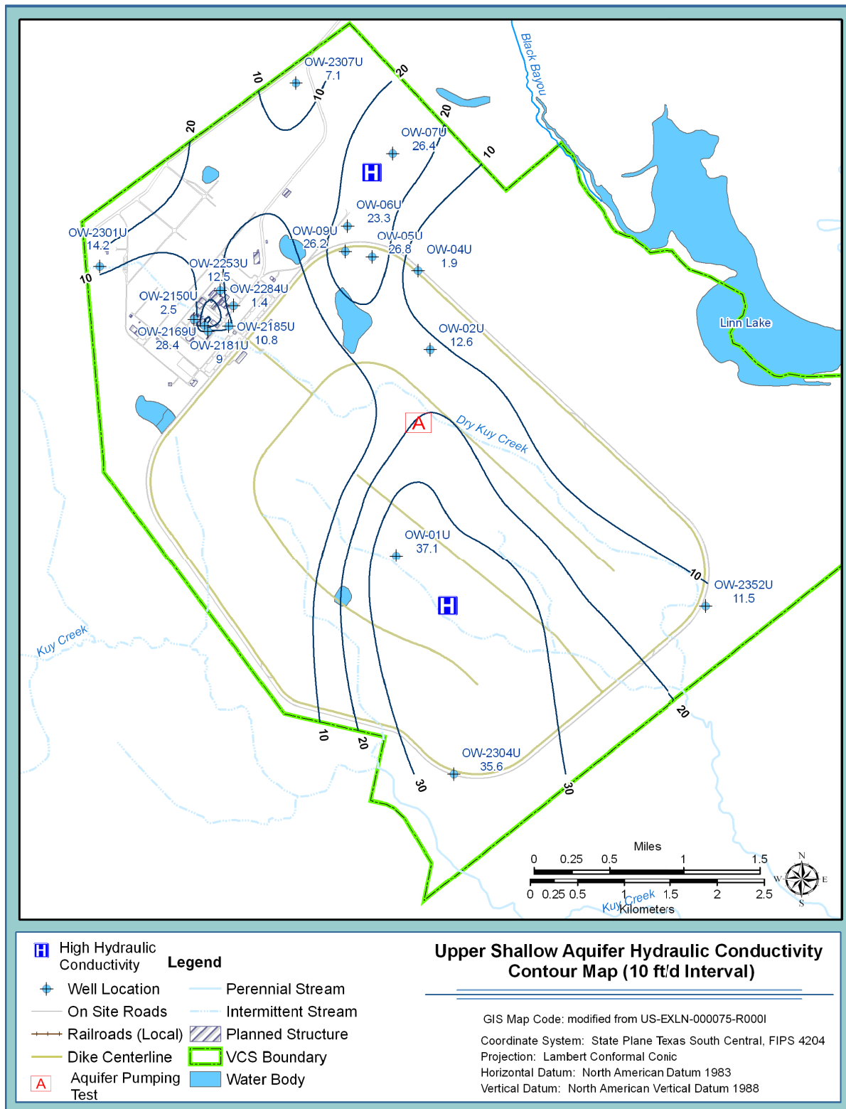
Figure 2.4.12-18 Contour Maps of Hydraulic Conductivity from Slug Tests (Sheet 1 of 3)
