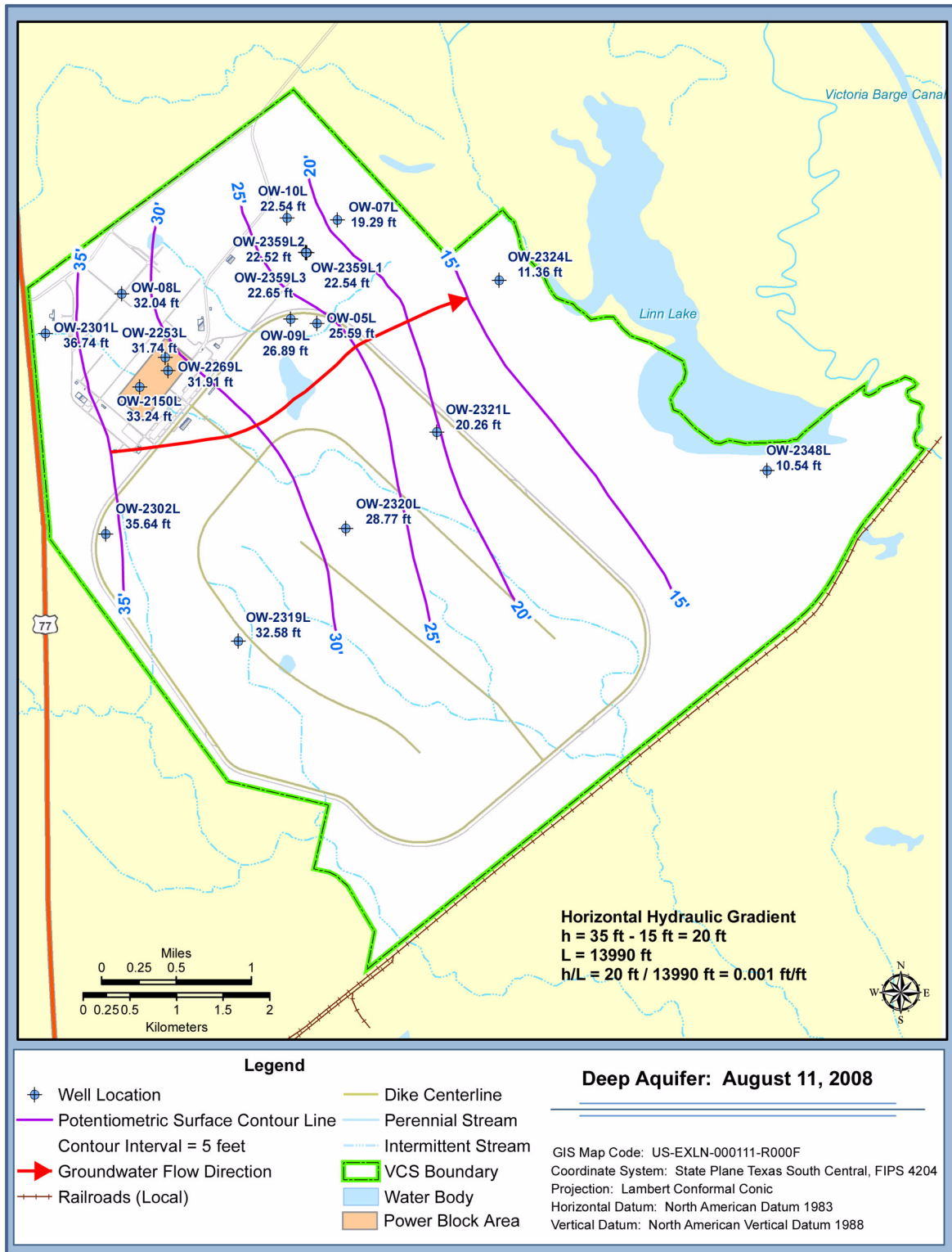
Figure 2.4.12-15 Potentiometric Surface Maps (Sheet 9 of 21)
