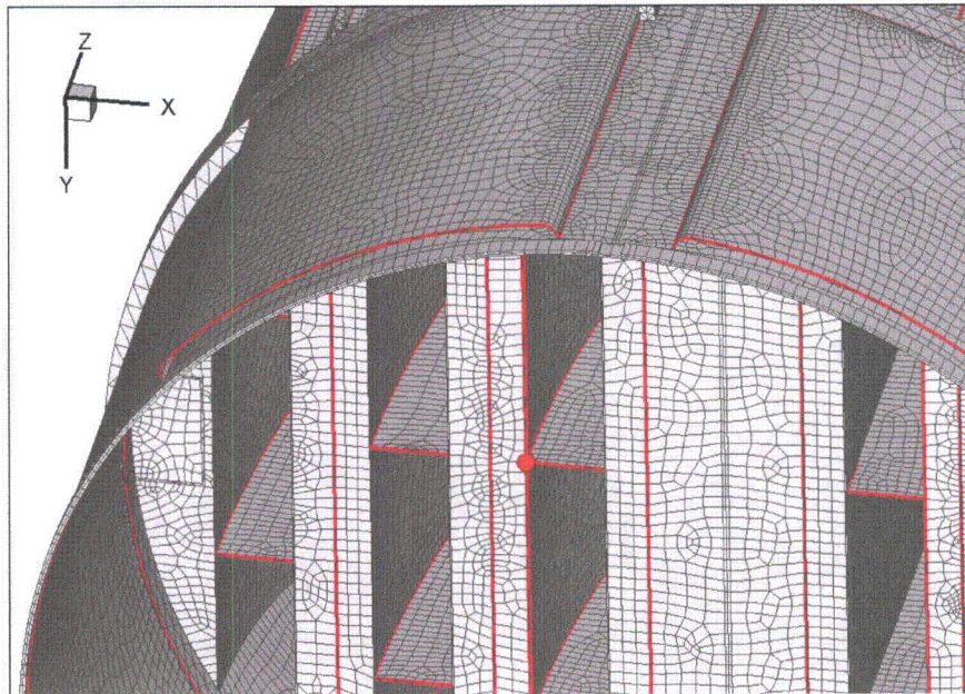
Figure 11c. Location of node on hood/hood support/base plate weld analyzed with sub-model in [18]. Sub-model corresponds to location 6 in Table 7.
