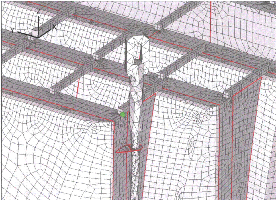
Figure 11e. Location of node on side plate/top plate weld analyzed with sub-model analysis procedure in [22]. Sub-model corresponds to location 8 in Table 7.
