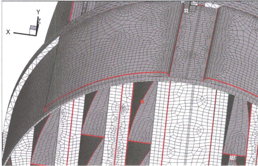
Figure 11d. Location of node on hood/hood support weld analyzed with sub-model analysis procedure in [19]. Sub-model corresponds to location 7 in Table 7.
