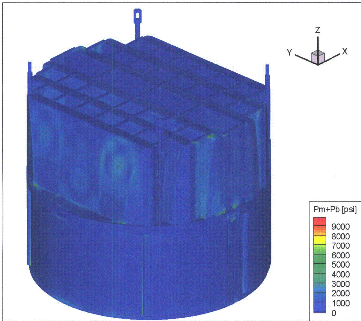
Figure 13b. Contour plot of maximum membrane+bending stress intensity, P_m+P_b , for CLTP operation with frequency shifts. The recorded stress at a node is the maximum value taken over all frequency shifts. The maximum stress intensity is 9809 psi. First view.
