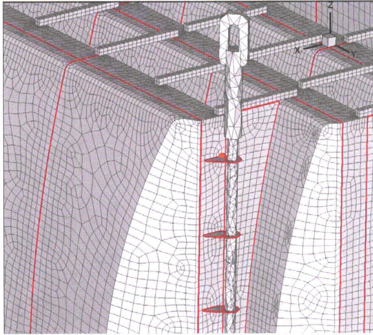
Figure 11b. Location of node on inner hood/hood support/middle base plate weld analyzed with sub-model in [22]. Sub-model corresponds to location 5 in Table 7.
