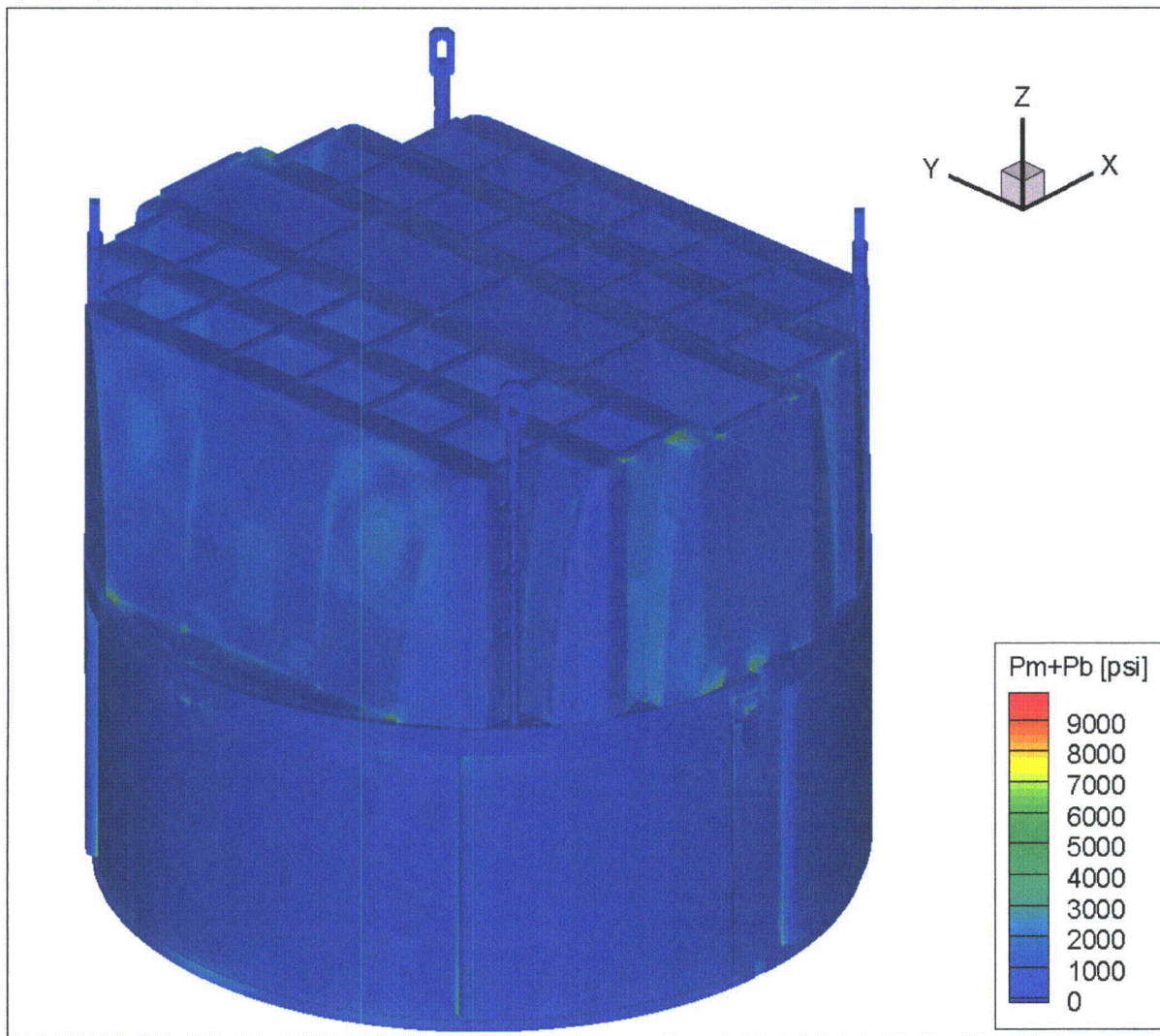
Figure 12b. Contour plot of maximum membrane+bending stress intensity, P_m+P_b , for CLTP load. The maximum stress intensity is 9809 psi. First view.
