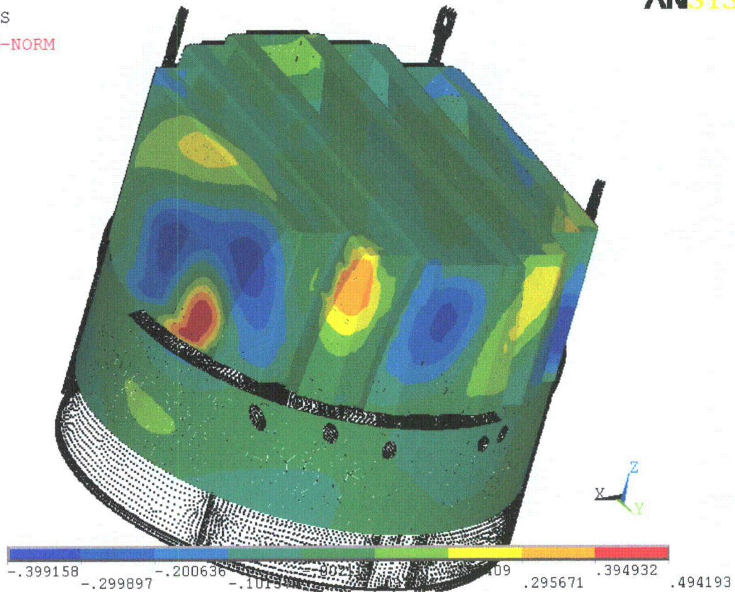
Figure 8b. Real part of unit pressure loading MSL A (in psid) on the steam dryer at 200.45 Hz. No loading is applied to the submerged surface and lifting rods.
