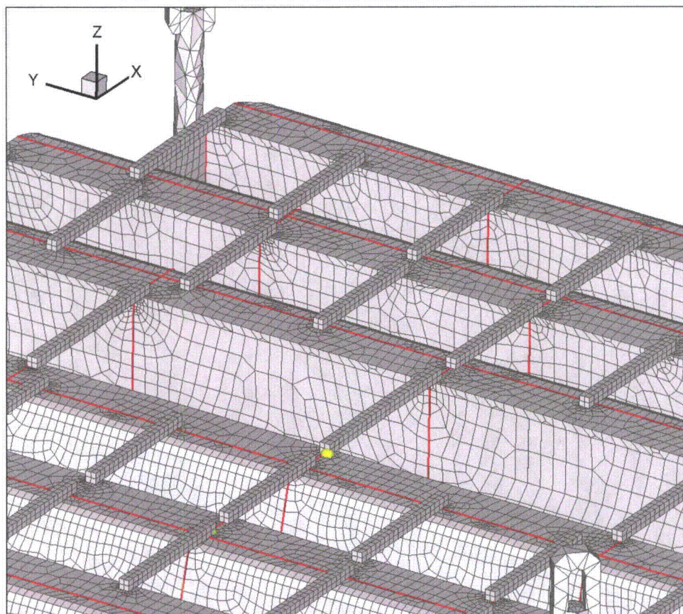
Figure 11f. Location of node on tie bar/top vane bank plate weld analyzed with sub-model analysis procedure in [22]. Sub-model corresponds to location 9 in Table 7.
