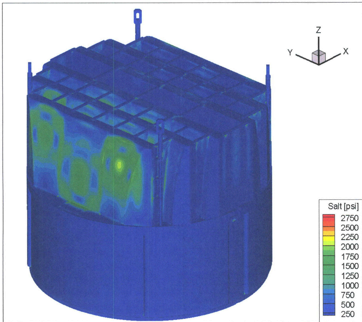
Figure 12d. Contour plot of alternating stress intensity, S_{alt} , for CLTP load. The maximum alternating stress intensity is 2728 psi. First view.
