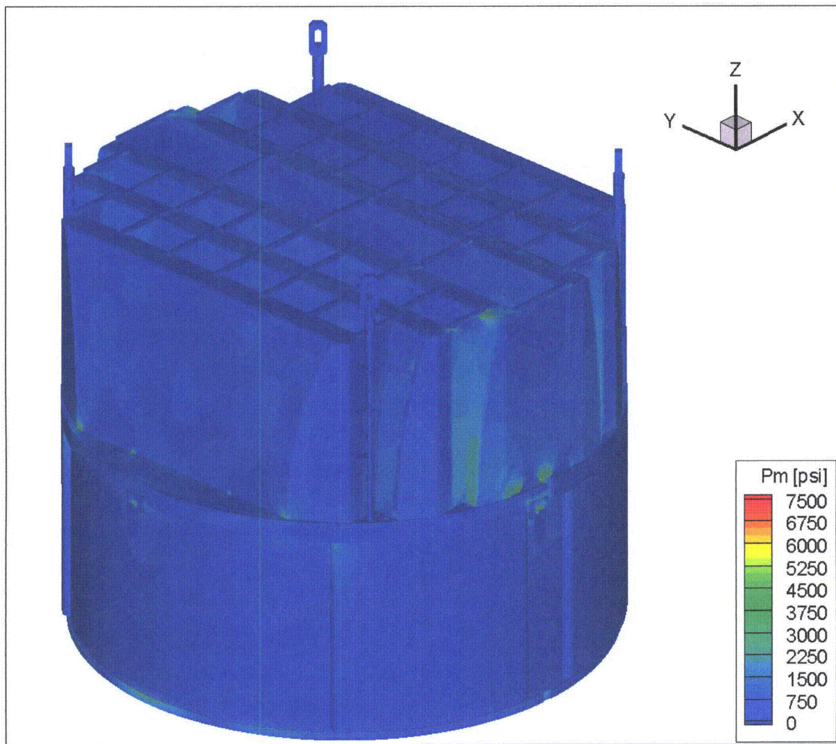
Figure 12a. Contour plot of maximum membrane stress intensity, P_m , for CLTP load. The maximum stress intensity is 7475 psi.
