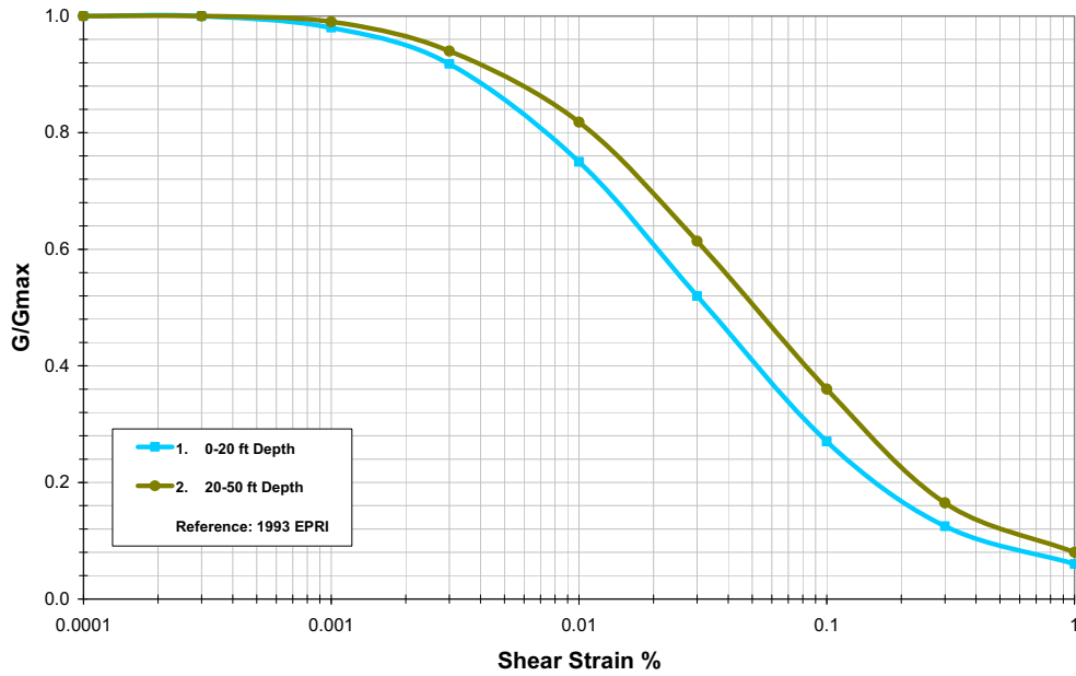
Figure 1a: G/G_{max} vs. Strain (Sand Characteristic Behaviour, EPRI 1993)
