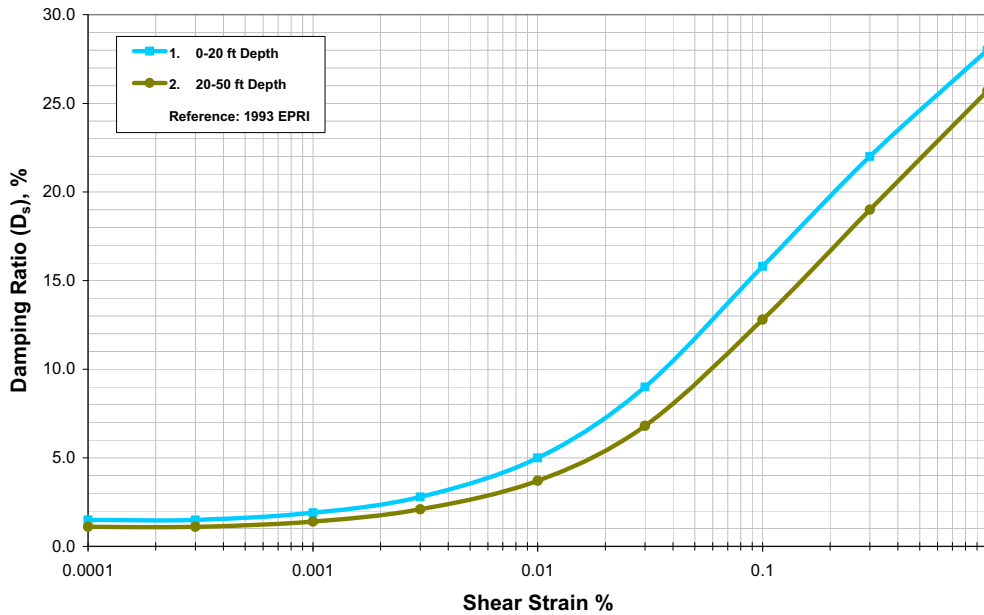
Figure 1b: Damping in Shear vs. Strain (Sand Characteristic Behaviour, EPRI 1993)
