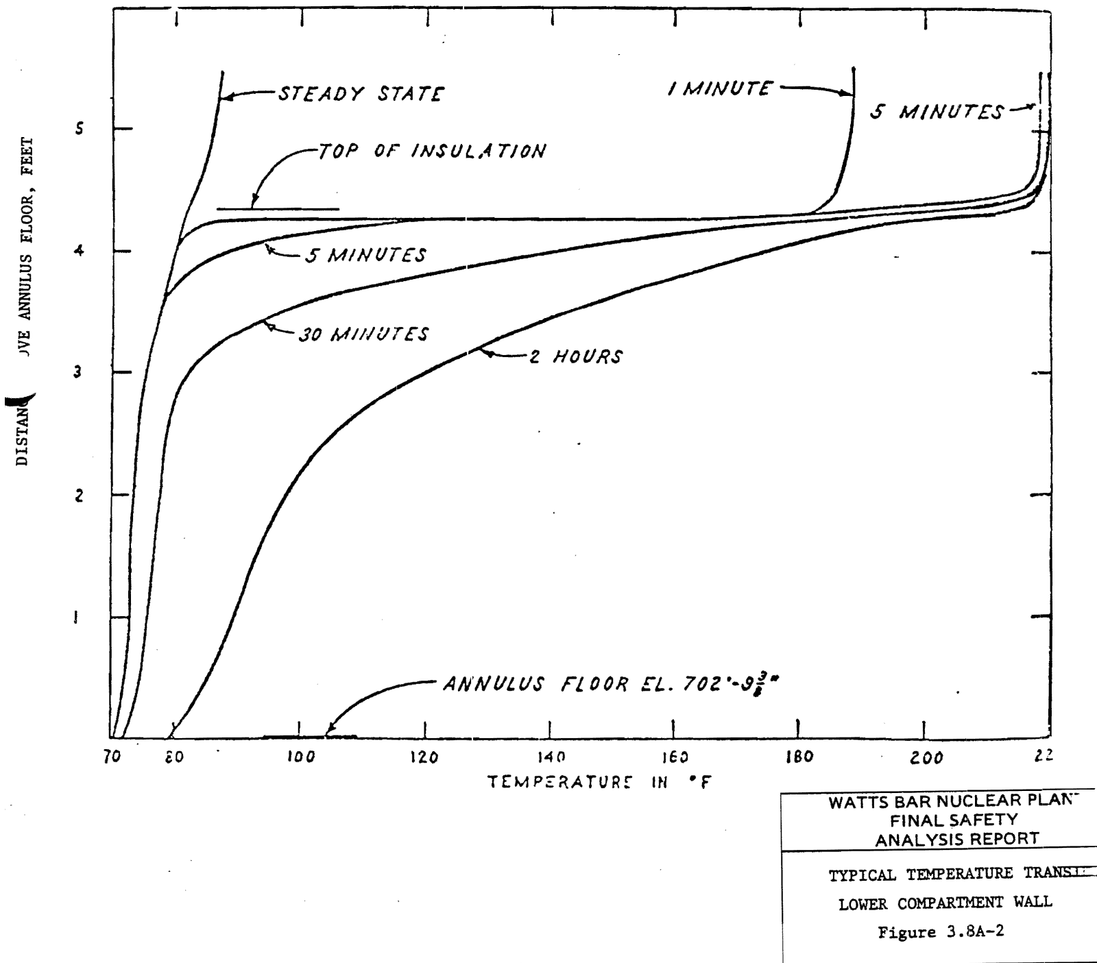
Figure 3.8A-2 Typical Temperature Transient Lower Compartment Wall
