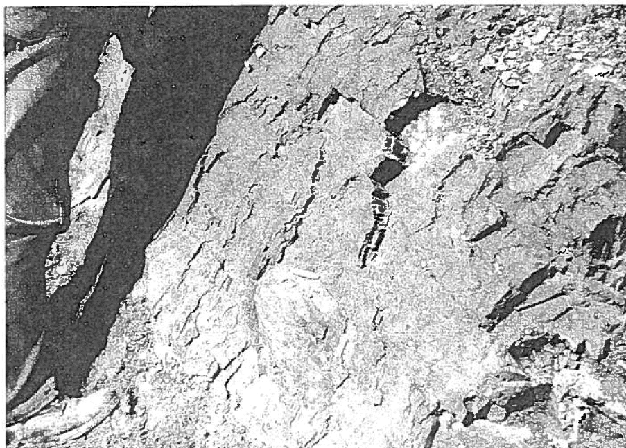
Figure 8-9. Polymictic diamictite in the lower part of the Rockwell Formation, exposed along the westbound lane of Interstate Route 70 in Bedford County, just west of the Bedford-Fulton County line. Note the abundant small pebbles in the mudstone matrix and the large clast (27 by 12 cm [11 by 5 in.]) just below the penknife. Photograph by J. A. Harper.
