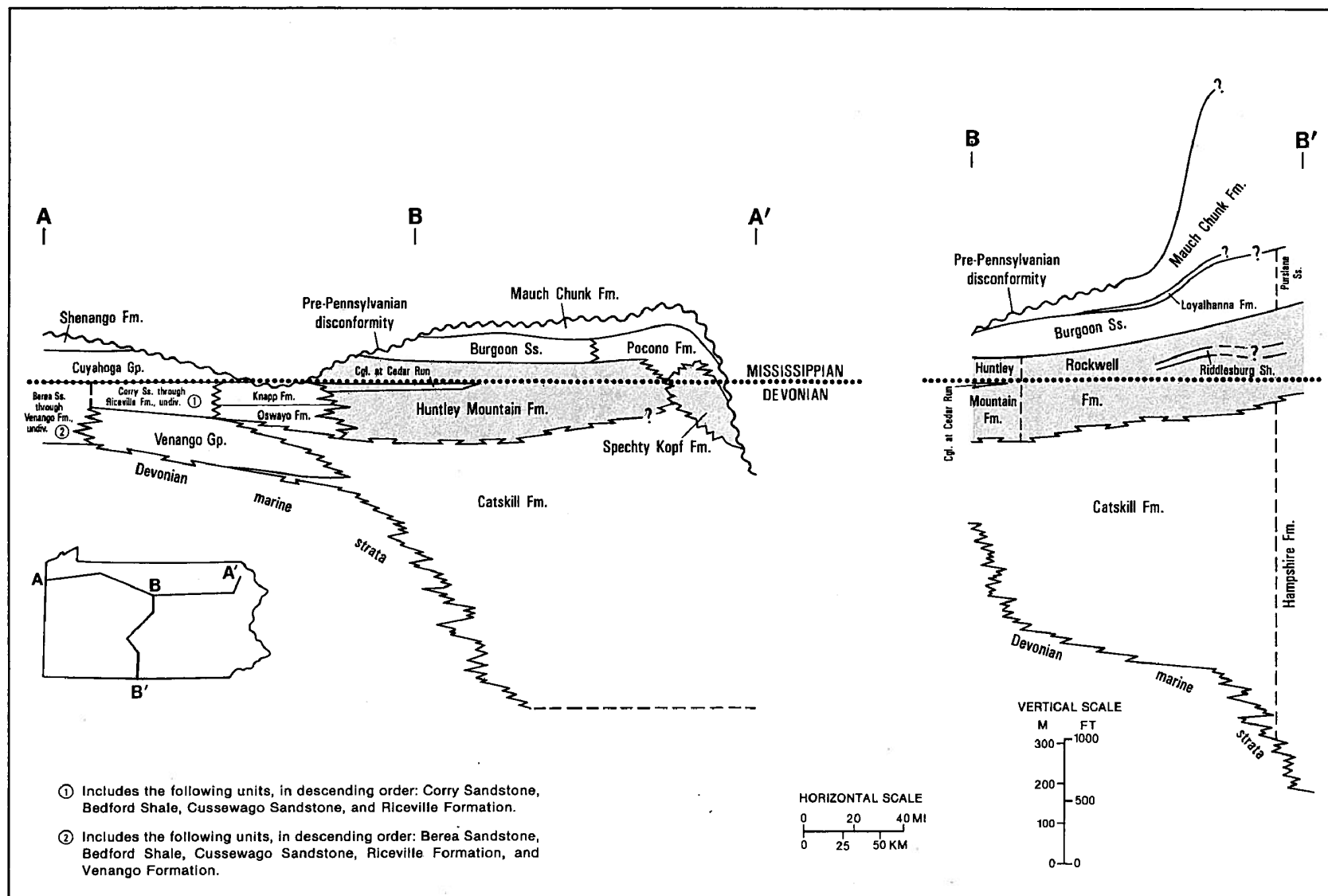
Figure 8-1. Lithostratigraphic cross sections showing the relationships among the Devonian-Mississippian transition formations (colored), overlying and underlying formations, and Mississippian and Upper Devonian marine units of northwestern Pennsylvania.
