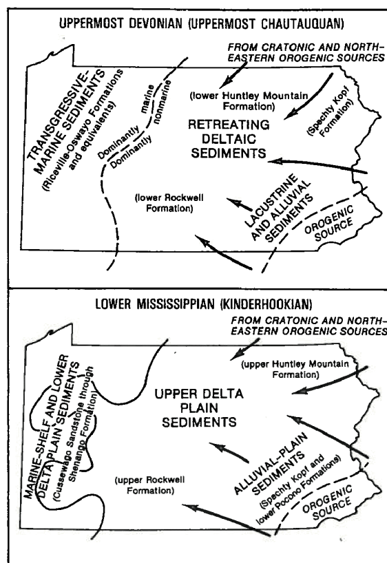
Figure 8-3. Paleogeographic maps showing generalized sedimentary environments during deposition of Devonian-Mississippian transition formations.
