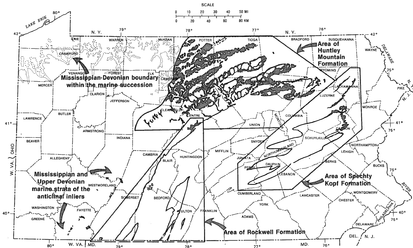
Figure 8-2. Areas in Pennsylvania where the Spechty Kopf, Huntley Mountain, and Rockwell Formations have been mapped (modified from Berg and others, 1980). The position of the boundary between Mississippian and Devonian strata of northwestern Pennsylvania is shown by the dotted line.
