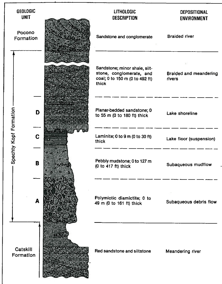
Figure 8-4. Generalized stratigraphic column showing the character of the Spechty Kopf Formation and inferred depositional environments. The colored arrow marks a fining-upward cycle in the Catskill Formation.
