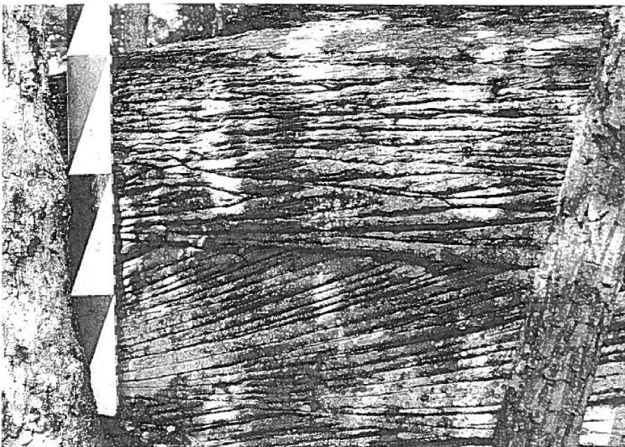
Figure 8-6. Outcrop of crossbedded sandstone in the lower part of the Huntley Mountain Formation at the type section in Lycoming County, near Waterville. The scale is marked in feet.
