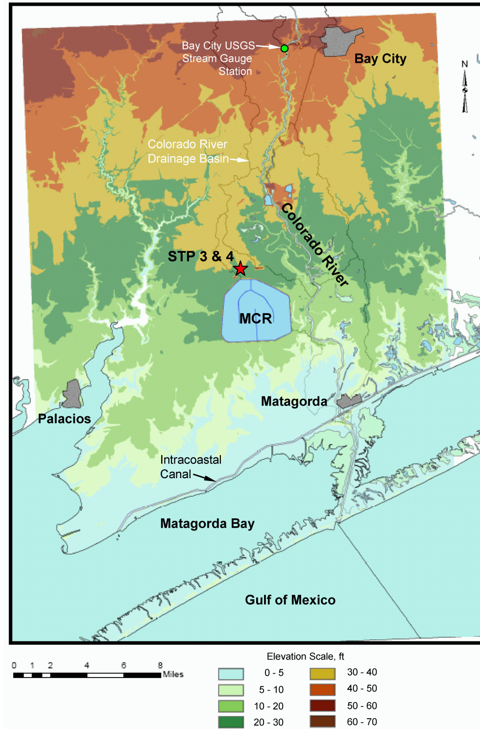
Figure 2.3.1-1 Site Map of STP 3 &amp; 4
