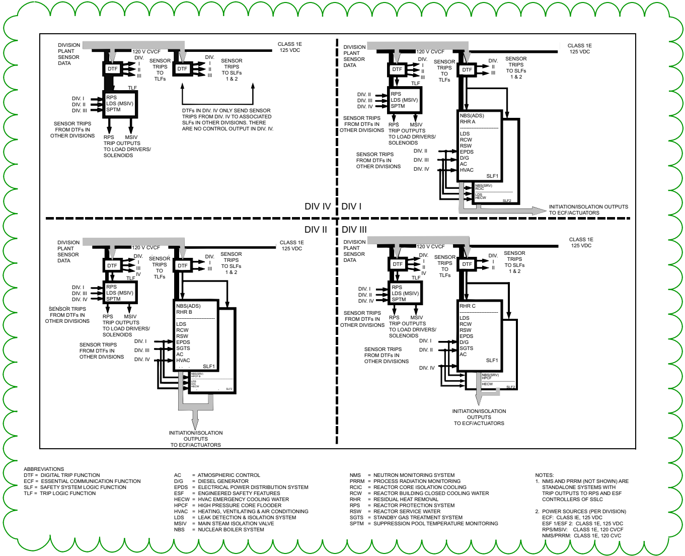
Figure 7.1-2 Assignment of Interfacing Safety System Logic to SSLC Controllers
