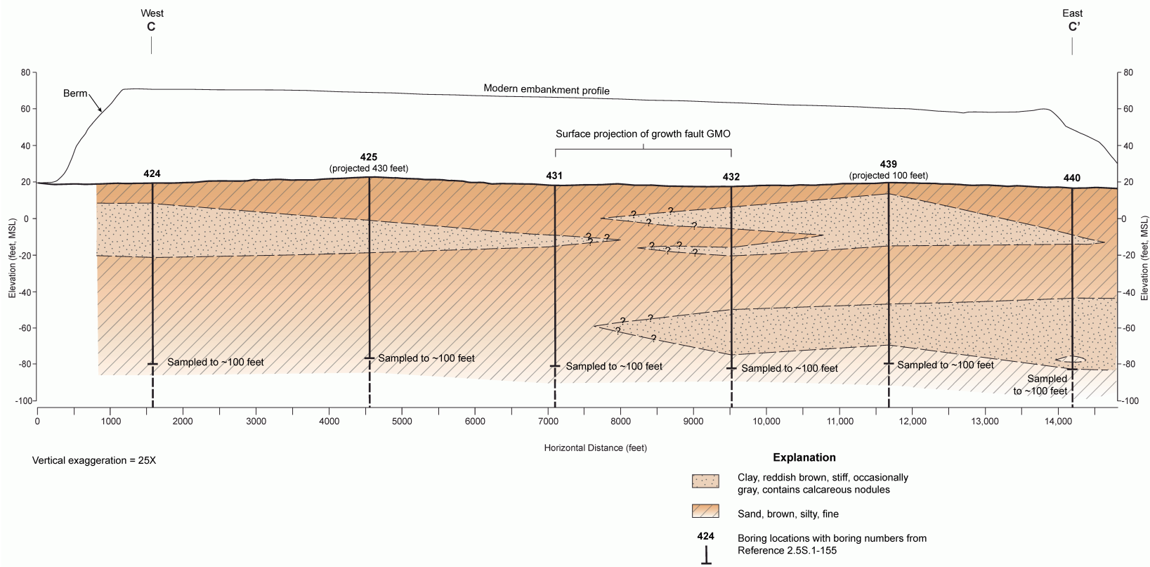
Figure 2.5S.1-47 Cross Section C-C' Along Southern Embankment of Cooling Reservior
