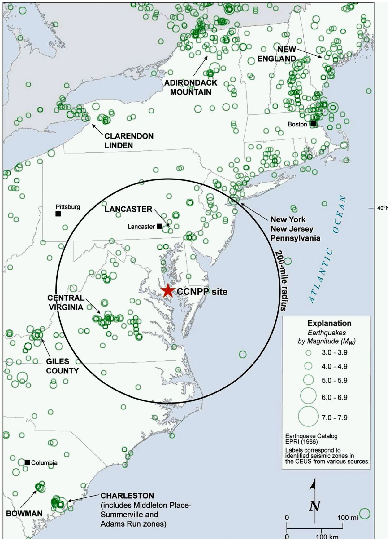
Figure 2.5-52—{Seismic Zones and Seismicity in CEUS}
