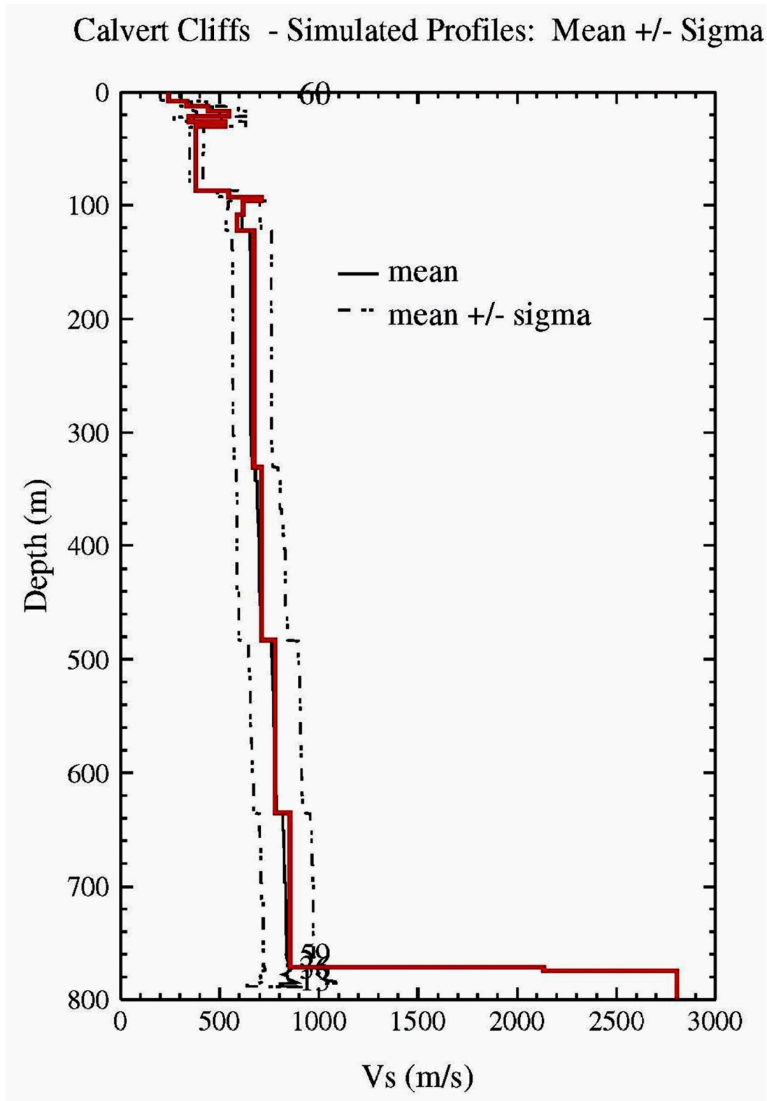
Figure 2.5-75—{Median (Mean of Logarithmic Values) \pm Standard Deviation ( \sigma of Log Values) of Shear Wave Velocity ( V_s ) vs Depth for All 60 Profiles (Thin Solid and Dashed Lines, Compared to Median V_s Profile (red))}
