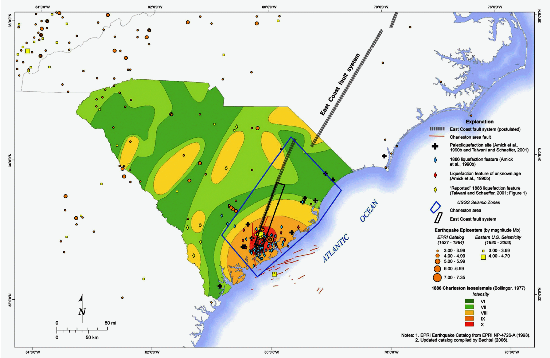
Figure 2.5-53—{USGS Model}
